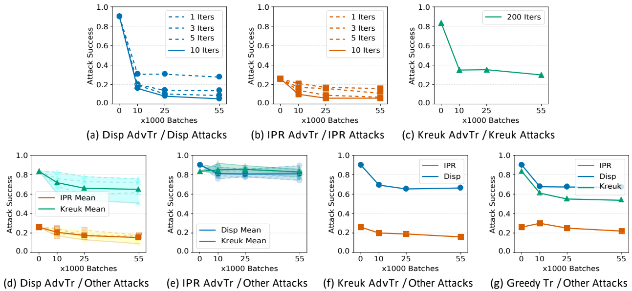
Figure 3: Comparing attack success rates for Disp, IPR, and Kreuk attacks up to 200 iterations between models trained with varying number of adversarial examples and training attack iterations. Training on these attacks substantially increases model robustness to the same attack, as shown in Figs. 3a–3c. The downward trends in Fig. 3d and Fig. 3f show that training on Disp or Kreuk attacks reduces model vulnerability to other attacks by a smaller amount. “{IPR, Disp, Kreuk} Mean” is the mean attack success rate over multiple adversarially trained models (e.g., 1-, 3-, 5-, 10-iteration Disp-adversarially-trained models in Fig. 3d).
