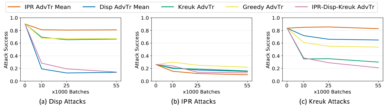
Figure 4: Attack success rates for Disp, IPR, and Kreuk attacks up to 200 iterations against different types of adversarial training. IPR-Disp-Kreuk training represents a model trained with a combination of IPR (up to 5 iterations), Disp (up to 5 iterations), and Kreuk attacks. Training with all three of these attacks induces near best-case robustness benefit to all attacks simultaneously.
