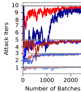
Figure 7: Number of attack iterations (smoothed over 100 batches) executed in different adversarial training runs. Red, blue lines represent IPR, Disp attacks, resp. Attacks quickly take up to their allowed iter cap, slowing adv training.
