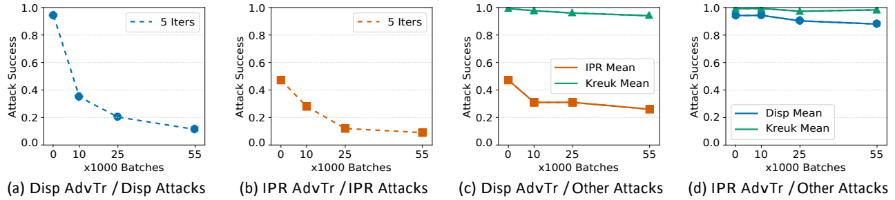
Figure 5: Plots show results for AvastNet. Comparing attack success rates for Disp, IPR, and Kreuk attacks up to 200 iterations between AvastNet models trained with varying number of adversarial examples and training attack iterations. Training on either IPR or Disp attacks substantially increases model robustness to the same attack, as shown in Figs. 5a–5b. The downward trends in Fig. 5c show that training on Disp attacks reduces model vulnerability to other attacks by a smaller amount.
