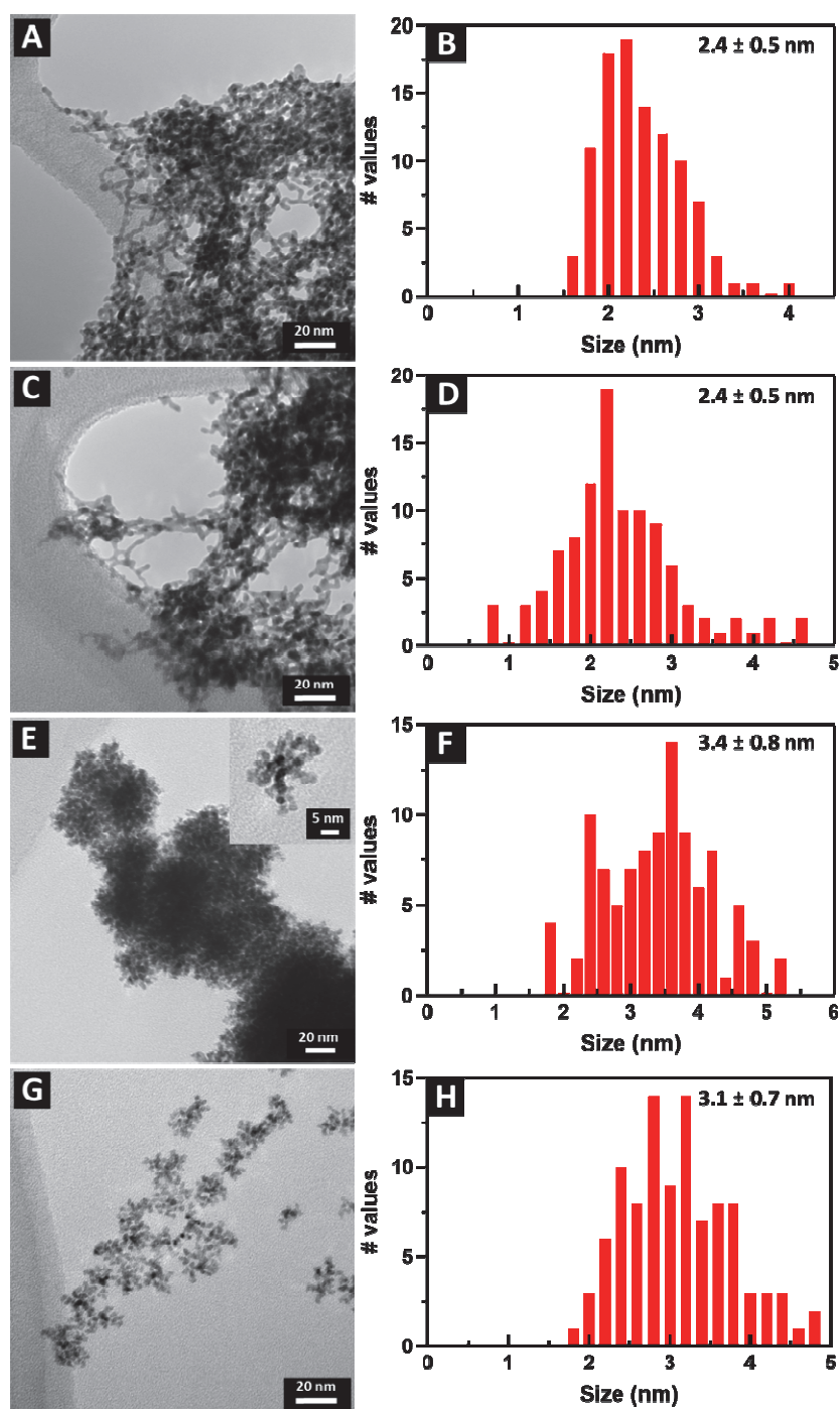
Figure 1. TEM images and size distributions are shown of a range of chemically distinctive ultrathin NWs, prepared by different synthesis methods. (A, B) Pt 1 Ru 1 and (C, D) Pt 1 Ru 1 were both prepared with CTAB. (E, F) Pt 1 Ru 1 with the inset showing an individual cluster as well as (G, H) Pt 1 Ru 9 were generated with OAm and OA.
