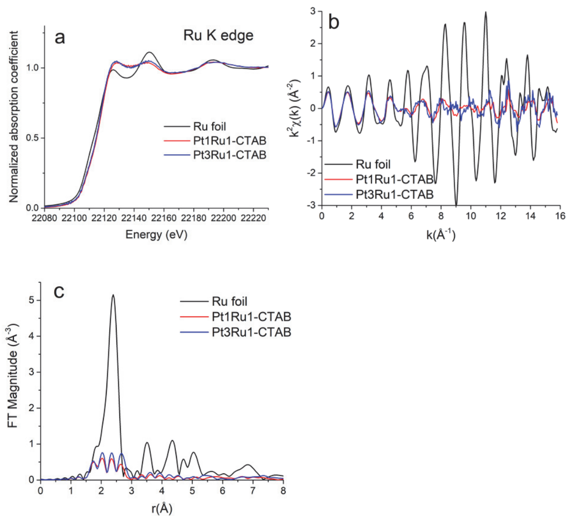
Figure 5. (A) Ru K-edge XANES data. (B) k^2 -weighted EXAFS data in k -space. (C) Fourier transform magnitudes of the k^2 -weighted EXAFS data for Ru foil, Pt 1 Ru 1 (produced with CTAB), and Pt 3 Ru 1 (generated with CTAB).
