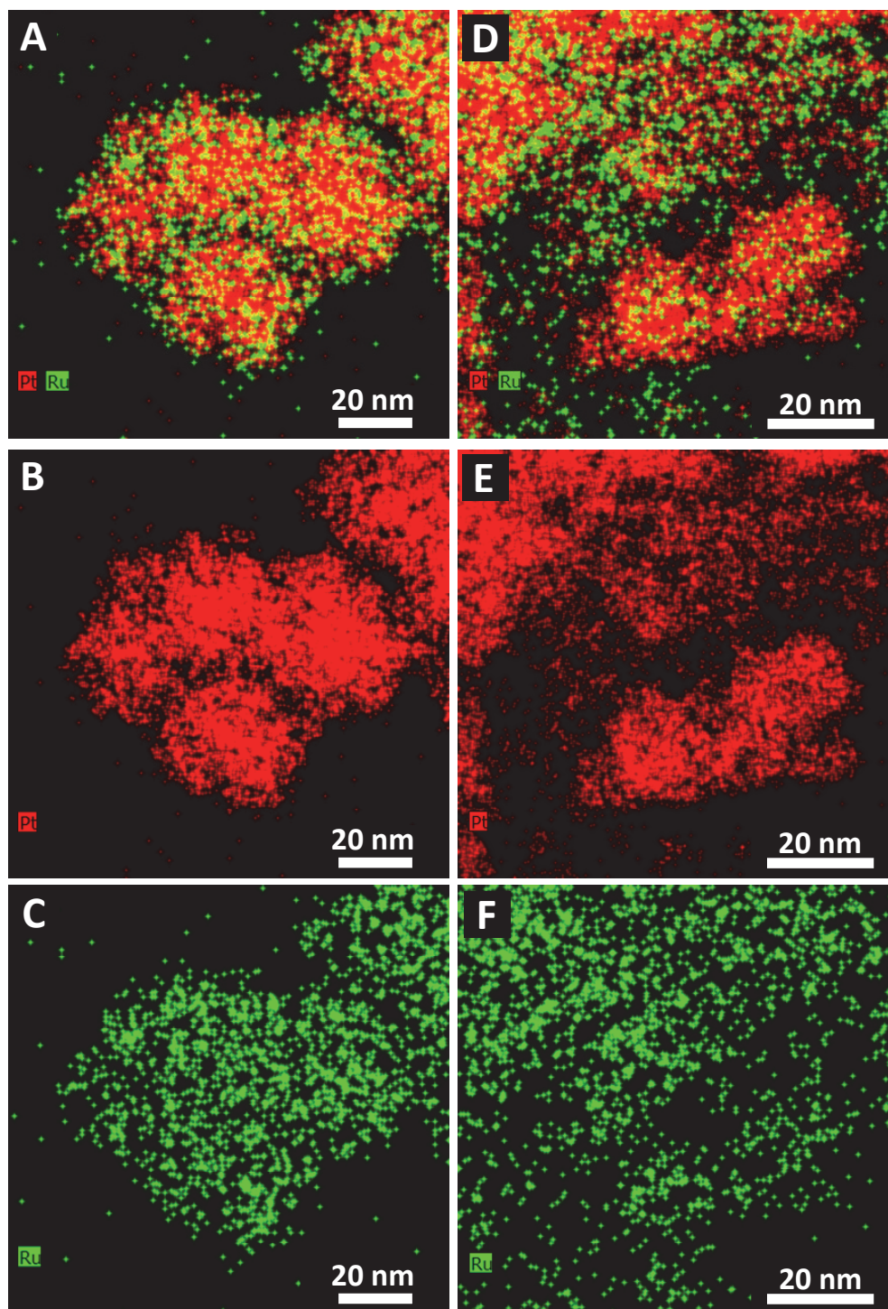
Figure 3. EDS elemental maps of PtRu prepared using the OAm/OA method. Pt 1 Ru 1 maps are given as (A) the composite of Pt and Ru, (B) Pt, and (C) Ru. Corresponding Pt 1 Ru 9 elemental maps are shown in (D) the composite of Pt and Ru, (E) Pt, and (F) Ru.
