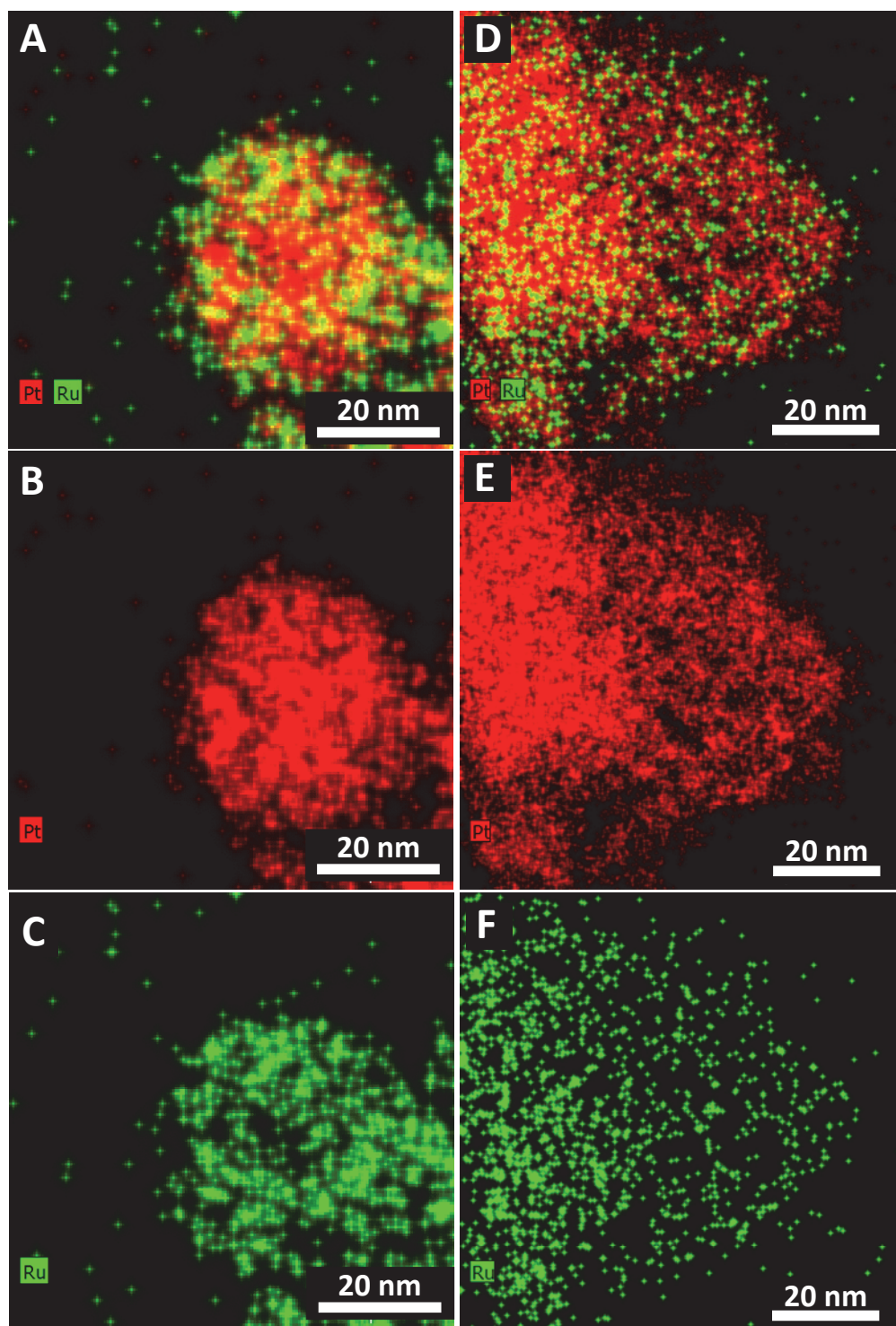
Figure 2. EDS elemental maps of PtRu generated using the CTAB method. Pt 1 Ru 1 maps are provided as follows: (A) composite of Pt and Ru, (B) Pt, and (C) Ru. Analogous Pt 3 Ru 1 maps are shown, as (D) composite of Pt and Ru, (E) Pt, and (F) Ru.
