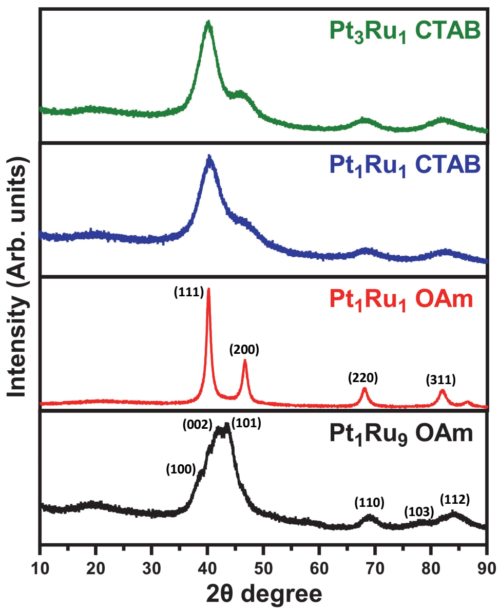
Figure 7. XRD data for all of the alloyed samples generated.
