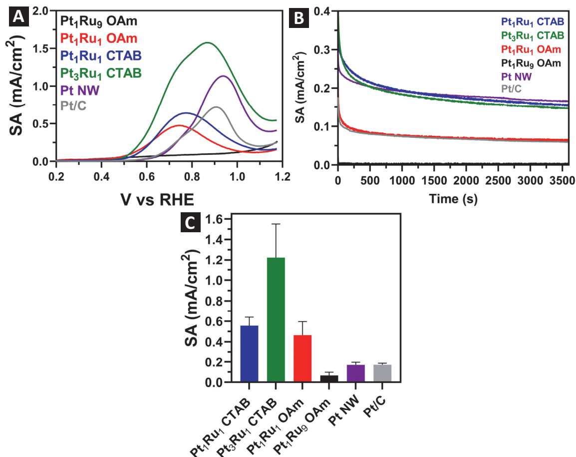
Figure 8. MOR results for all PtRu alloyed ultrathin wires as well as particulate clusters, in addition to the Pt nanowire and Pt/C commercial control samples, with their corresponding synthesis methods and surfactants. Data shown herein include (A) MOR LSVs, (B) chronoamperometry plots, and (C) bar graphs of the specific activity measurements of the various nanoscale motifs.
