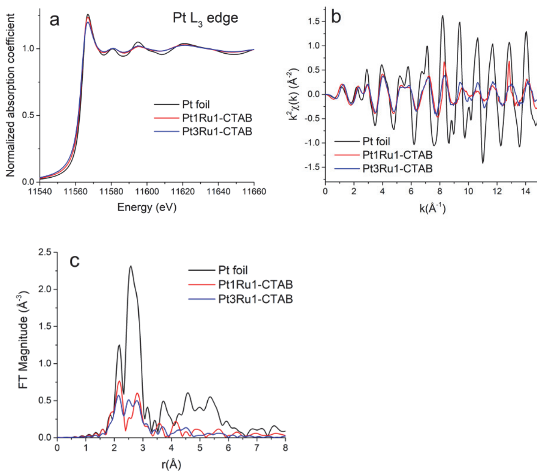
Figure 4. (A) Pt L 3 -edge XANES data. (B) k 2 -weighted EXAFS data in k-space. (C) Fourier transform magnitudes of the k 2 -weighted EXAFS data for Pt foil, Pt 1 Ru 1 (produced with CTAB), and Pt 3 Ru 1 (produced with CTAB).
