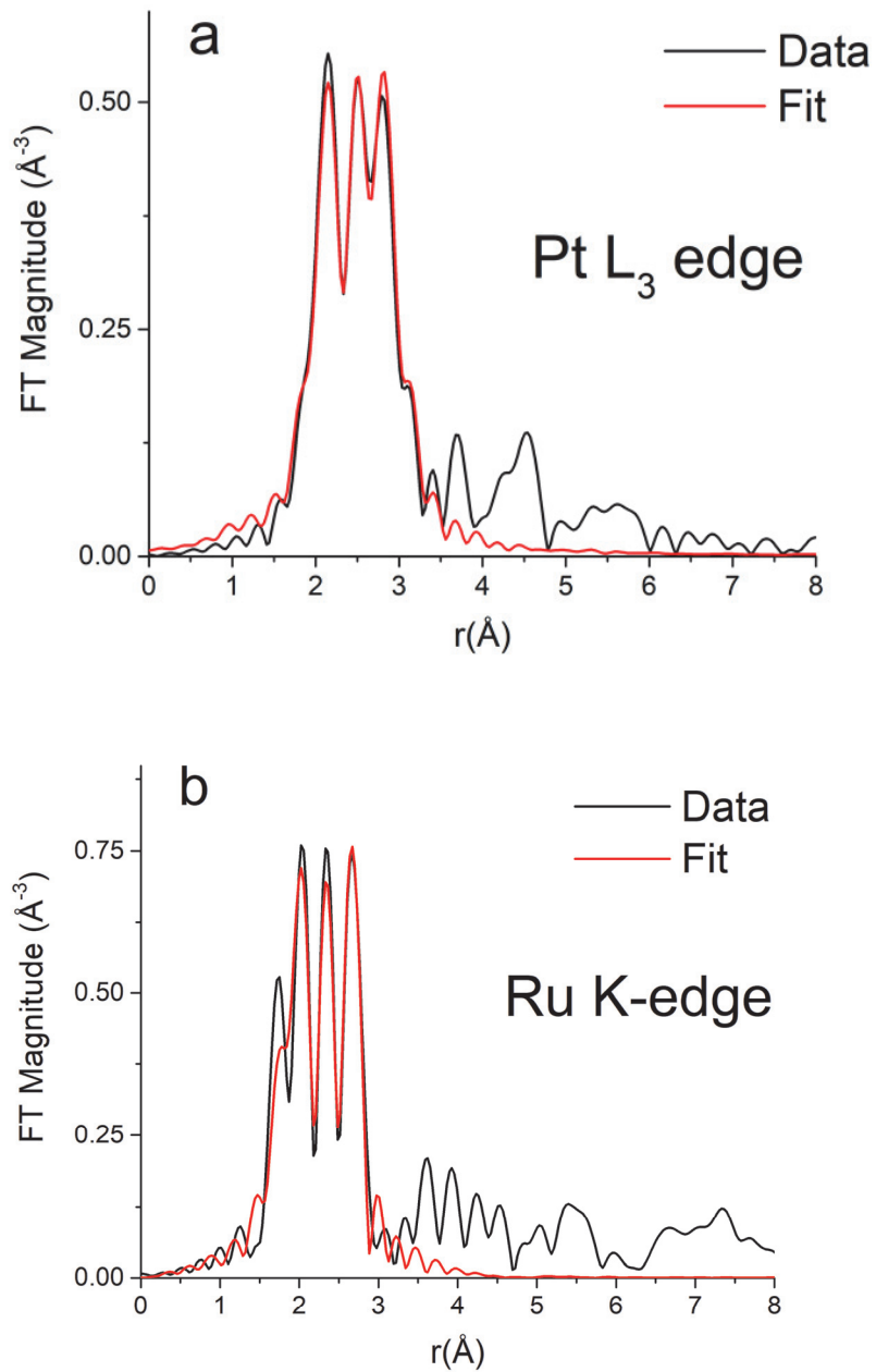
Figure 6. Fourier transform magnitudes of k^2 -weighted EXAFS data and theoretical fits for the \text{Pt}_3\text{Ru}_1 (generated with CTAB) sample at (A) the Pt L_3 -edge and (B) the Ru K-edge.
