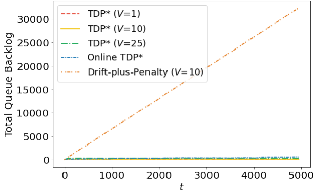
(a) All policies.
