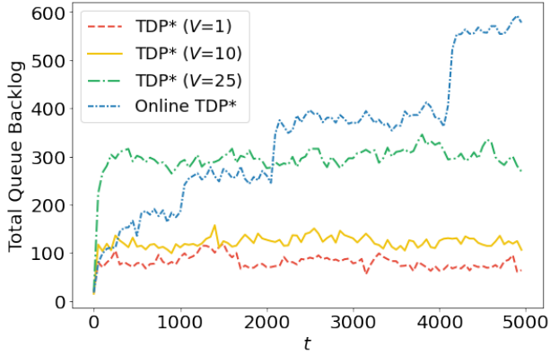
(b) Stabilizing policies.
