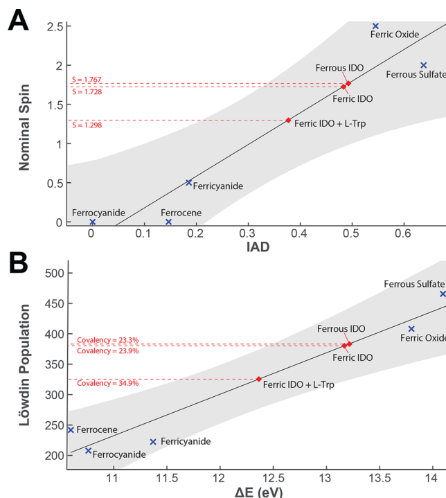
Figure 5. (A) IAD analysis based on a reference curve generated from a set of known spin state Fe standards (see Figure S1). Gray shading indicates 95% confidence interval of fit. (B) Similar covalency analysis based on a comparison of K\beta_{1,3} and K\beta' peak splitting and DFT orbital population calculations.
