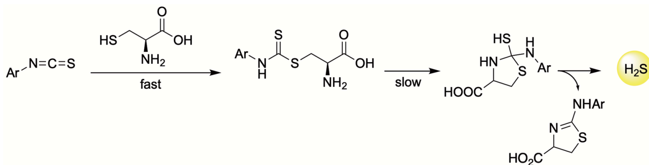
Figure 13. Thiol-triggered H 2 S release from isothiocyanates.
