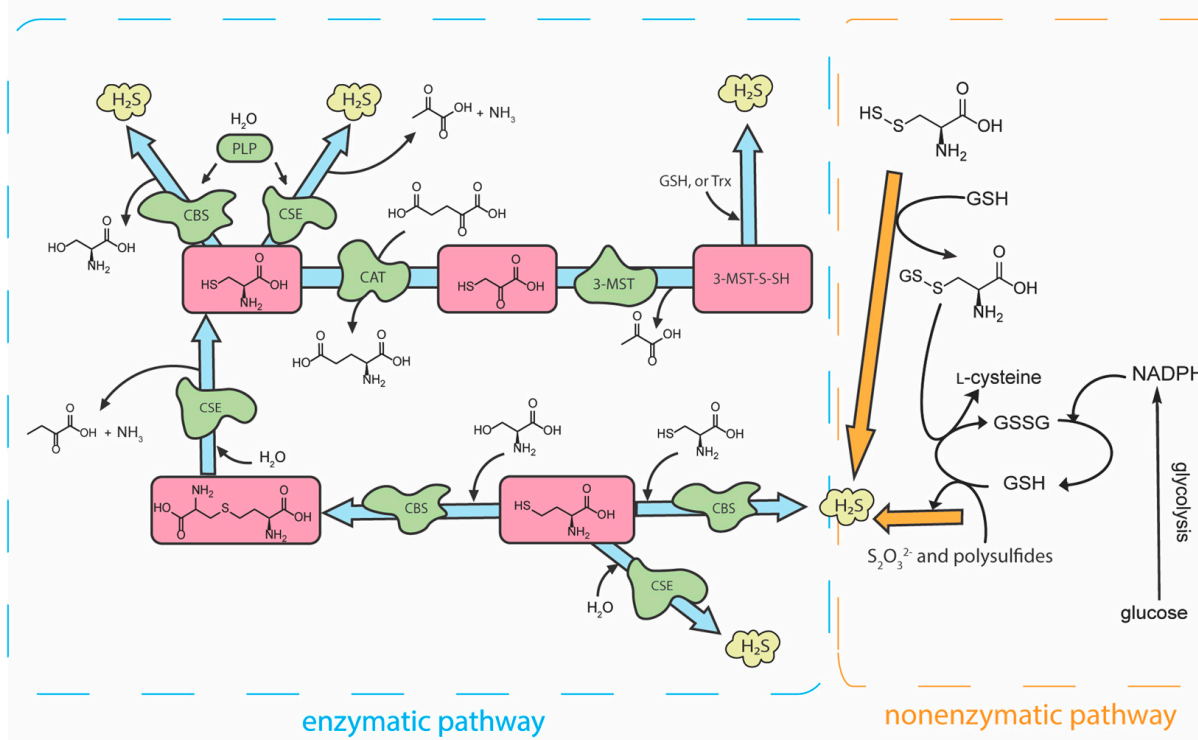
Figure 1. Enzymatic and nonenzymatic production of H 2 S in mammalian systems. PLP: pyridoxal 5'-phosphate; CBS: cystathionine \beta -synthase; CSE: cystathionine \gamma -lyase; CAT: cysteine aminotransferase; 3-MST: 3-mercaptopyruvate sulfurtransferase; NADPH: nicotinamide adenine dinucleotide phosphate.
