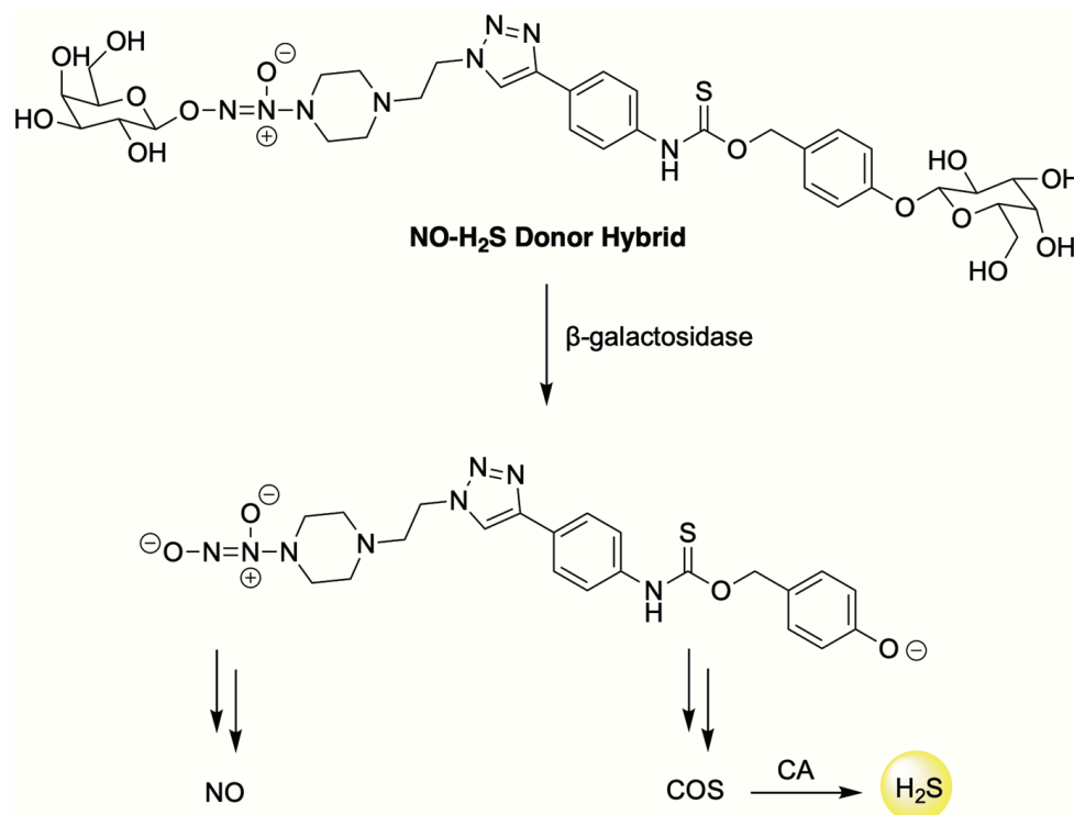
Figure 15. \beta -galactosidase-triggered \text{H}_2\text{S} release from an NO- \text{H}_2\text{S} donor hybrid, a compound with cardioprotective effects in MI/R injury models.
