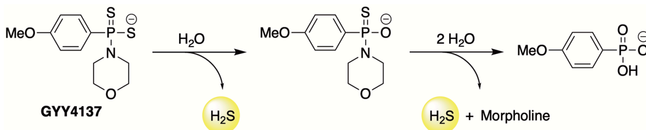
Figure 3. Hydrolysis-triggered \text{H}_2\text{S} release from GYY4137.
