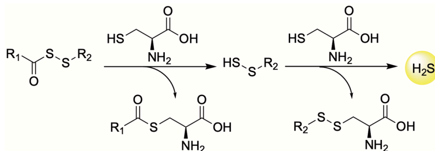
Figure 10. Thiol-triggered H 2 S release from acyl perthiols.
