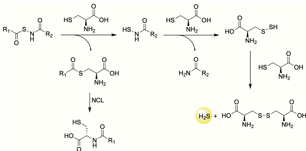
Figure 9. Thiol-triggered H 2 S release from NSHDs.
