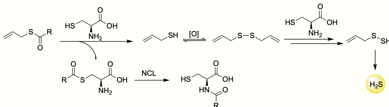
Figure 11. Thiol-triggered H 2 S release from allyl thioesters.
