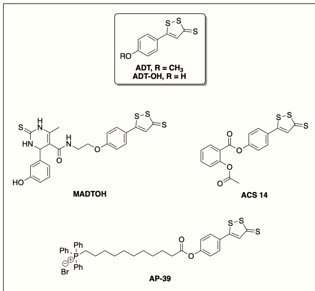
Figure 5. Chemical structures of DTIs and donor hybrids with protective effects against MI/R injury.
