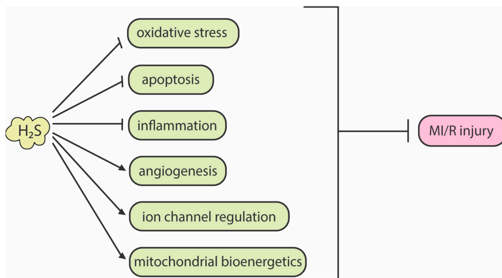
Figure 2. Molecular mechanisms that underscore the cardioprotective effects of \text{H}_2\text{S} , including its ability to combat MI/R injury.
