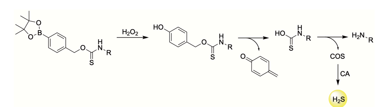
Figure 16. General mechanism for \text{H}_2\text{S} release from ROS-triggered, O-alkyl thiocarbamate-based donors.
