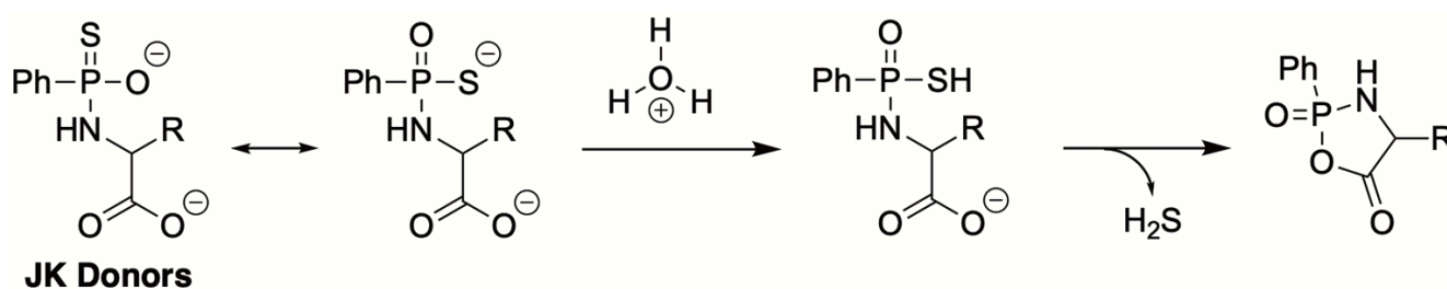
Figure 6. pH-triggered H 2 S release from JK donors.
