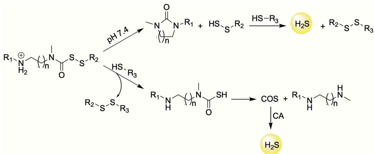
Figure 12. Thiol-triggered H 2 S release from perthiocarbamates.
