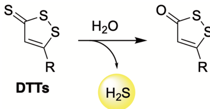
Figure 4. Hydrolysis-triggered \text{H}_2\text{S} release from DTTs.
