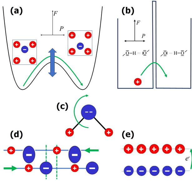
Figure 1. The green arrows indicate symmetry-restoring ferron excitations in selected ferroelectric materials. (a) sketches the soft-phonon excitation in the free energy landscape of a displacive ferroelectric with a temperature-dependent barrier (blue arrow). (b) In typical order-disorder ferroelectrics, the symmetry is restored by the hopping of protons in hydrogen bonds. (c) Thermally activated rotations destroy the order of permanent molecular dipoles. (d) The rigid relative shift of the bilayers reverses the electric polarization in a double well potential. (e) In electronic ferroelectrics, the symmetry is restored by the motion of electrons, not the ions.
