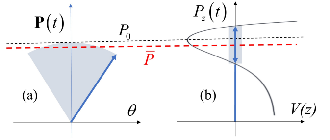
Figure 2. Sketch of an (a) “Goldstone” transverse and (b) “Higgs” longitudinal ferron mode. In (a) the modulus of the electric dipole P_0 is conserved during transverse oscillations, as in stable molecular dipoles. The projection on the equilibrium polarization |\bar{P}| < |P_0| . In (b) the length of the dipole fluctuates in an anharmonic potential V(z) that also reduces the average value |\bar{P}| < |P_0| .
