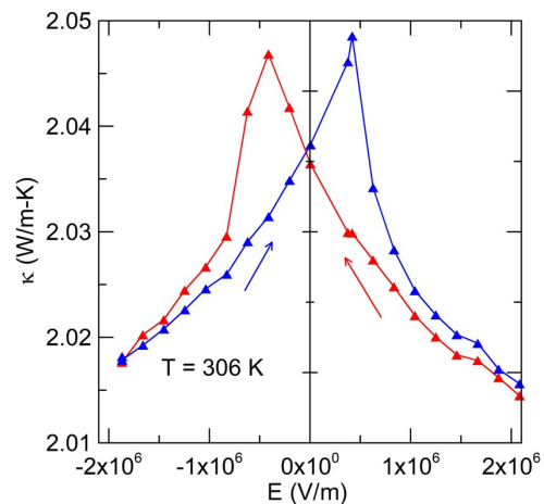
Figure 3. Electric field dependence of the thermal conductivity of the ferroelectric PZT (adapted from [41] )
