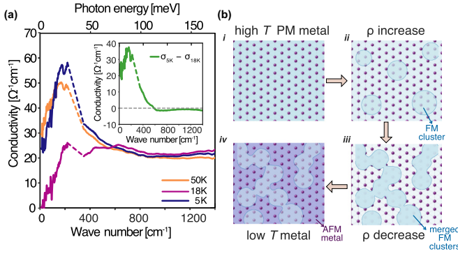
FIG. 5. (a) Optical conductivity at 50, 18, and 5 K, showing electron localization at 18 K. The inset is the difference between the 5- and the 18-K data, showing the conduction electron spectral weight. The dashed lines are interpolations across a region where the measurement is dominated by the spectral weight of an optical phonon. (b) Schematic temperature evolution of the coupled Eu-electron system.
