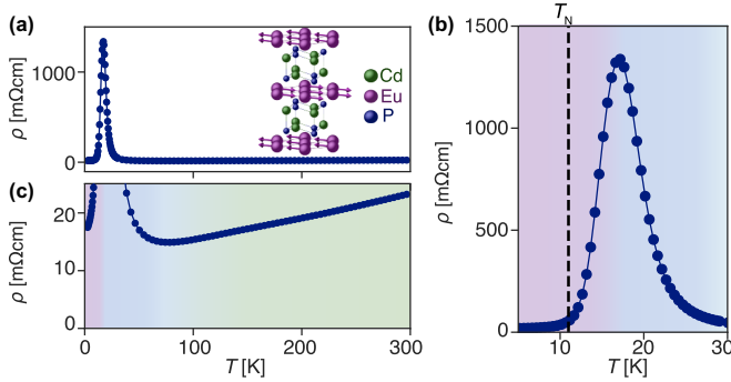
FIG. 1. (a) and (b) The resistivity of \text{EuCd}_2\text{P}_2 (structure in the inset) shows a pronounced peak at 18 K. (c) Above 75 K it exhibits metallic behavior. Data are from Ref. [5].
