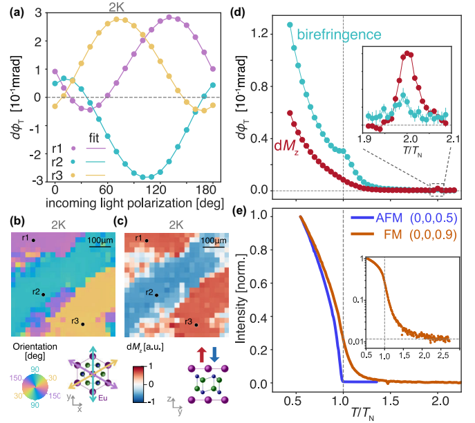
FIG. 2. (a) Thermally modulated polarization rotation as a function of incident polarization and corresponding fits [Eq. (1)], measured at three sample locations (probe: 20 \mu\text{W} , 633 nm; pump: 50 \mu\text{W} , 780 nm, modulated at 2345 Hz). (b) and (c) Maps of (b) principal axis orientation and (c) dM_z , extracted from the phase and offset of curves, such as those in (a) (step size: 25 \mu\text{m} , light spot diameter: 5 \mu\text{m} ). (d) Thermally modulated birefringence amplitude (teal) and dM_z (red) as a function of temperature ( T_N = 11.5 K). Both signals onset at \sim 2T_N (the inset). (e) Normalized antiferromagnetic [blue; ( h, k, l ) = (0, 0, 0.5)] and ferromagnetic [orange; ( h, k, l ) = (0, 0, 0.9) with structural scattering subtracted] resonant elastic x-ray scattering (REXS) as a function of temperature. AFM scattering onsets sharply at T_N , in contrast to the gradual onset of ferromagnetism around 2T_N , emphasized in the logarithmic plot in the inset.
