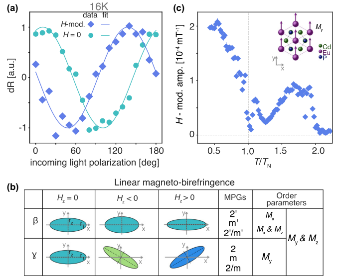
FIG. 3. (a) The phase difference between the H_z -linear birefringence (diamonds) and the H = 0 birefringence (circles) proves \gamma \neq 0 Eq. (3), and, therefore, M_y \neq 0 [the inset of (c)]. For clarity the curves are normalized by the respective amplitudes, and constant offsets are subtracted. (b) Diagonal ( \beta ) and off-diagonal ( \gamma ) LMB: the orientation and length of the ellipse axes represent the orientation of the optic principal axes and the reflectivity along them, respectively. Magnetic point groups (MPGs) and order parameters compatible with the two effects are listed. (c) The amplitude of the LMB as a function of temperature ( T_N = 11.5 K) reveals the onset of TR—and C_3 —broken phase at \sim 2T_N . Probe beam: 20 \mu\text{W} , 633 nm; field amplitude: 0.2 mT, modulated at 500 Hz.
