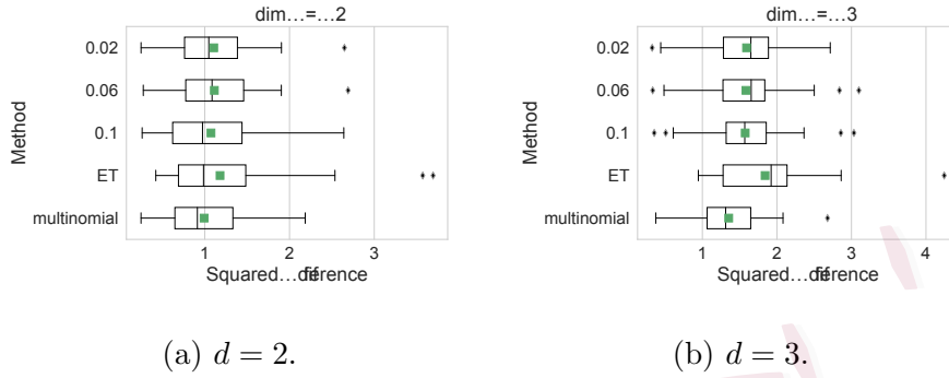
Figure 4: Simulation results for the stochastic volatility model in different dimensions. Boxplots of squared differences over 50 independent experiments, with mean values indicated by green squares. Here, T = 40 , particle numbers are 50.
