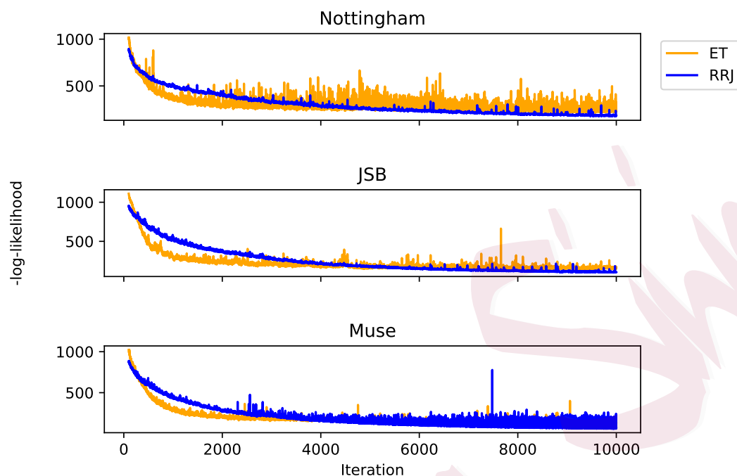
Figure 6: The likelihood evaluation for VRNN model in a single run. The first 100 burn-in steps are omitted.
