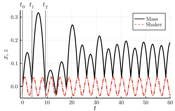
Fig. 2 An example waveform, with impacts occurring at t_0, t_1, t_2, \dots . The transient response overshoots the steady-state amplitude before converging to a periodic solution
