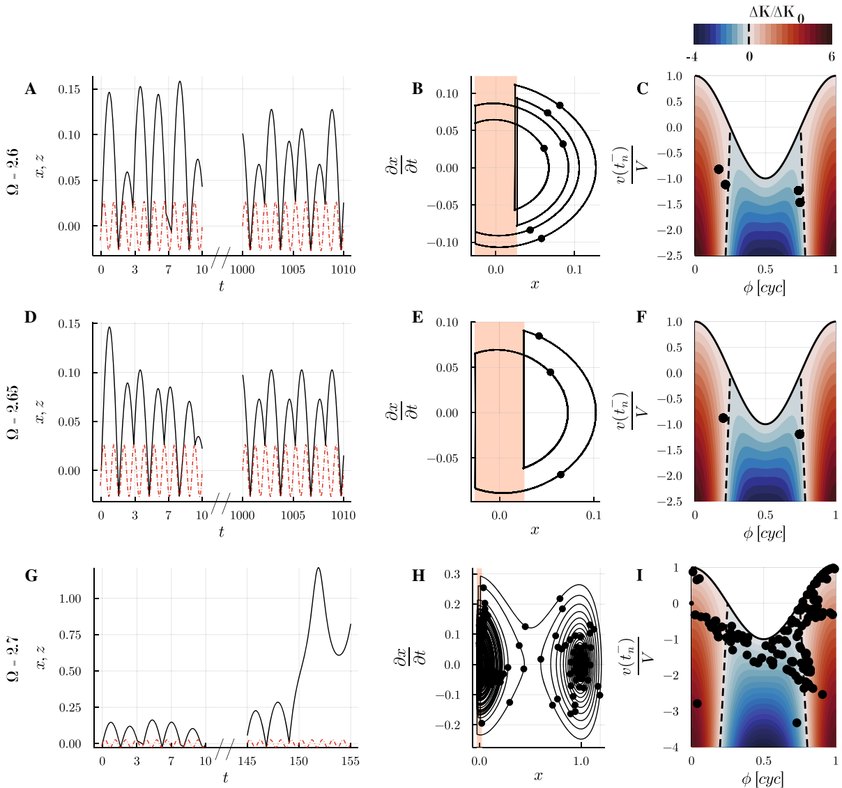
Fig. 5 Same as Fig. 4 but for higher excitation frequencies. Panels h & i include transient response. An intrawell to interwell bifurcation is observed with increasing frequency. As fre-
