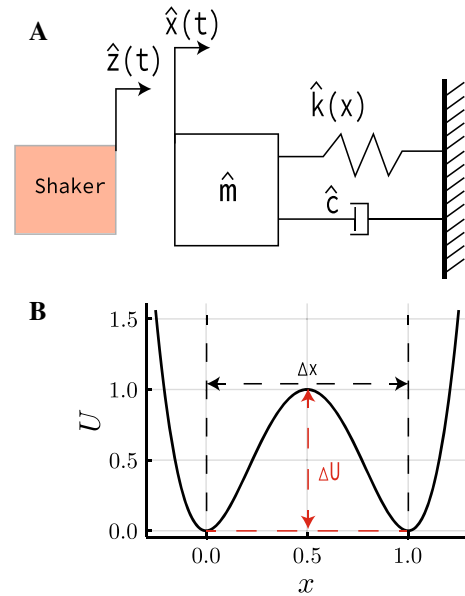
Fig. 1 a Lumped system with dimensional parameters. b Bistable potential energy profile. \Delta x is the distance between energy minima, and \Delta U is the energy barrier
