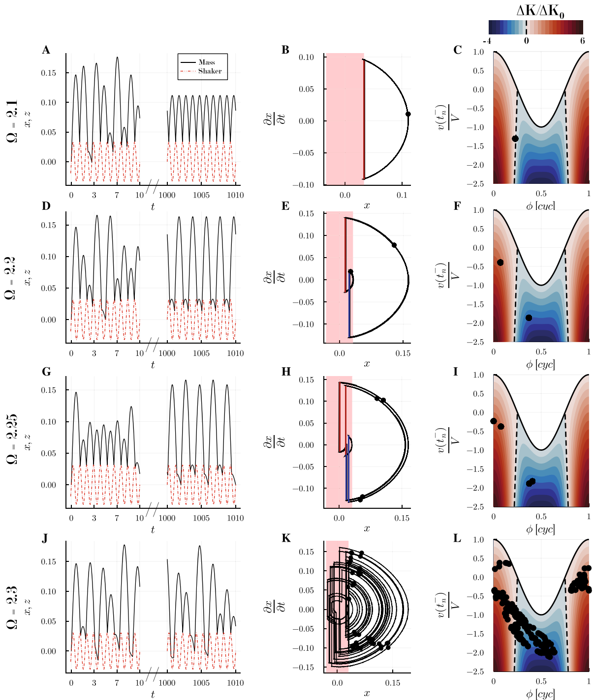
Fig. 4 Transition to chaos as frequency increases for V = 0.07 . a, d, g, j Waveforms showing both transient and steady-state responses. b, e, h, k Phase plane with overlaid Poincaré section for steady-state response. The shaded region indicates the range
