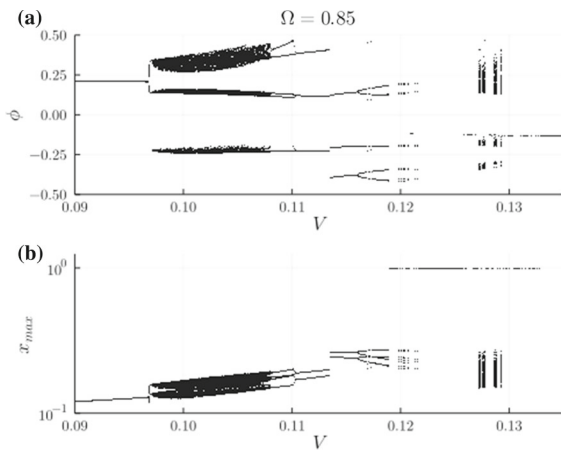
Fig. 8 Interwell bifurcation occurs with increasing velocity with \Omega = 0.85 . Vertical lines indicate values shown in Fig. 7. At low velocities, the system is periodic. As velocity increases, the response period increases toward chaos. Finally, the mass travels to the second equilibrium in either transient or continuous interwell responses
