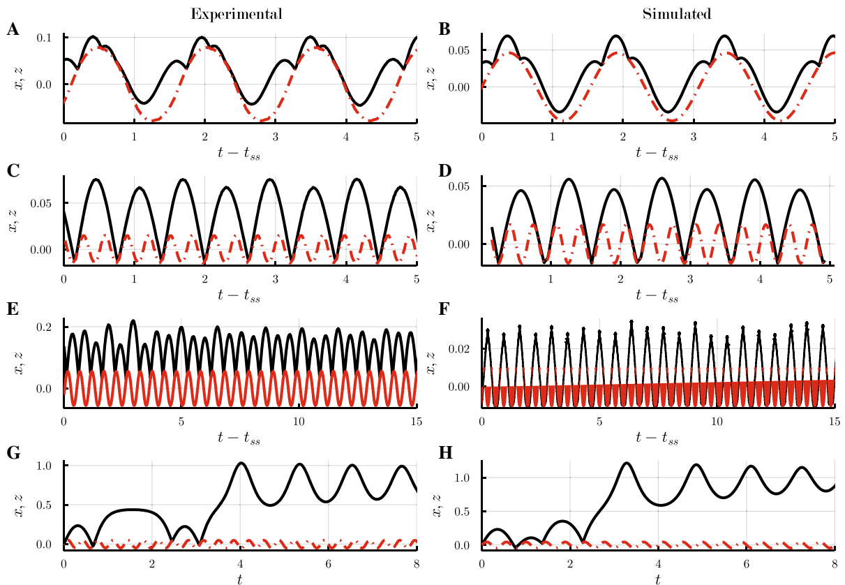
Fig. 14 Representative waveforms showing qualitative similarities between simulation and experiment. t_{ss} represents sufficient delay to reach a steady-state response. a Period-one intrawell, \Omega = 0.649 , V = 0.025 . b Period-one intrawell, \Omega = 0.65 , V = 0.03 . c Period-four intrawell, \Omega = 3.247 , V = 0.03 . d
