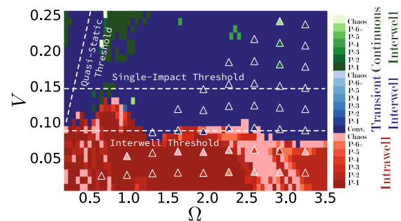
Fig. 13 Experimental (shaded triangles) and theoretical (colormap) results for the influence of shaker amplitude and frequency on the nonlinear dynamics of the system. e = 0.7 to match experimentally determined value. (Color figure online)
