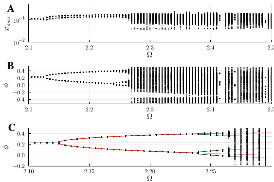
Fig. 6 Bifurcation diagram when \Omega is used a control parameter while V = 0.07 . a Maximum displacement of the mass within each cycle of the shaker displacement. b Phase of the impacts. Vertical red lines indicate values shown in Fig. 5c. Phase of impacts for \Omega between 2.10 and 2.30. Continuous lines indicate predicted periodic responses described in Supplemental Information. Thick and thin lines correspond to stable and unstable solutions, respectively. Blue, red and green lines correspond to period-one, period-two and period-four solutions, respectively. As frequency increases, a series of period-doubling bifurcations occurs until a region of chaos is reached. At higher frequencies, stability is regained and the mass eventually exceeds the energy barrier and moves to the second equilibrium. (Color figure online)
