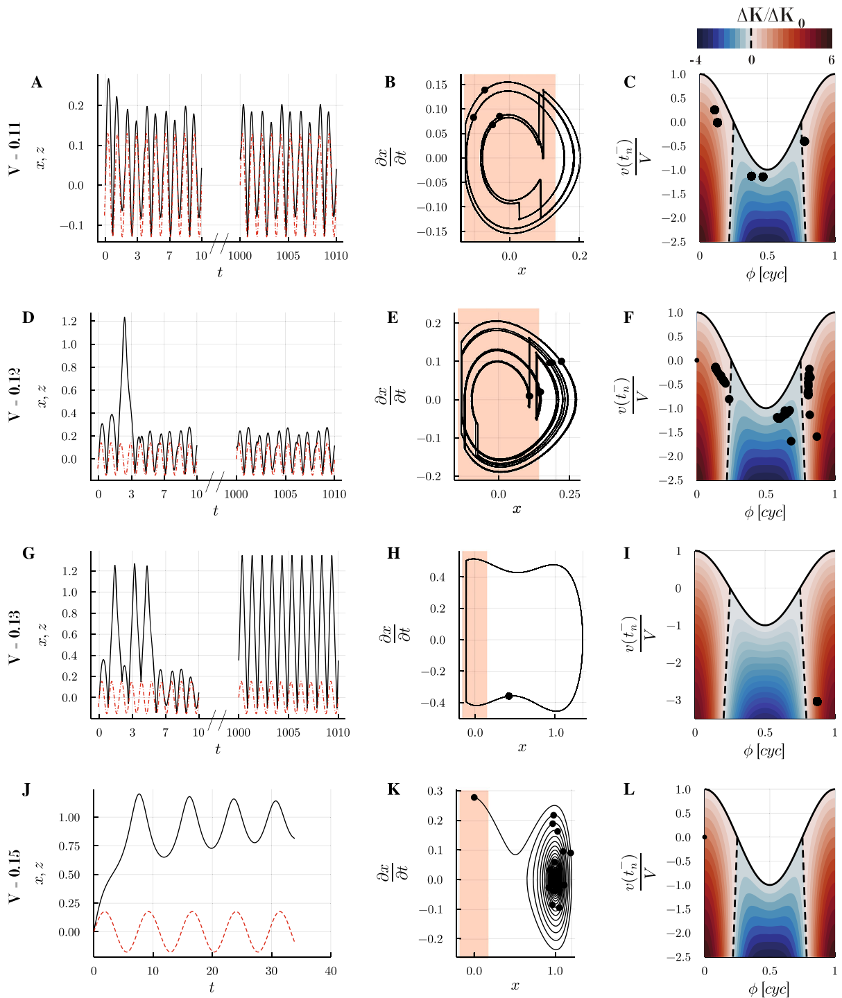
Fig. 7 Same as Fig. 5 for \Omega = 0.85 as velocity is increased. As velocity increases, a bifurcation from intrawell to interwell responses occurs
