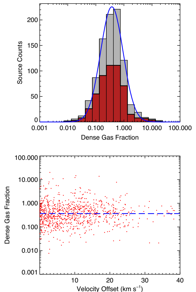
Figure 8. Distribution of the GMC DGF determined by summing the masses of all embedded clumps and dividing by the GMC mass. The upper panel shows the distribution of the whole GMC sample (grey histogram) while the red histogram shows the distribution of clouds located within 10 km s -1 of a spiral arm. The lower panel shows the distribution of DGF of each cloud as a function of velocity offset from their nearest spiral arms. The dashed blue line shows the results of a linear least-squares fit to the \log_{10}[\text{DGF}] and the velocity offset; this has a slope of (-1.8 \pm 0.97) \times 10^{-3} , which is essentially flat. The bin size used in the upper panel is 0.25 dex. The blue curve is the result of a lognormal fit to the distribution of the whole GMC sample.
