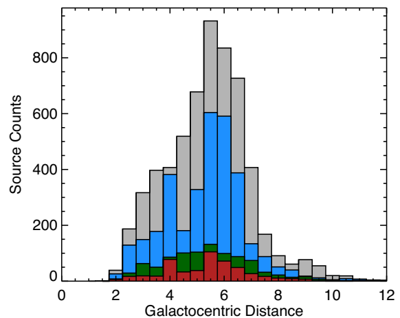
Figure 11. Distribution of GMCs as a function of Galactocentric distance. The distribution of the whole sample is shown in grey, those located within 10 \text{ km s}^{-1} of a spiral arm, are shown in blue. The clouds associated with dense gas are shown in green and the population of these clouds that are within the 10 \text{ km s}^{-1} of a spiral arm are shown in red. The bin size used is 0.5 kpc.
