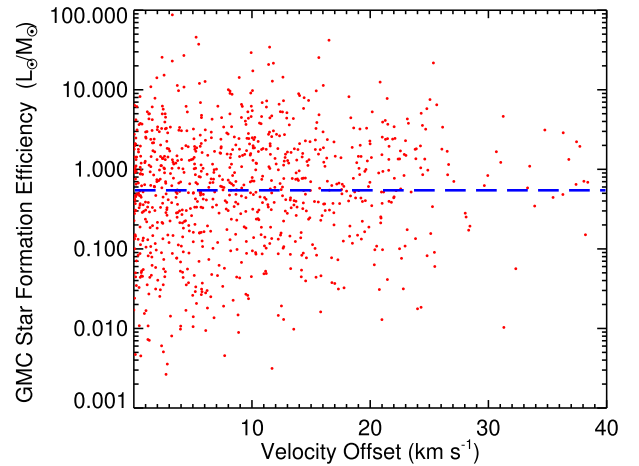
Figure 9. As Fig. 8 but for the SFE. The dashed blue line shows the results of a linear least-squares fit to the \log_{10}[\text{SFE}] and the velocity offset; this has a slope of 6.9 \times 10^{-5} \pm 1.7 \times 10^{-3} , which is essentially flat. The bin size used in the upper panel is 0.25 dex.
