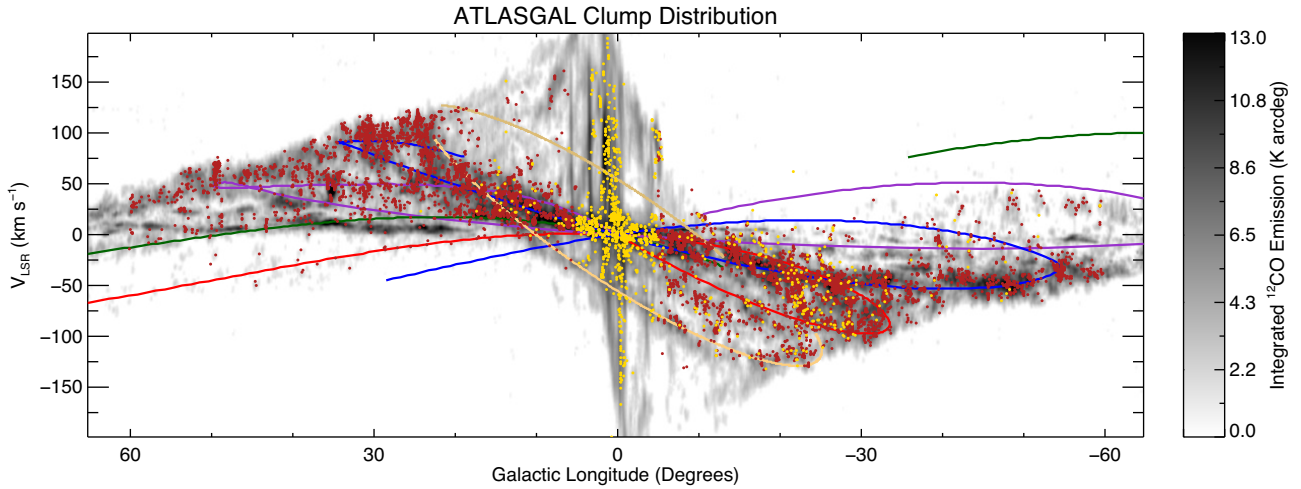
Figure 6. Galactic longitude-velocity distribution of all ATLASGAL sources located between 300^\circ < \ell < 60^\circ for which we have been able to assign a velocity. The grey-scale image shows the distribution of molecular gas as traced by the integrated ^{12}\text{CO} (1–0) emission for comparison (Dame, Hartmann & Thaddeus 2001). The red circles mark the positions of clumps where the velocity has been drawn from Urquhart et al. (2018), while the yellow circles mark the positions of clumps where a velocity has been determined from the work presented in this paper. The location of the spiral arms is shown as curved solid lines (colours are as given in Fig. 1). The positions of the four main spiral and local arms have been taken from the model of Taylor & Cordes (1993) and updated by Cordes (2004).
