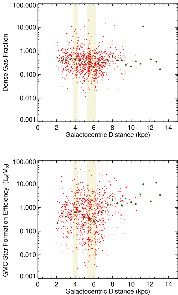
Figure 12. Distribution of the GMC DGF and SFE as a function of distance from the Galactic Centre. The vertical shaded areas on both plots correspond to regions in Galactocentric radius where the cloud population is dominated by the near sides of the Norma and Scutum arms (4 and 5.75 kpc, respectively). The green circles indicate the average value calculated for each 0.5 kpc.
