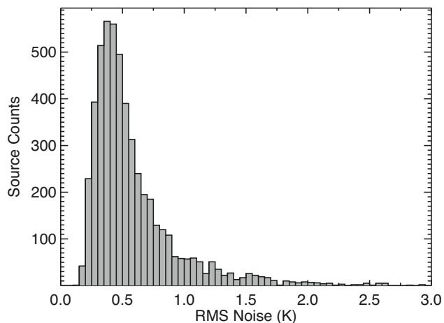
Figure 2. Distribution of rms noise values determined from the emission free regions of the \text{C}^{18}\text{O} (2–1) spectra smoothed to a velocity resolution of 1 \text{ km s}^{-1} . The bin size is 0.05 \text{ K} .
