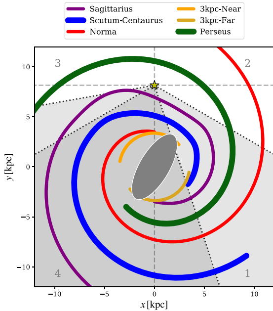
Figure 1. Schematic showing the loci of the spiral arms according to the model by Taylor & Cordes (1993) and updated by Cordes (2004), with an additional bisymmetric pair of arm segments added to represent the 3 kpc arms. The light grey shaded area is the region covered by the ATLASGAL survey while the darker grey area indicates the region of the plane covered by the SEDIGISM survey. The star indicates the position of the Sun and the numbers identify the Galactic quadrants. The bar feature is merely illustrative and does not play a role in our analysis.
