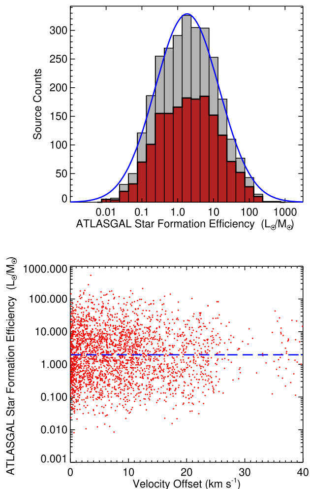
Figure 10. As Fig. 8 but for the ATLASGAL clump SFE. The dashed blue line shows the results of a linear least-square fit to the \text{Log}_{10}[\text{SFE}_{\text{clump}}] and the velocity offset; this has a slope of (9.1 \pm 1.5) \times 10^{-4} , which is essentially flat. The bin size used in the upper panel is 0.25 dex.
