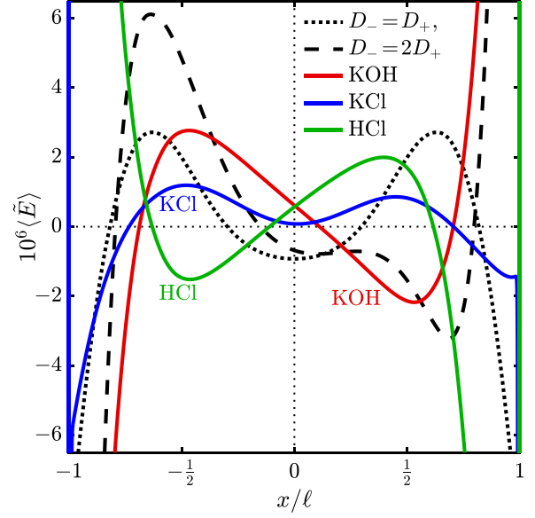
FIG. 7. Spatial structure of the dissymmetric AREF for different 1-1 binary electrolytes. Parameters: \phi_0 = 10\phi_T for (b), f = \omega/(2\pi) = 50 Hz for (a), \alpha = 2 , 2\ell = 20 \mu\text{m} , c^\infty = 1 \text{ mM} . The reference results correspond to D_+ = 10^{-9} \text{ m}^2/\text{s} .
