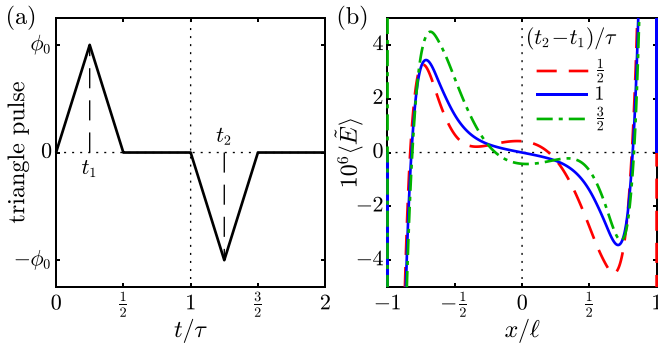
FIG. 8. Dissymmetric AREF due to a zero-time-average triangular pulse potential applied at x = -\ell . (a) Positive (at t = t_1 ) and negative (at t = t_2 ) triangular pulses of width \frac{1}{2}\tau and amplitude \phi_0 . (b) The corresponding induced AREF for different values of (t_2 - t_1)/\tau . Parameters: \phi_0 = 20\phi_T , 1/(2\tau) = 50 Hz, 2\ell = 20 \mu\text{m} , D_+ = 10^{-9} \text{m}^2/\text{s} , D_-/D_+ = 2 , c^\infty = 1 mM.
