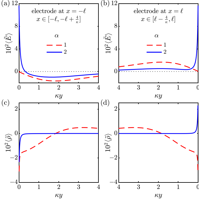
FIG. 3. Representative numerical solutions to (a), (b) the AREF \langle \tilde{E} \rangle = \langle E \rangle / (\kappa \phi_T) and (c), (d) time-average free charge density \langle \tilde{\rho} \rangle = \langle \rho \rangle / n^\infty , for two-mode applied potentials [\phi(t, -\ell) = \phi_0[\sin(\omega t) + \sin(\alpha \omega t)], \phi(t, \ell) = 0] at the Debye scale. For visualization purposes, the \langle \tilde{\rho} \rangle data for \alpha = 2 in (c) and (d) are divided by 100. The spatial variable y denotes the distance from the corresponding electrode. Parameters: \phi_0 = 10\phi_T , f = \omega/(2\pi) = 50 Hz, 2\ell = 20 \mu\text{m} , D_+ = 10^{-9} \text{ m}^2/\text{s} , D_-/D_+ = 2 , c^\infty = 1 \text{ mM} .
