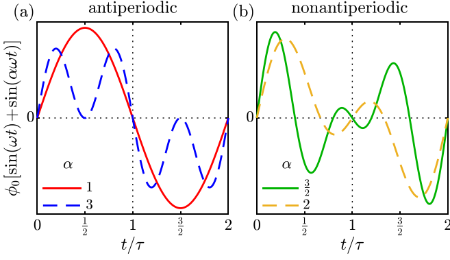
FIG. 5. Examples of (a) antiperiodic and (b) nonantiperiodic two-mode applied potentials \phi_0[\sin(\omega t) + \sin(\alpha\omega t)] .
