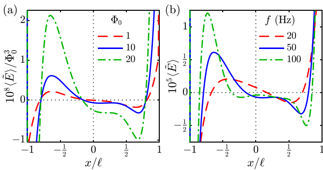
FIG. 6. Effects of the (a) two-mode potential amplitude and (b) frequency on the dissymmetric AREF. For visualization purposes the data in (a) are scaled by \Phi_0^3 with \Phi_0 = \phi_0/\phi_T . Parameters: \phi_0 = 10\phi_T for (b), f = \omega/(2\pi) = 50 Hz for (a), \alpha = 2 , 2\ell = 20 \mu\text{m} , D_+ = 10^{-9} \text{ m}^2/\text{s} , D_-/D_+ = 2 , c^\infty = 1 \text{ mM} .
