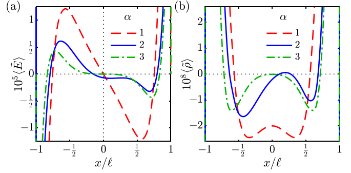
FIG. 2. Representative numerical solutions to (a) the AREF \langle \tilde{E} \rangle = \langle E \rangle / (\kappa \phi_T) and (b) time-average free charge density \langle \tilde{\rho} \rangle = \langle \rho \rangle / n^{\infty} , for two-mode applied potentials [\phi(t, -\ell) = \phi_0[\sin(\omega t) + \sin(\alpha\omega t)], \phi(t, \ell) = 0] in the bulk electrolyte. Parameters: \phi_0 = 10\phi_T , f = \omega/(2\pi) = 50 Hz, 2\ell = 20 \mu\text{m} , D_+ = 10^{-9} \text{ m}^2/\text{s} , D_-/D_+ = 2 , c^{\infty} = 1 \text{ mM} .
