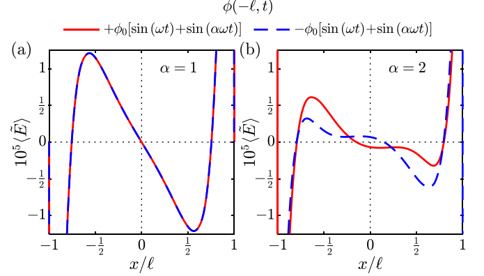
FIG. 4. Flipping the sign of the applied potential at x = -\ell for (a) \alpha = 1 and (b) \alpha = 2 . Parameters: \phi_0 = 10\phi_T , f = \omega/(2\pi) = 50 Hz, 2\ell = 20 \mu\text{m} , D_+ = 10^{-9} \text{ m}^2/\text{s} , D_-/D_+ = 2 , c^\infty = 1 \text{ mM} .
