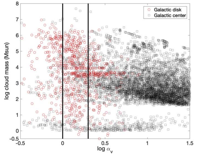
Figure 2. Cloud mass as a function of \alpha_v for the Galactic disk clouds (open red circle) and Galactic center clouds (open black squares). The two vertical lines indicate clouds with \alpha_v = 1 and 2, respectively, for reference.
