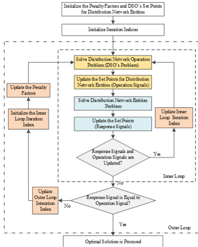
Fig. 5. Distribution Network Operation Framework
