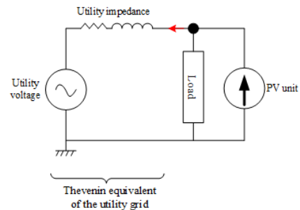
Fig. 2. Utility grid connected to PV generation
