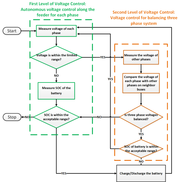
Fig. 3. Two-level control strategy to: a) regulate the phase voltage; b) to balance the three-phase voltage along the distribution feeder
