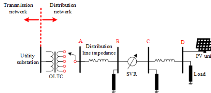
Fig. 1. Distribution network with voltage regulation assets
