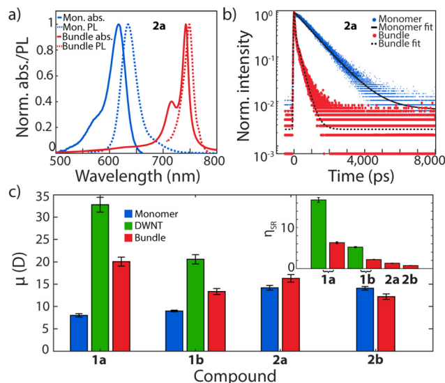
Fig. 3 Photophysical characterization of monomers and aggregates of 2a/2b . (a) Absorption (solid) and photoluminescence (dotted) spectra for 2a monomer (1 mM dye, 100% methanol) and bundle (1 mM dye, 10% methanol/water; emission from 750 nm peak). (b) Monomer lifetime, bundle lifetime, and corresponding fits for 2a . (c) Transition dipole moments for all monomers (blue) and aggregate morphologies (green, red) (inset: superradiance parameter \eta_{SR} for each aggregate morphology).
