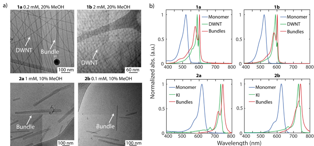
Fig. 2 (a) Cryo-electron microscopy images of trimethine double-walled nanotubes and pentamethine bundles. (b) Morphological characterization of monomers and aggregates of 1a , 1b , 2a , and 2b . Absorption spectrum of trimethine ( 1a and 1b ) and pentamethine ( 2a and 2b ) dye monomers (100% MeOH) and aggregates (DWNT = double-walled nanotube, KI = kinetic intermediate).
