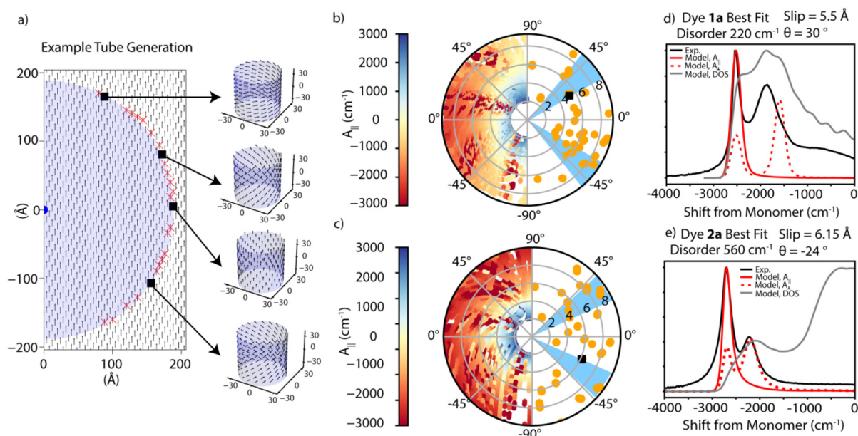
Fig. 4 (a) Examples of the tube-wrapping simulation used for bundles of 2a . (b and c) Polar plots of 1a (b) and 2a (c) visualizing the computational screening conditions of slip and chiral angle used to find matches between the monomer to aggregate shift and relative ratios of aggregate peaks. The degree of blue/redshift for each slip/chiral angle is given on the left side of the plot. The space of possible solutions screened (right side) is shaded in blue, with yellow dots indicating possible solutions, and a black dot indicating the best match to experimental data. (d and e) Experimental and modelled absorption spectra/DOS of 1a (d) and 2a (e) from screening fits shown in Fig. 4b.
