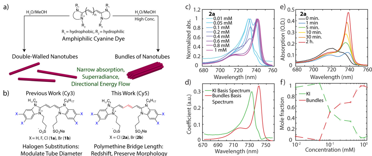
Fig. 1 (a) Self-assembly of amphiphilic cyanine dyes into J-aggregate nanostructures. (b) Synthetic modifications on C8S3 ( 1a ) in prior work (modifying halogen substitution/placement) and this work (trimethine to pentamethine). (c) Normalized absorption of variable concentration samples of 2a . All samples created using 10% MeOH, 90% H_2O using the procedure in ESI section 4.† (d) Basis spectra for kinetic intermediate and bundles of 2a achieved through non-negative matrix factorization of the concentration series in 1c. (e) Kinetic time series of a 2a aggregate created at 10% MeOH, 90% H_2O and 0.05 mM dye. (f) Plot of the normalized relative mole fraction of kinetic intermediate vs. bundles changing as a function of concentration.
