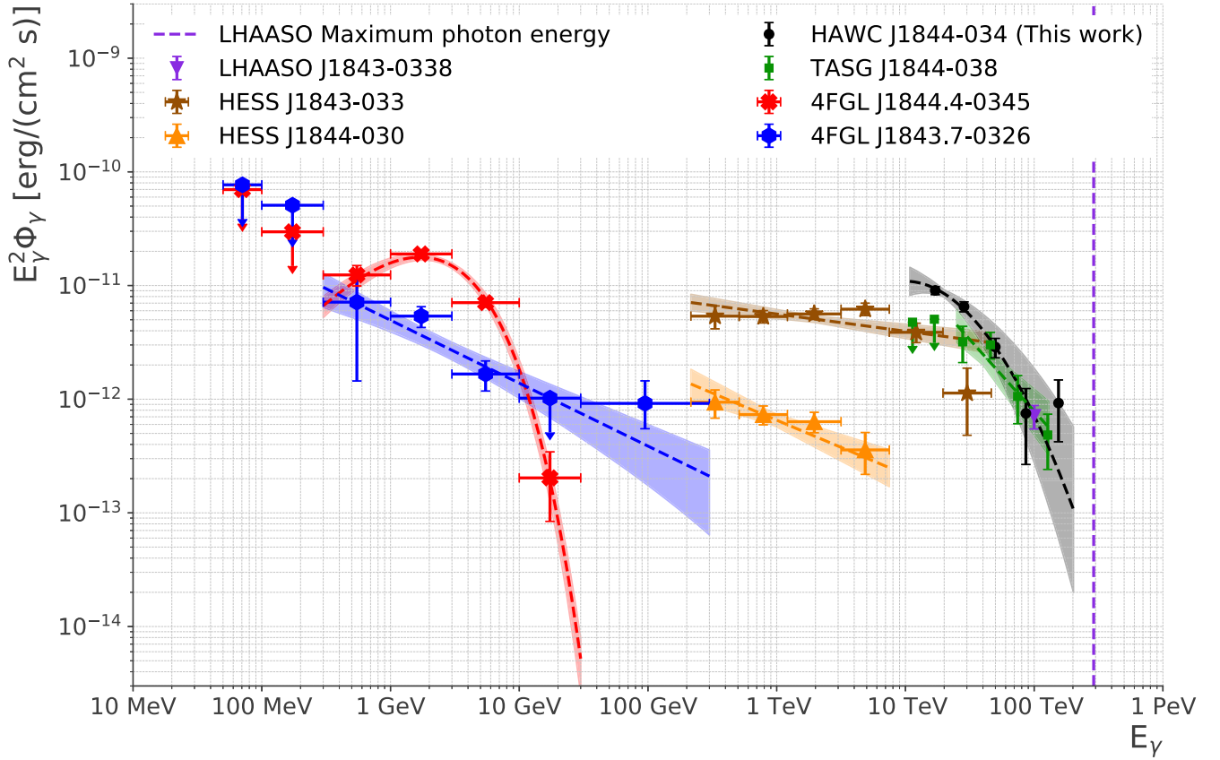
Figure 7. Collection of spectra for \gamma -ray sources within the vicinity of HAWC J1844–034. The results have been collected from Fermi-LAT (Abdollahi et al. 2020), H.E.S.S. (H.E.S.S. Collaboration et al. 2018), Tibet AS-Gamma (Amenomori et al. 2022), LHAASO (Cao et al. 2021), and HAWC.
