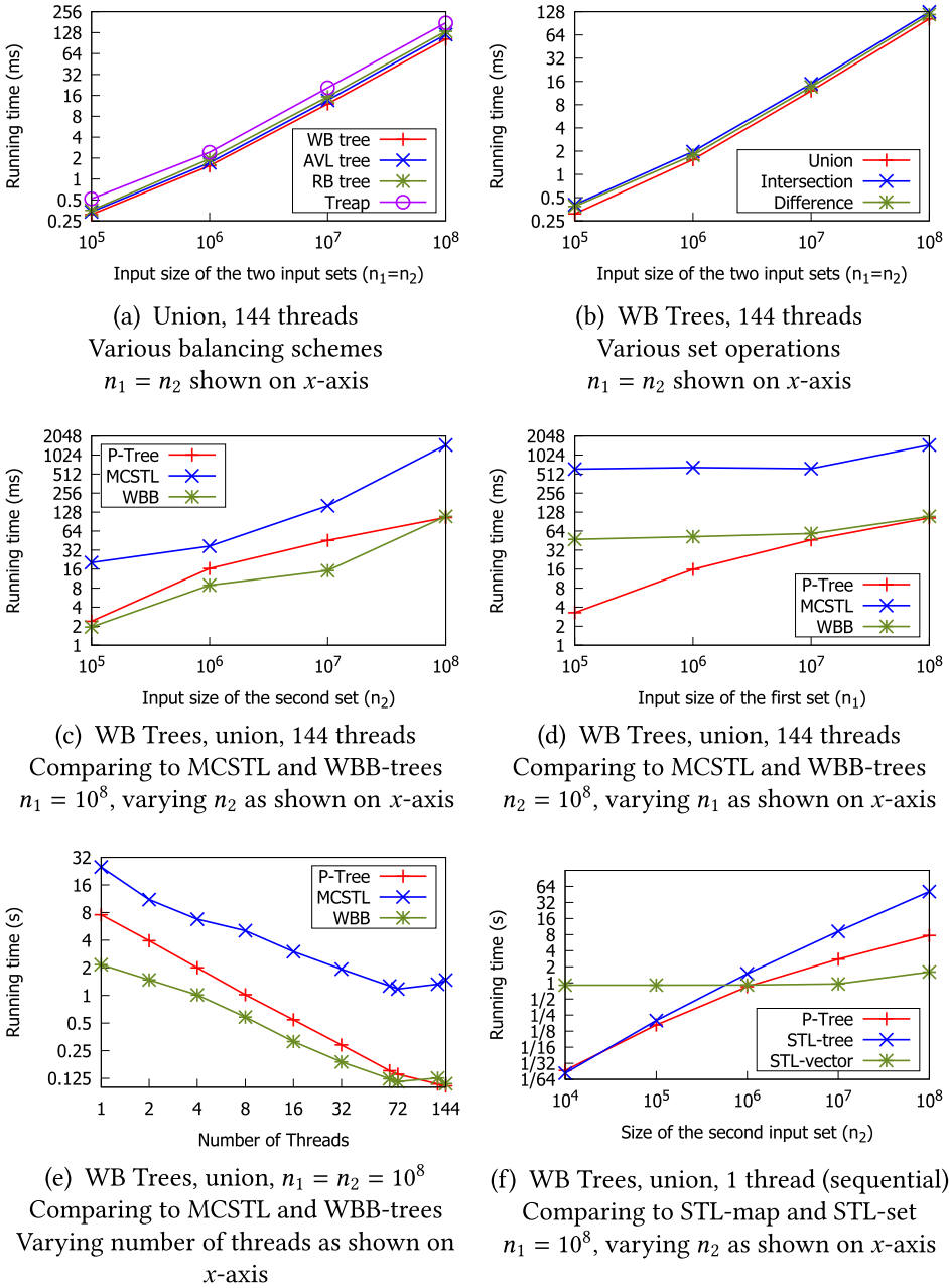
Fig. 16. Experimental results on join -based algorithms.
