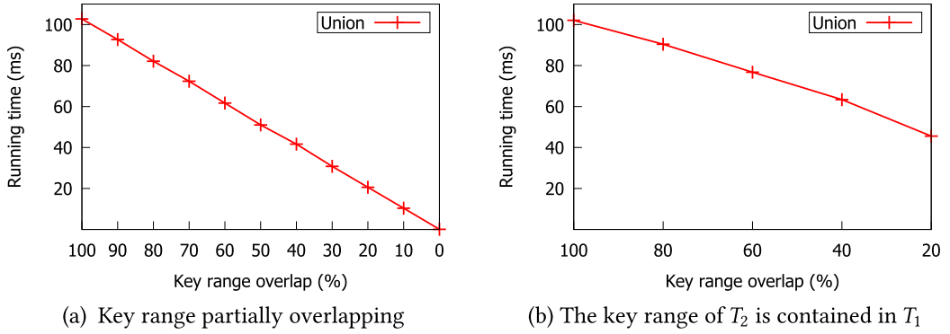
Fig. 17. The running time of union algorithm on two input trees with different key range overlapping. We use WB trees and 144 threads. The numbers on the x-axis show how much the key ranges of the input sets overlap.
