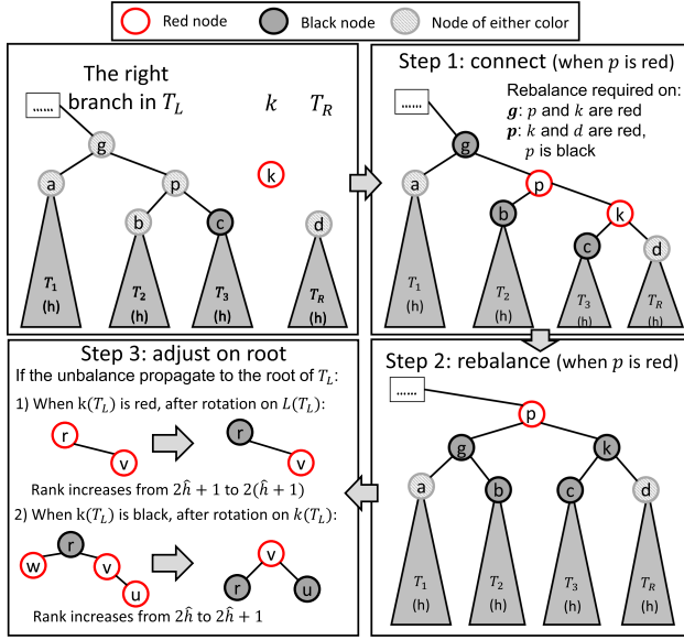
Fig. 7. An example of join on red-black trees. An example of join on red-black trees ( \hat{h} = \hat{h}(T_L) > \hat{h}(T_R) ). We follow the right spine of T_L until we find a black node with the same black height as T_R (i.e., c ). Then a new red node (c, k, T_R) is created, replacing c (Step 1). The only invariant that can be violated is when either c 's previous parent p or T_R 's root d is red. If so, a left rotation is performed at some black node. Step 2 shows the rebalance when p is red. The black height of the rotated subtree (now rooted at p ) is the same as before ( h + 1 ), but the parent of p might be red, requiring another rotation. If the red-rule violation propagates to the root, the root is either colored red, or rotated left (Step 3).
