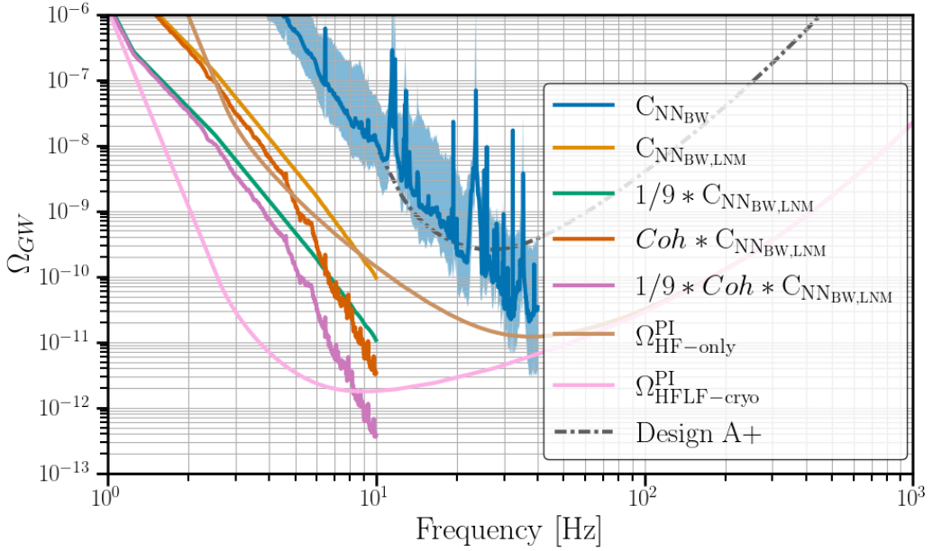
Figure 34. The projected impact from correlated NN from body-waves C_{\text{NNBW}} , as calculated in section III of [141], is shown in blue. The blue line represents the median value, and the associated surface is delimited by the 10% and 90% percentiles. Also curves with more optimistic assumptions (see the text) are shown. Based on figure 16 of [141]. Adapted with permission from [141], copyright (2022) by the American Physical Society.
