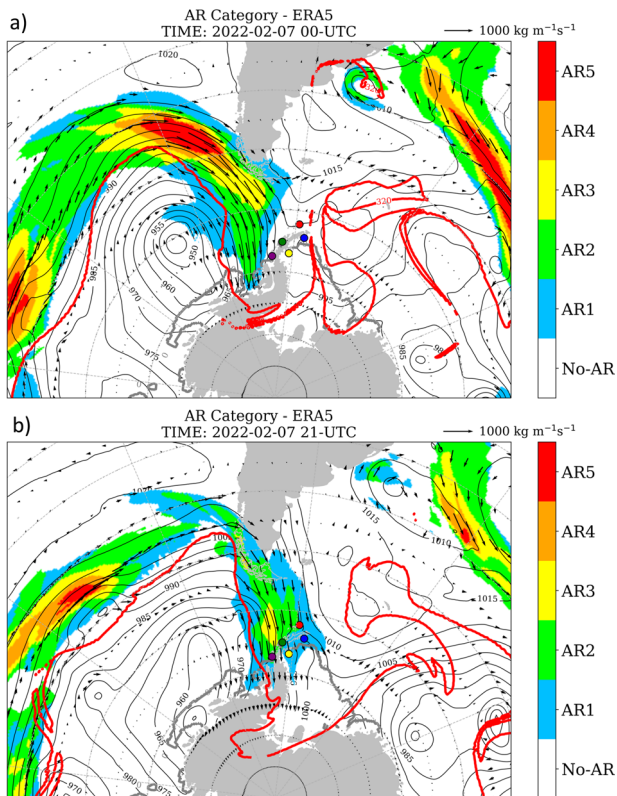
Fig. 4 Atmospheric river and Rossby wave breaking. AR scale (shading), integrated vapor transport (IVT) vectors ( \text{kg m}^{-1} \text{s}^{-1} , black arrows), mean sea level pressure (hPa, black contours), 320-K potential temperature on the dynamic tropopause ( -2 \text{ PVU} surface) (thick red line) and sea ice edge (identified as the 10% sea ice concentration) (thick gray line) for 7 February 2022 at a 00 UTC and b 21 UTC. Colored circles show station locations: King George Island (red), Vernadsky (green), Rothera (brown), Marambio (blue), and Larsen C north AWS (yellow). Based on ERA5 reanalysis.
