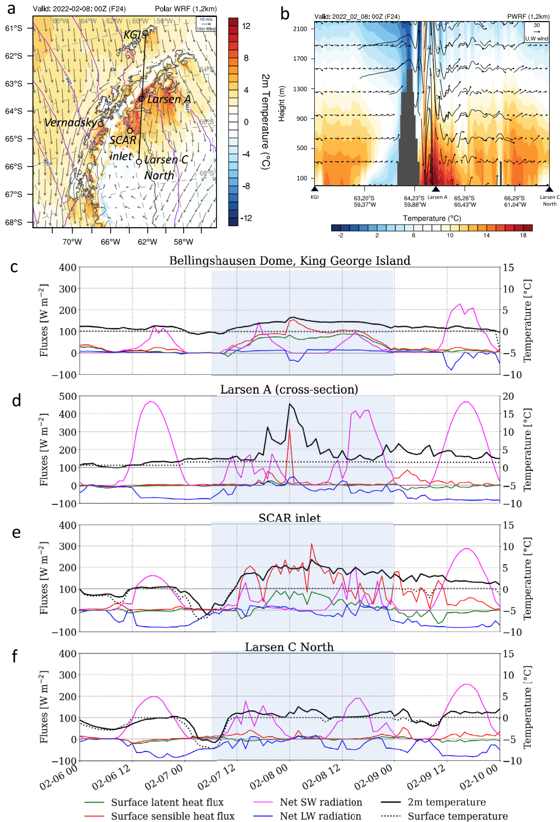
Fig. 5 High-resolution analysis of temperature, wind and heat fluxes over the northern AP. a 2-m air temperatures (°C, shaded), 10-m wind ( \text{m s}^{-1} , vectors) and mean sea level pressure (hPa, violet contours). Thin black line indicates the cross-section in (b) . b Air temperature (°C, shading) and wind ( \text{m s}^{-1} , vectors, with 10x scaling for the vertical component) cross-section from King George Island (KGI, Bellingshausen Dome) to Larsen C north AWS location (passing through Larsen A) from near the surface (4-m above ground) up to 2200 m height, including topography (dark gray). c–f Time series of surface latent (green) and sensible heat fluxes (red), net SW (magenta) and net LW (blue) radiative fluxes, 2-m air temperature (black line) and skin temperature (black dots) at the point locations with ice and/or snow surfaces for c Bellingshausen Dome (King George Island, Collins glacier), d Larsen A (cross-section point), e SCAR inlet, and f Larsen C north (AWS location). All fields are the output from the Polar WRF, 1.2-km resolution domain (3-domain run forced with ERA5, see “Methods”).
