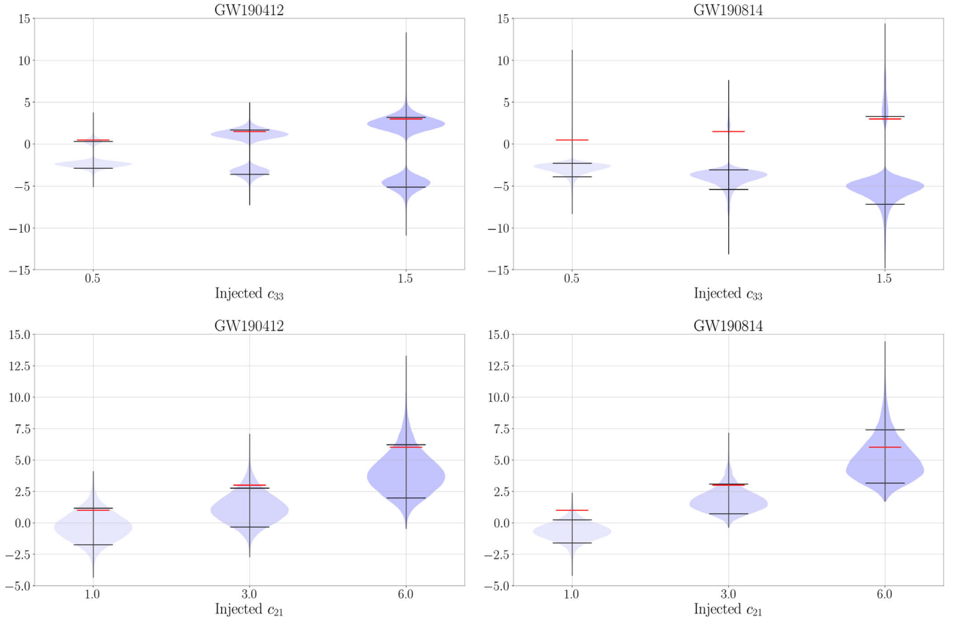
FIG. 6. Violin plots for the posterior density distributions of c_{33} (top row) and c_{21} (bottom row), for injections similar to GW190412 (left column) and GW190814 (right column). In each case the black horizontal bars indicate 90% confidence intervals, and the red horizontal bar the injected value; the black vertical line shows the support of the posterior.
