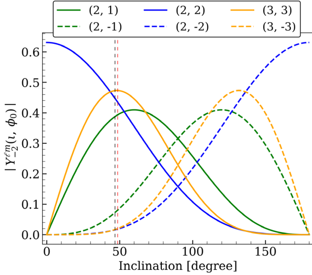
FIG. 1. The absolute values of spin-weighted spherical harmonics of weight -2 as function of the inclination angle \iota . The vertical lines indicate the peak likelihood values of \iota for GW190412 (black dashed) and GW190814 (red dashed), located at \approx 47^\circ and \approx 49^\circ , respectively [26,27].
