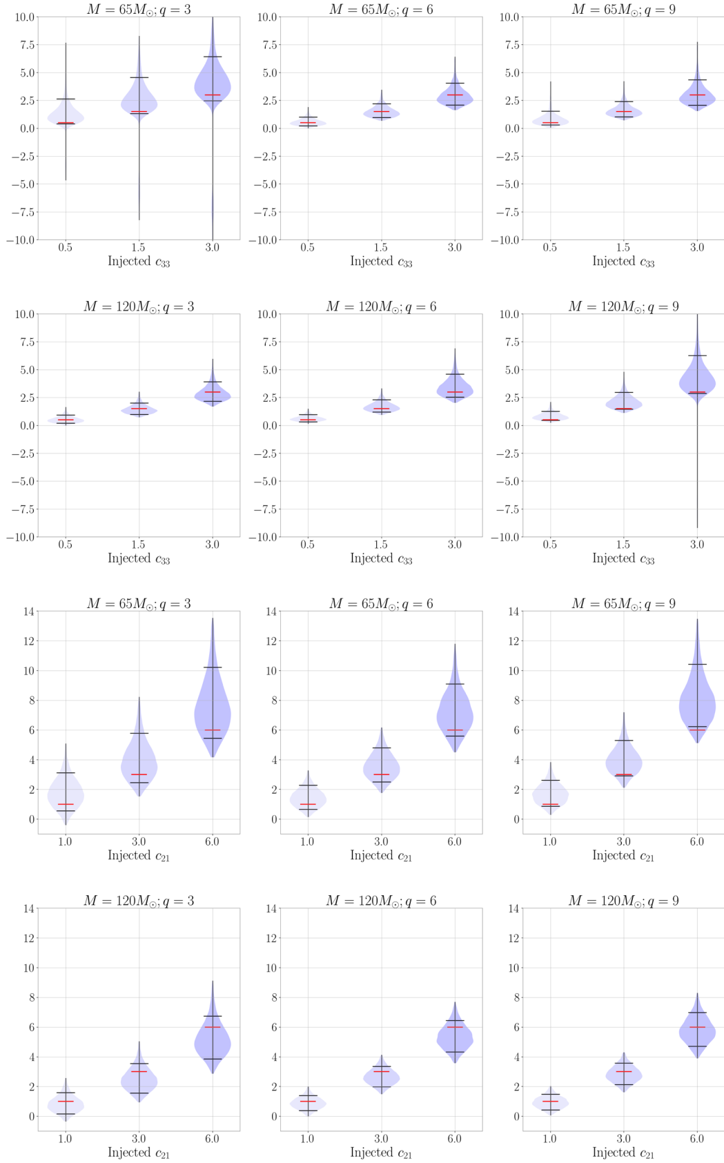
FIG. 4. Violin plots for the posterior density distributions of c_{33} (top two rows) and c_{21} (bottom two rows), for M = 65, 120 M_{\odot} , and q = 3 (left column), q = 6 (middle column), and q = 9 (right column). In each case the black horizontal bars indicate 90% confidence intervals, and the red horizontal bar the injected value; the black vertical line shows the support of the posterior.
