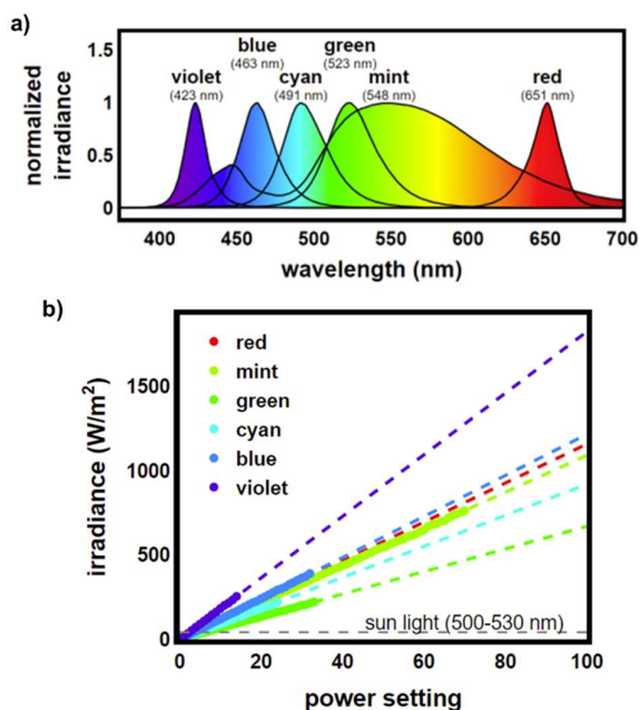
Fig. 6 a) Normalized emission spectra for each color LED on the photochemical platform. b) Irradiance vs power setting for all 6 LED colors. Measurements were taken at 80 mm below the light setup with mirrors. Data points were taken starting at the lowest power setting and increasing until the detector reached its max irradiance limit. Linear fits were applied to the data collected and projected to the max power setting.
