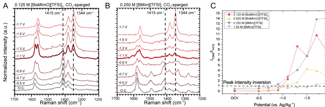
Figure 5. In situ SERS spectra of 0.125\text{ M} [\text{BisMImO}][\text{TFSI}]_2 (A) and 0.250\text{ M} [\text{BMIm}][\text{TFSI}] (B) under \text{CO}_2 -sparged conditions. The potential at which the 1344\text{ cm}^{-1} peak intensity surpasses the 1415\text{ cm}^{-1} peak is bolded. The relative intensities of the 1344 and 1415\text{ cm}^{-1} peaks are used to determine the extent of imidazolium reorientation (C). The normalized peak intensity of the 1344\text{ cm}^{-1} peak surpasses that of the 1415\text{ cm}^{-1} peak at -1.1\text{ V} vs. \text{Ag}/\text{Ag}^+ for both samples. Comparing the ratios of the peak intensities of the 1344 to 1415\text{ cm}^{-1} peaks, we find that the 1.65\text{ M} [\text{BMIm}][\text{TFSI}] inversion potential is more negative than the other ionic liquid concentrations. The inversion potential for the 0.825\text{ M} [\text{BisMImO}][\text{TFSI}]_2 remains similar to the lower concentration electrolytes, which suggests that the covalent link provides a “pre-structuring” effect between the two imidazoliums of the [\text{BisMImO}]^+ cation.
