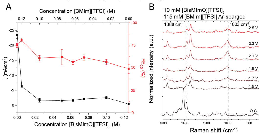
Figure 6. Results of mixed electrolytes demonstrate the preferential accumulation of the [\text{BisMImO}]^{2+} cation. Steady state electrolysis (A), where current density (black) and faradaic efficiency for CO (red) in mixtures of [\text{BisMImO}][\text{TFSI}]_2 and [\text{BMIm}][\text{TFSI}] show that the addition of 5 mM [\text{BisMImO}][\text{TFSI}]_2 to 120 mM [\text{BMIm}][\text{TFSI}] results in a decrease in current density and the formation of an occluding phase on the electrode surface. The faradaic efficiency for CO decreases steadily with increasing concentration of [\text{BisMImO}][\text{TFSI}]_2 . SERS spectra of 10 mM [\text{BisMImO}][\text{TFSI}]_2 and 115 mM [\text{BMIm}][\text{TFSI}] under Ar-sparged conditions reveal the presence and growth of the 1003\text{ cm}^{-1} peak that was observed in [\text{BisMImO}][\text{TFSI}]_2 electrolytes and not in [\text{BMIm}][\text{TFSI}] electrolytes. Due to the drop in current density and the formation of an occluding phase on the electrode surface, our interpretation is that the [\text{BisMImO}]^{2+} cation accumulates within the double layer and thus has an outsized effect on reactivity.
