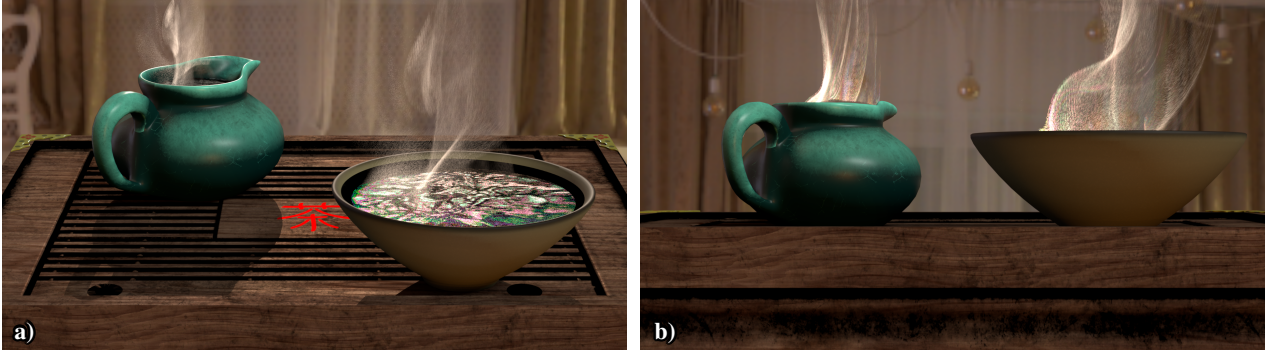
Figure 13: The figure contains two frames of our animation showcasing iridescent levitating drops (Figure a) and iridescent steam (Figure b). This scene includes an environmental light and a directional light. The animation features changes in lighting and viewing directions. We observe Quetelet scattering patterns on the water surface in the bowl, and the iridescent pattern changes as the angle changes. In the second part of the animation, we see color patterns in the steam that correlate with the steam flow. In Figure b), we see colors in the steam both above the bowl and the pitcher.
