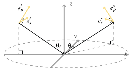
Figure 5: This figure illustrates the polarization coordinates for the incident wave and the outgoing wave. The incoming wave is decomposed into the parallel ( p ) polarized direction \mathbf{e}_p^i and the perpendicular ( s ) polarized direction \mathbf{e}_s^i . The outgoing wave field is decomposed into the parallel ( p ) polarized direction \mathbf{e}_p^s and the perpendicular ( s ) polarized direction \mathbf{e}_s^s .
