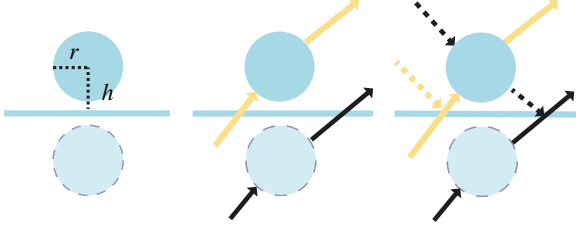
Figure 7: The bi-sphere model can be considered as introducing an imaginary sphere with reflection symmetry to the original sphere across the water surface (left figure). Adding Mie scattering from the two spheres (middle figure) computes the interference between path type II and type III in the first-order paths (right figure).
