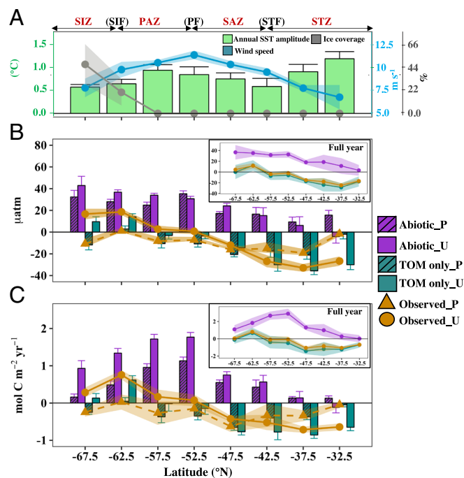
Fig. 3. Influence of biology on air-sea \text{CO}_2 exchange in the SO. Meridional pattern of (A) seasonal SST range, annual average wind speed, and percentage sea ice cover; (B) average sea-air p\text{CO}_2 difference ( \Delta p\text{CO}_2 = p\text{CO}_{2\text{ sea}} - p\text{CO}_{2\text{ air}} ); and (C) cumulative \text{CO}_2 flux over the productive (P) and unproductive (U) seasons for the different productivity scenarios, with annual results shown in subpanels. The shading and error bars reflect the propagated uncertainty. Frontal zones as described in Fig. 1. Positive values in B and C indicate a source of \text{CO}_2 to the atmosphere. Abiotic: reconstructed, abiotic ocean; TOM only: reconstructed ocean with only total organic carbon production; Observed: observed, biotic ocean including both TOM and PIC production.
