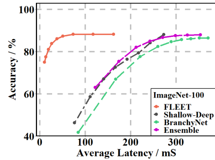
Figure 7: Latency of FLEET vs local early-exit.
