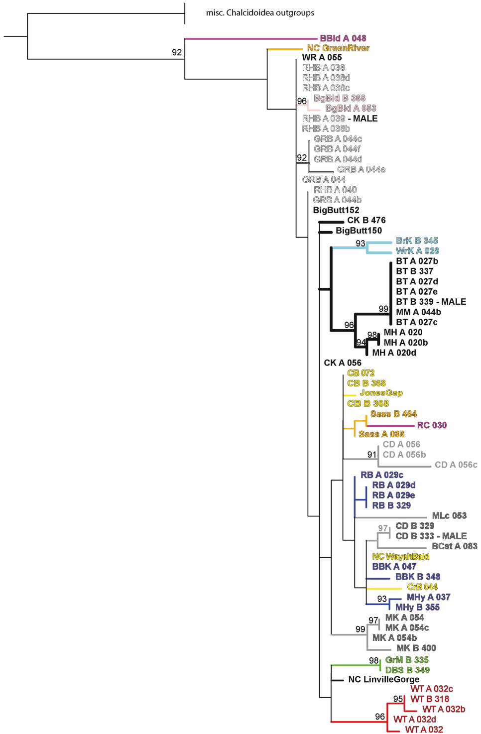
Figure 2. Maximum likelihood phylogeny of Dipara trilineata individuals, with locality abbreviations as in Suppl. material 1, and colors of OTUs keyed to localities shown in Fig. 1.
