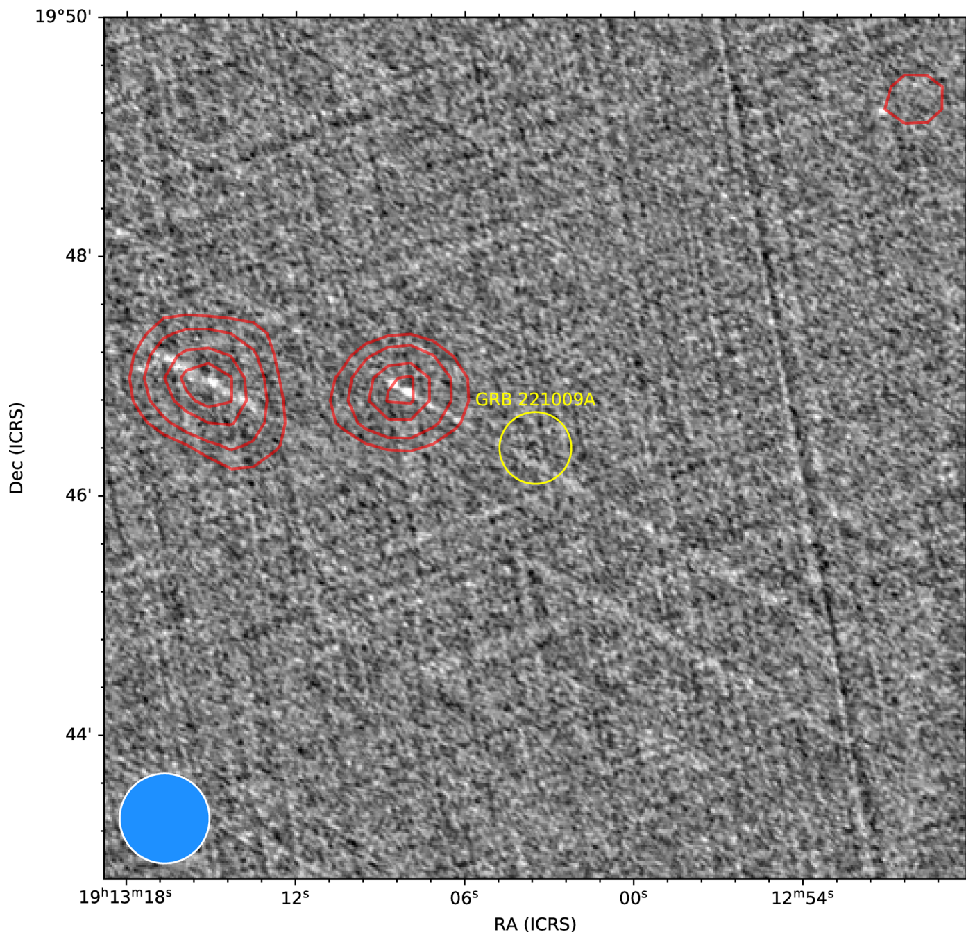
Extended Data Fig. 1 | Very Large Array Sky Survey archival observations of the field of GRB 221009A. The Very Large Array Sky Survey (VLASS; version 2.2; [86]) observation of the field of GRB 221009A, with National Radio Astronomy Observatory Very Large Array Sky Survey (NVSS; [87]) contours overlaid in red. The restoring beam for the NVSS image is shown as a blue circle in the bottom left of the image, the restoring beam for VLASS is significantly smaller and is not shown, but has a major and minor axis of 3.31'' and 2.29'' , respectively, at a position angle of 51.04^\circ . The yellow circle is centred on the position of GRB
