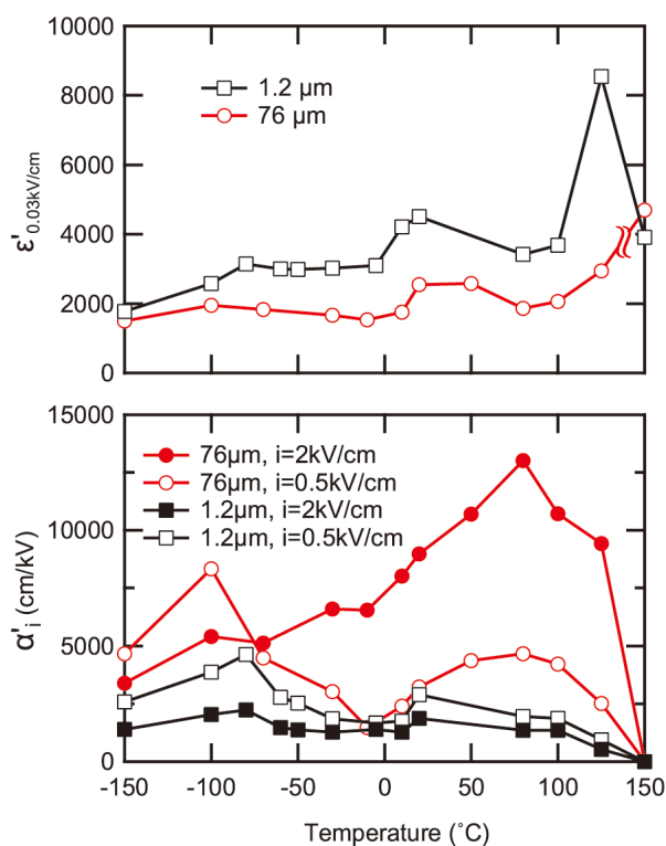
Figure 6. Temperature dependence of the pseudo-Rayleigh parameters of the BaTiO 3 ceramics with grain sizes of 1.2 \mu\text{m} and 76 \mu\text{m} .
