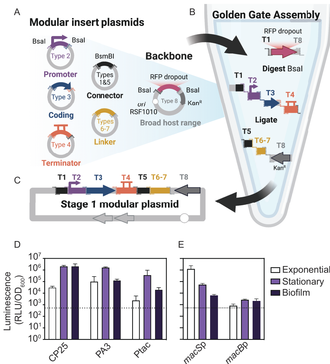
FIG 1 Schematic overview of the modular plasmid system and quantitative promoter measurements. (A) Schematic representation of the modular golden gate assembly plasmid parts with flanking Bsal cut sites (dashed lines). Overlapping 4 bp overhangs are color coordinated. The modular broad-host-range (BHR) backbone (pBTK402) contains inverted Bsal cut sites and an RFP dropout. (B) Golden Gate Assembly is performed in a one-tube reaction by digesting the backbone and insert part plasmids with Bsal and ligating with T4 ligase. (C) A modular stage-1 plasmid is complete when all overlapping inserts are successfully assembled in order. (D and E) Luciferase assays of P. luteoviolacea strains expressing plasmids with different promoters during exponential, stationary, or biofilm growth driving a Nanoluciferase ( NLuc ) gene where (D) shows CP25- NLuc -T7, PA3- NLuc -T7, Ptac- NLuc -T7 and (E) compares native MACs macS and macB promoters. Luminescence, as relative luminescence units (RLUs), is normalized to optical density at 600 nm (OD 600 ) and plotted on a log base 10 scale. The dashed line indicates P. luteoviolacea cells expressing a non-luminescent plasmid as represented by the dotted line ( Y = 524 \text{ RLU/OD}_{600} ). Plotted is the mean of three biological replicates. Error bars indicate standard deviations.
