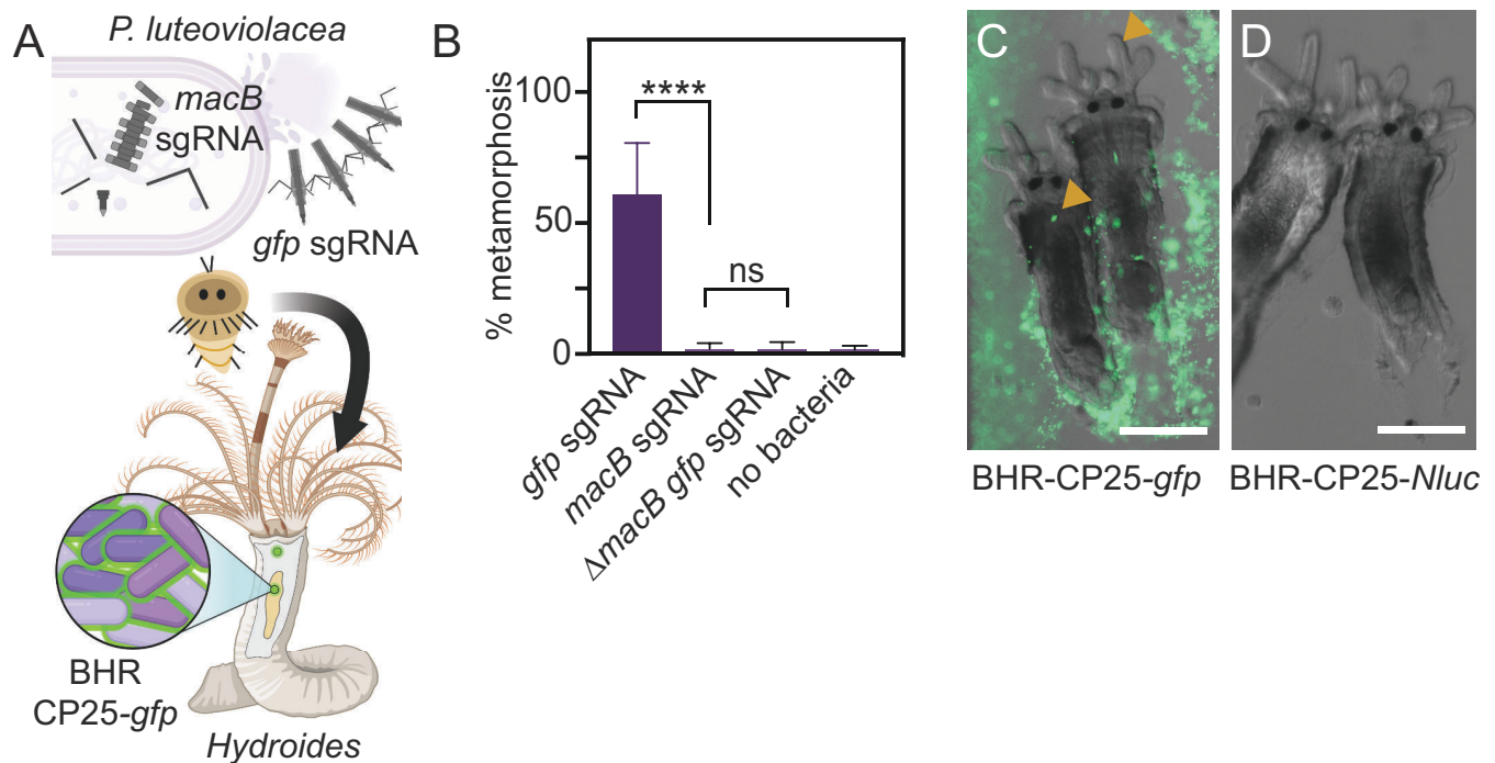
FIG 3 Functional knockdown of MACs and visualization of P. luteoviolacea during the tubeworm-microbe interaction. (A) Schematic depicting P. luteoviolacea and the production of MACs, which induce tubeworm metamorphosis. CRISPRi single-guide RNA (sgRNA) targeting the macB MACs baseplate gene prevents MACs from assembling, rendering the bacterium unable to induce metamorphosis. Cells that produce intact MACs are able to induce tubeworm metamorphosis. A strong fluorescent reporter strain (BHR-CP25- gfp ) enabled visualization of live tubeworm-bacteria interactions. (B) Bar graph representing biofilm metamorphosis assays with P. luteoviolacea carrying a CRISPRi plasmid targeting macB or gfp and Hydroides tubeworms. A P. luteoviolacea \Delta macB strain with a sgRNA targeting gfp and a treatment without bacteria (no bacteria) were included as controls. Biofilm concentrations were made with cells at OD 600 0.1. Bars plotted show the average of 12 replicates, performed across three independent experiments. Each well contained 20–40 worms. Error bars indicate standard deviations. Statistical significance between treatments was determined by Dunn's multiple comparisons test ( N = 12 ). (C and D) Merged fluorescence and DIC micrographs of Hydroides elegans juveniles imaged 24 h after the competent larvae were exposed to inductive biofilms of P. luteoviolacea containing plasmids with (C) CP25- gfp or (D) CP25- Nluc . Strains containing Nluc plasmids were used as a negative control to account for autofluorescence. Yellow arrows show accumulation of fluorescent bacteria in the Hydroides juvenile pharynx. Scale bar is 100 \mu m.
