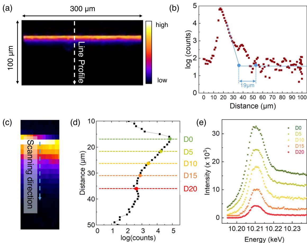
Figure 4. (a) Representative XFM image of spray-calcined WO 3 film on a fluorine-doped tin oxide (FTO) substrate and immersed in a 0.5 M sulfuric acid (H 2 SO 4 ) electrolyte. The image dimension is 300 μm × 100 μm and the size of each pixel is 1 × 1 μm 2 . (b) With the XFM line profile, log (counts) is a function of the distance shown in (a). The auxiliary lines (in blue) are drawn to estimate the thickness of the diffusion layer in the WO 3 -H 2 SO 4 electrochemical cell. (c) The enlarged XFM image highlights the X-ray scanning direction during the collection of μ-XANES data. (d) The corresponding μ-XANES data collection positions, where D0 represents the brightest starting point, and D5 to D20 represent the subsequent μ-XANES data collection positions, with an interval of 5 μm. (e) Experimental μ-XANES spectra at the W L 3 -edge. The spectra are collected when the potential of the WO 3 electrode is held at −0.1 V vs Ag/AgCl. The white arrow in (a) indicates the direction of the presented line profile.
