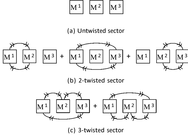
Figure 2. A cartoon of the sectors of the symmetric orbifold theory \mathcal{M}_3 = \mathcal{M}^{\otimes 3}/S_3 . Each box is a copy of the seed theory. Boxes connected by arrows are identified with one another (i.e. “glued”), and any remaining boxes are just factors in the symmetric product. The untwisted sector (a) is simply the symmetrized product space. The 2-twisted sector (b) is constructed by gluing together any two seed copies and symmetrizing. The 3-twisted sector (c) arises from gluing together three copies in any order and symmetrizing.
