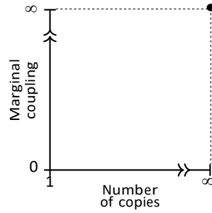
Figure 3. The parameter space of the symmetric orbifold of T^4 . We can dial both the number of seed copies and the marginal coupling which makes the copies interact. The bottom axis (with coupling = 0) describes the orbifold point. The black point is the holographic limit at which the description by type IIB supergravity on Janus is valid.
