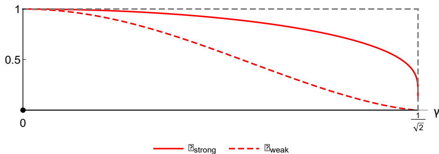
Figure 6. The transmission coefficients as functions of the Janus parameter \gamma \in [0, \frac{1}{\sqrt{2}}] both at strong coupling (solid) and at weak coupling (dashed). While they match at the extremal values of \gamma , the values at strong coupling are consistently larger than those at weak coupling. Furthermore, the weak-coupling coefficient has an inflection point at \gamma \approx 0.406 , whereas the strong-coupling coefficient has a strictly negative derivative.
