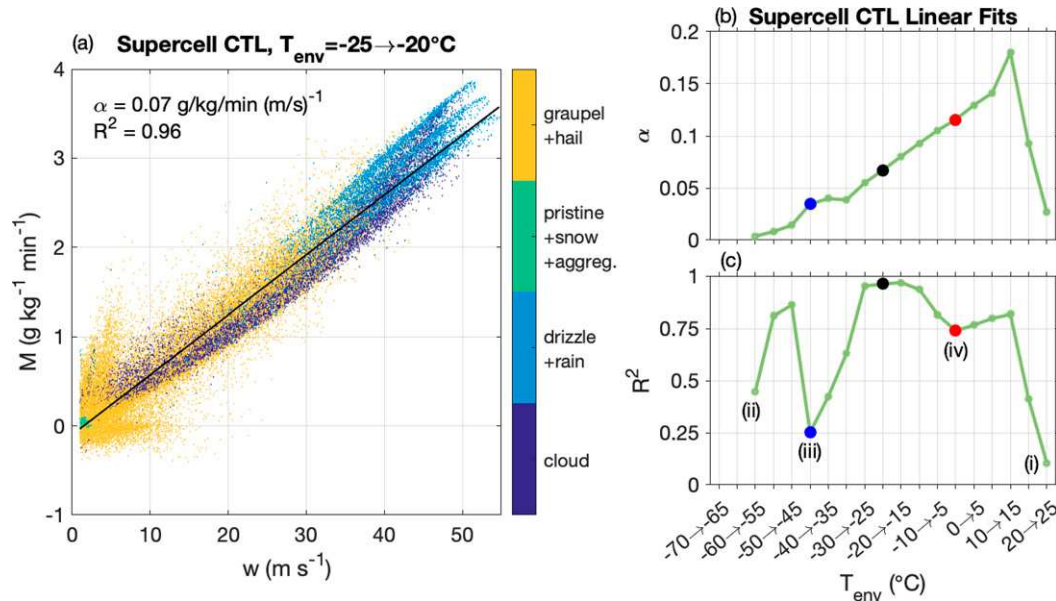
FIG. 2. (a) Scatterplot of w vs M for the Supercell CTL case. Results are shown for w > 1 m s -1 and environmental temperatures between -25^{\circ} and -20^{\circ} C every 5 simulation minutes. Color shading indicates the hydrometeor type with the largest mixing ratio in each grid box at the end of the 1-min interval. Only every tenth grid point is plotted. The black line shows a linear regression fit; values of the slope of the linear fit ( \alpha ) and R^2 are listed in the top left of the panel. (b) Slope of the linear fit and (c) R^2 of the linear fit for environmental temperatures every 5^{\circ} C for the Supercell CTL case. Units in (b) are g kg -1 min -1 (m s -1 ) -1 . Black dots in (b) and (c) highlight the slope and R^2 for the fit shown in (a), while blue and red dots in (b) and (c) highlight the slope and R^2 for the fits shown in Figs. 3 and 4, respectively. Labeled points (i)–(iv) in (c) are discussed in the text. Note that (b) and (c) share the same x axis.
