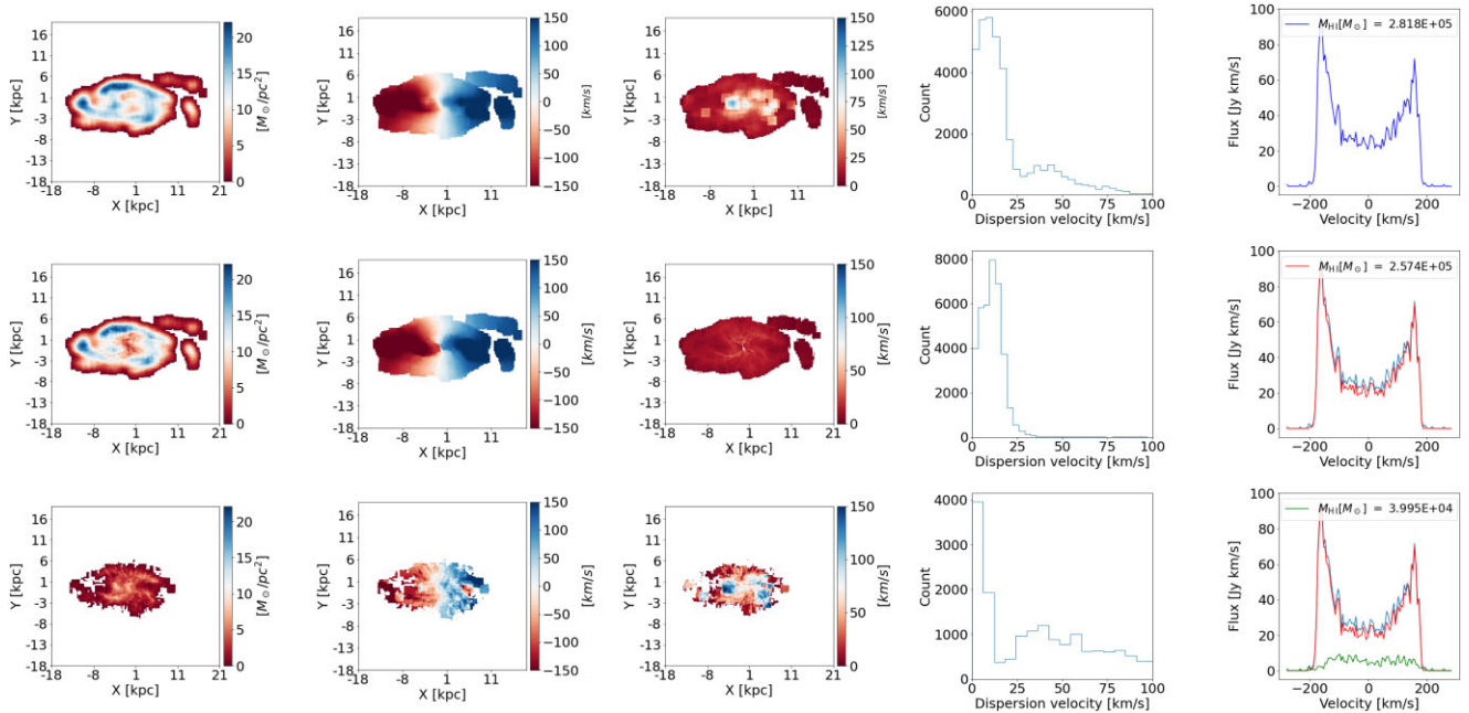
Figure 4. Dissection of H I in a galaxy from the simulation at z = 0 . The first through third columns represent the moment 0, 1, and 2 maps, respectively, and the fourth and fifth columns show the distributions of velocity dispersion and the H I profiles. The first row shows the original simulated data cube, while the second and third rows show the regular and anomalous gas, respectively.
