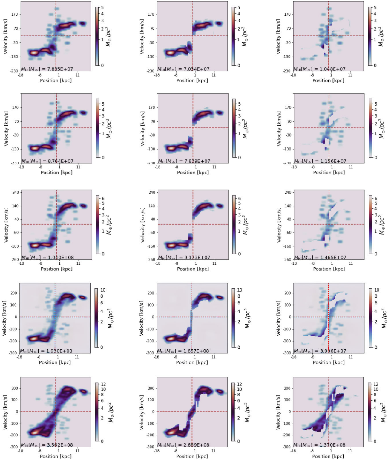
Figure 8. P–V plots of the galaxy shown in Fig. 2 at different inclination angles. Each row shows the P–V slice of the galaxy inclined at 30°, 40°, 50°, 70°, and 80°, respectively, from top to bottom. The first column comes from the full cube, while the second and third P–V slices are for the extracted regular and anomalous emission. The value shown on the upper left of each panel in the first column indicates the fraction of kinematically anomalous gas present in that slice. Values at the bottom indicate the total H I mass present in the respective P–V slices.
