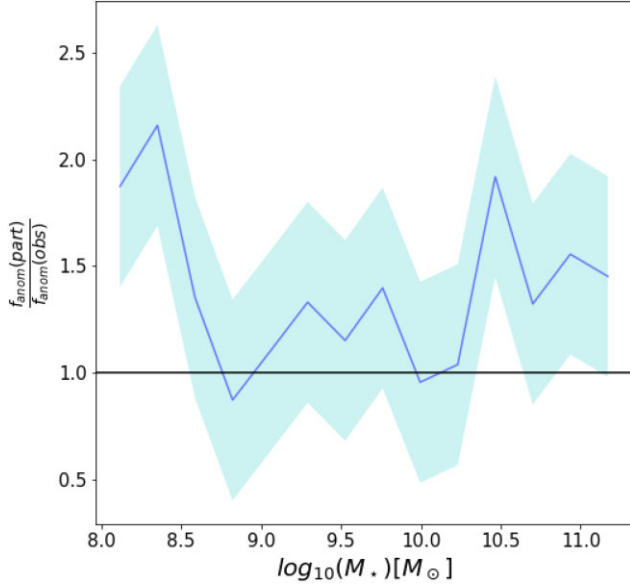
Figure 7. Ratio of the particle-based anomalous gas fraction to the cube-based ('observational') anomalous gas fraction as a function of stellar mass. The blue curve and cyan area represent the median and interquartile range of this ratio; the black line marks a ratio of unity.
