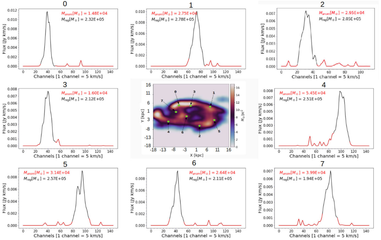
Figure 3. H I moment 0 map of a galaxy from the simulation (centre panel) alongside line profiles extracted at the positions numbered on the H I map. The red lines in the profiles denote the emission from the galaxy's anomalous gas, while the black lines represent regular emission.
