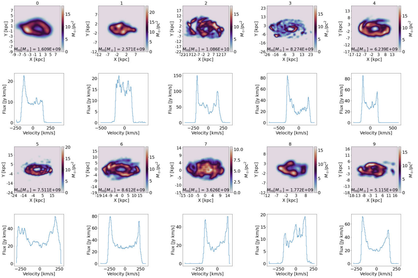
Figure 10. Plots of the H I moment 0 maps and profiles of the ten galaxies (numbered from 0 to 9) used to produce Fig. 9.
