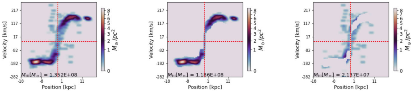
Figure 2. P–V plots of a galaxy from the simulation. The x- and y-axis values are subtracted by the position of the centre of mass of the galaxy and its systemic velocity, respectively. The left-hand panel shows the P–V diagram for the full cube containing all of the galaxy’s H I emission. The black circles indicate some of the most conspicuous examples of kinematically anomalous material, which is the sort of gas that our decomposition method has been designed to identify and extract. The middle panel shows the gas that comes from the main disc of the galaxy; the right-hand panel shows the anomalous gas that has been extracted from the original cube. Values at the bottom indicate the total H I mass present in the respective P–V slices. The vertical and horizontal red dashed lines represent the position and velocity of the centre of mass the galaxy.
