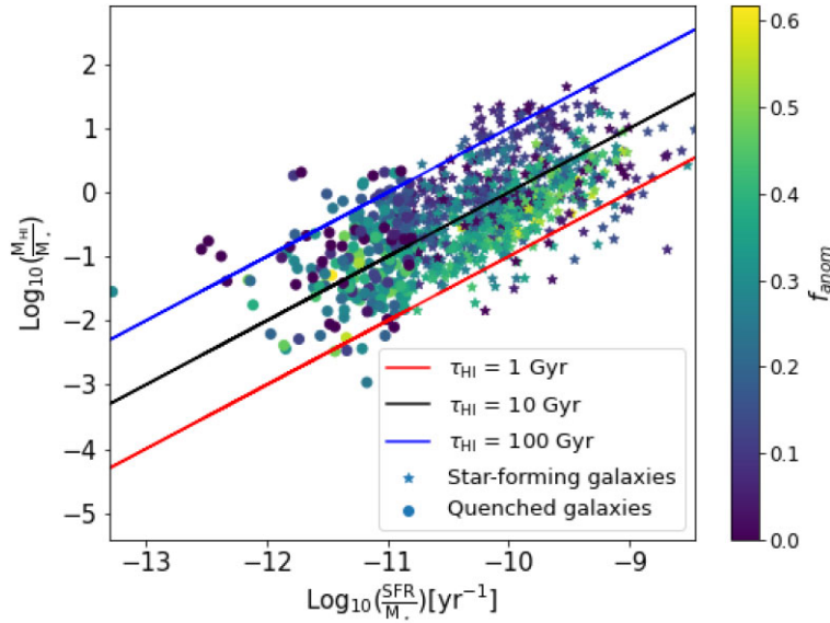
Figure 11. Dependence of specific star formation rate on H I gas fraction colour-coded by the anomalous gas mass fraction. Star-forming galaxies are represented by star symbols, while quenched galaxies are represented by dot symbols. The three lines indicate atomic gas depletion times of 1, 10, and 100 Gyr (red, black, and blue respectively).
