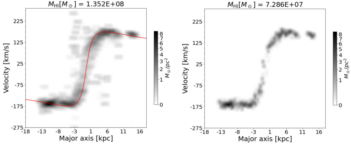
Figure 6. Left: P–V diagram for the galaxy shown in Fig. 5. The red line is the expected rotation curve that comes from the best-fit rotation curve plotted in Fig. 5. The value on top is the total mass of H I gas present in this slice. Right: P–V diagram for the regularly rotating gas after removal of anomalous material using the particle-based decomposition method.
