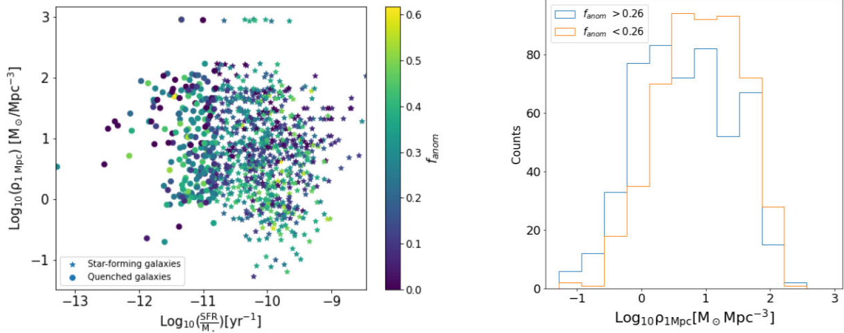
Figure 12. Left: Mean stellar mass density in a sphere of radius 1Mpc ( \log(\rho_{1\text{Mpc}}) ) vs. specific star formation rate, colour-coded by the anomalous gas fraction. Star-forming galaxies are represented by star symbols, while quenched galaxies are represented by dot symbols. Right: Distribution of the environmental density for galaxies with high and low anomalous gas fractions, represented by the orange and blue curves respectively.
