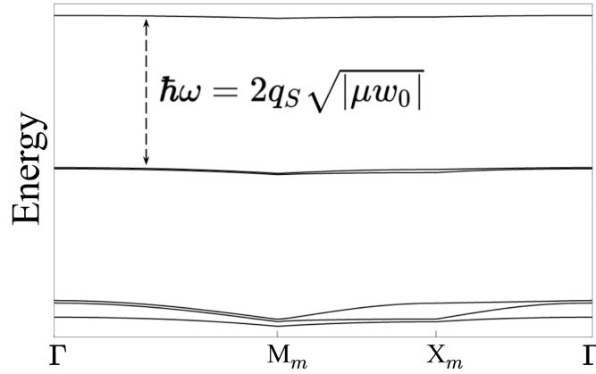
Figure 4: Energy of the bands in the tight-binding limit, which occurs deep in the trivial phase of Fig 2a. The degeneracy structure approaches: 1, 2, 3, ..., n , ... for the n^{\text{th}} set of bands.
