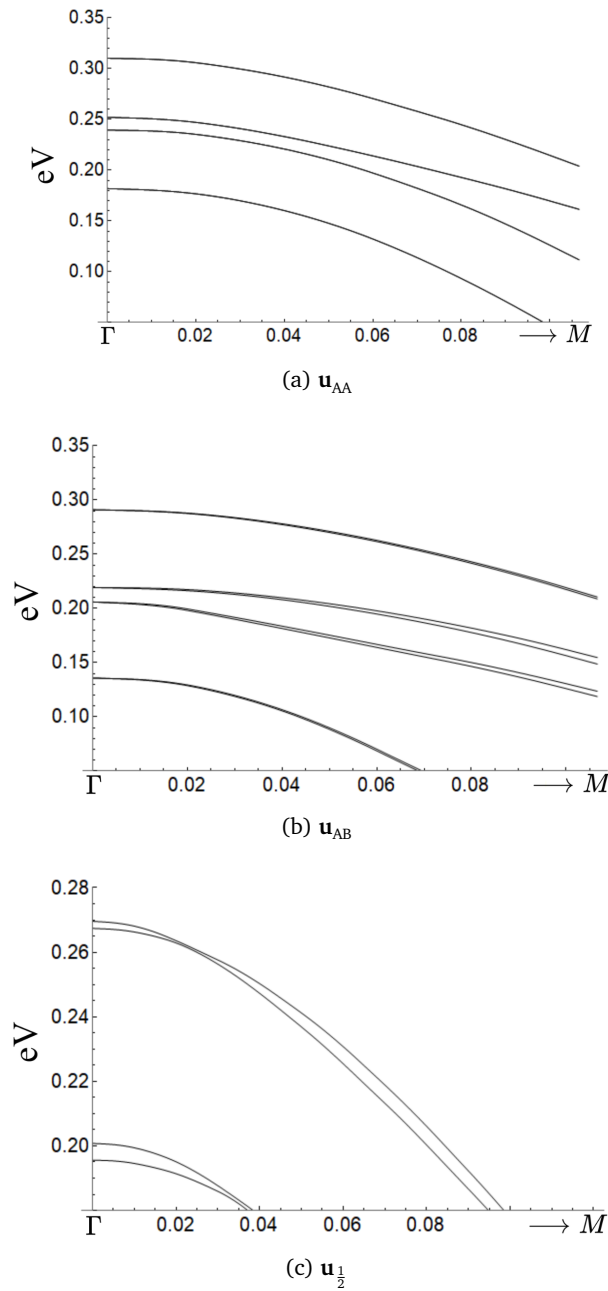
Figure 11: Bands near \Gamma for the (a) AA stacked, (b) AB stacked, and \mathbf{u}_{\frac{1}{2}} = (\frac{l_{Fe}}{2}, 0) stacking. The momenta are given in units of \frac{2\pi}{l_{Fe}} . The band energies at \Gamma are reported as follows: \{E_{AA,+,+\lambda}, E_{AA,-,+\lambda}, E_{AA,+,-\lambda}, E_{AA,-,-\lambda}\} = \{310.3, 252.9, 238.5, 181.0\} meV, \{E_{AB,+,+\lambda}, E_{AB,-,+\lambda}, E_{AB,+,-\lambda}, E_{AB,-,-\lambda}\} = \{290.2, 218.4, 204.0, 135.1\} meV, and \{E_{\frac{1}{2},+,+}, E_{\frac{1}{2},+,-}, E_{\frac{1}{2},-,+}, E_{\frac{1}{2},-,-}\} = \{269.5, 267.5, 200.8, 195.7\} meV.
