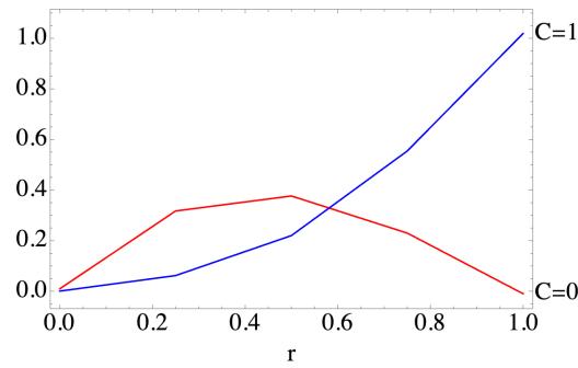
Figure 6: The integrated Berry curvature as a function of the fraction of the total mBZ for the two phases. The bounds of the integrated fraction is defined within a square with side length r q_S , where r \in \{0, \frac{1}{4}, \frac{1}{2}, \frac{3}{4}, 1\} , centered at \Gamma . As r approaches 1, the integrated Berry curvature approaches C [98].
