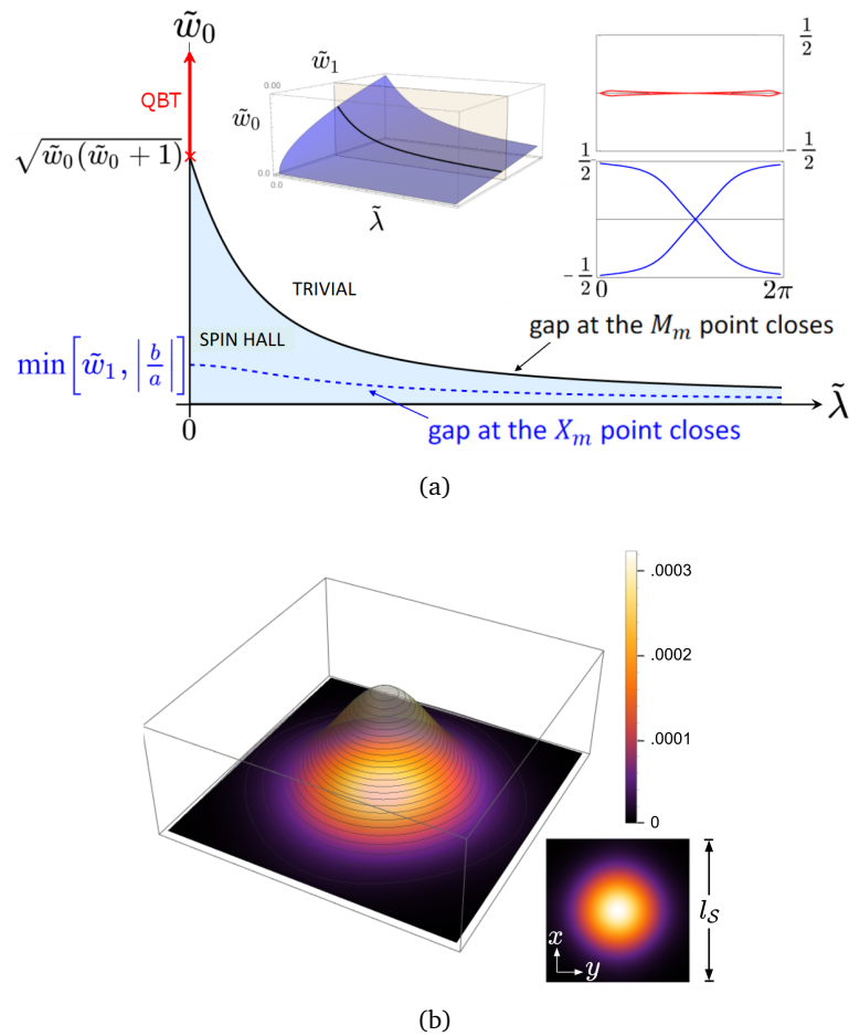
Figure 2: (a) Phase diagram for the upper moire hole band at fixed \tilde{w}_1 . The boundary between the spin Hall and trivial phase corresponds to the black line in the 3D diagram (shown as inset). The charge center winding within the unit cell, as a function of mBZ momentum k_y \in \{0, 2\pi\} , is shown for the two phases. The quadratic-band touching at \Gamma is preserved along the \tilde{\lambda} = 0 line. The red \times indicates a triple-band touching at M_m , beyond which becomes a quadratic-band touching (shown as a red line). The diagram for \tilde{w}_0 < 0 is equivalent, except for the absence of the dashed blue line, because the gap at X_m does not close there. (b) Density of the Wannier state for the band in the trivial phase, calculated via the projection method [87].
