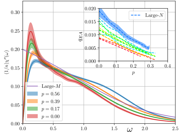
FIG. 11 (Shackleton et al. , 2021) Local spin response function for the spin-1/2 doped random exchange t - J model, as obtained by exact diagonalization of an N = 18 site cluster, averaged over 100 disorder realizations, for t = J = 1 . n = 1 - p is the particle density.
