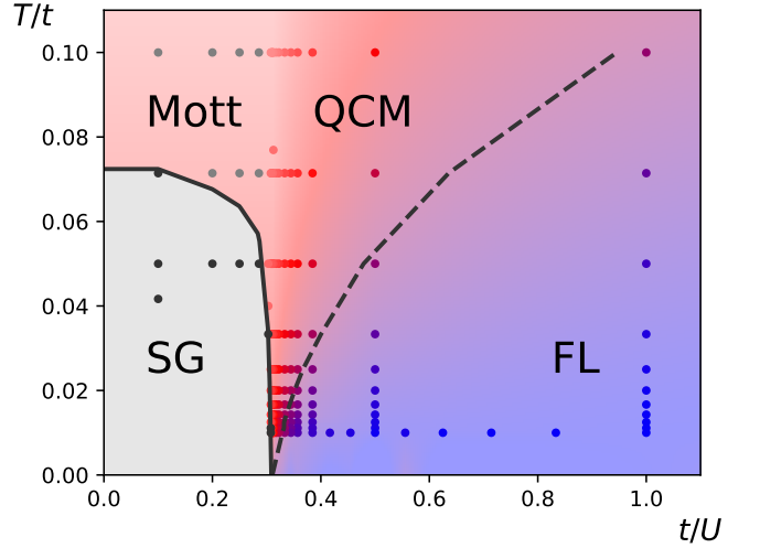
FIG. 12 Phase diagram of the spin-1/2 half-filled random exchange t - J - U model. At low temperature, a quantum critical point separates the spin glass phase (SG) from a Fermi liquid phase (FL). The background color corresponds to the fitted power-law exponent of the local spin correlation function \chi(\tau) \sim 1/\tau^{2\Delta} , with 2\Delta \simeq 1 in the quantum critical metal (QCM) (red), and \Delta = 1 in the Fermi liquid (blue). At high temperature and U , one obtains a Mott insulator. Reproduced from (Cha et al. , 2020b).
