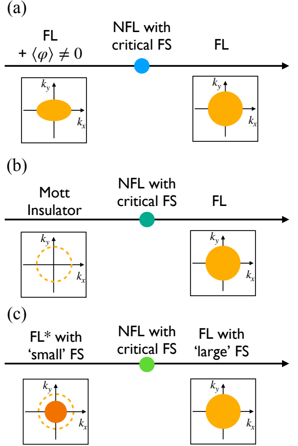
FIG. 1 (a) A nFL obtained by coupling a critical boson (e.g. nematic order with \mathbf{Q} = 0 ) to an electronic Fermi surface. (b) A bandwidth-tuned metal to paramagnetic Mott insulator transition. The Mott insulator hosts a neutral Fermi surface (dashed circle) of fractionalized degrees of freedom coupled to an emergent gauge field. (c) A Fermi volume changing transition between two distinct metals across a ‘Kondo-breakdown’ quantum critical point. The quantum critical point hosts a critical Fermi surface of electrons in all the examples. The Mott insulator and the FL* phases host a critical Fermi surface of ‘spinons’ in (b) and (c), respectively.
