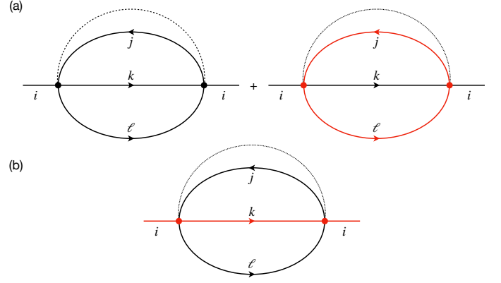
FIG. 22 The melon graphs for the model in Eq. (10.7a) for the electron self-energies for (a) c , and (b) d electrons, respectively. Solid black (red) lines denote fully dressed c ( d ) Green’s functions. The dashed (dotted) line represents the disorder averaging associated with the interaction vertices, \overline{|U_{ij; k\ell}|^2} ( \overline{|V_{ij; k\ell}|^2} ), respectively.
