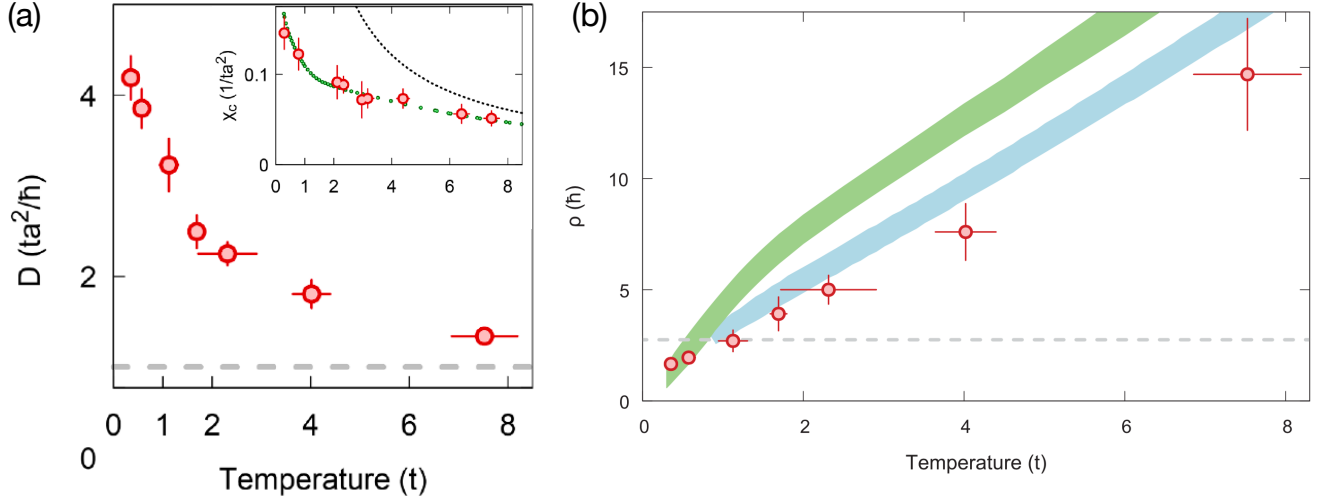
FIG. 2 Measurement of the diffusion constant (a) and compressibility ((a)-inset) for a gas of ultra-cold ^6\text{Li} atoms in an optical lattice, realizing a two-dimensional Fermi-Hubbard model with U/t \simeq 7.5 at a density n \simeq 0.825 . (b) Reconstructed ‘resistivity’ using Einstein-Sutherland relation. Grey horizontal dashed line represents the estimated MIR value. Theoretical calculations are shown in (a) and (b) as shaded regions.
