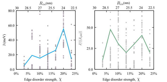
FIG. 3. Enhancing SYK interactions through edge disorder \chi . (a) SYK coupling strength J , (b) dimensionless ratio J/|\langle J_{ijkl} \rangle| as a function of edge disorder scale \chi for the medium size flake at B = 20 \text{ T} (approx. 100 000 atoms, 60 nm in diameter). Solid lines correspond to the average over up to 20 disorder realizations (marked with grey points, some outside of plot range).
