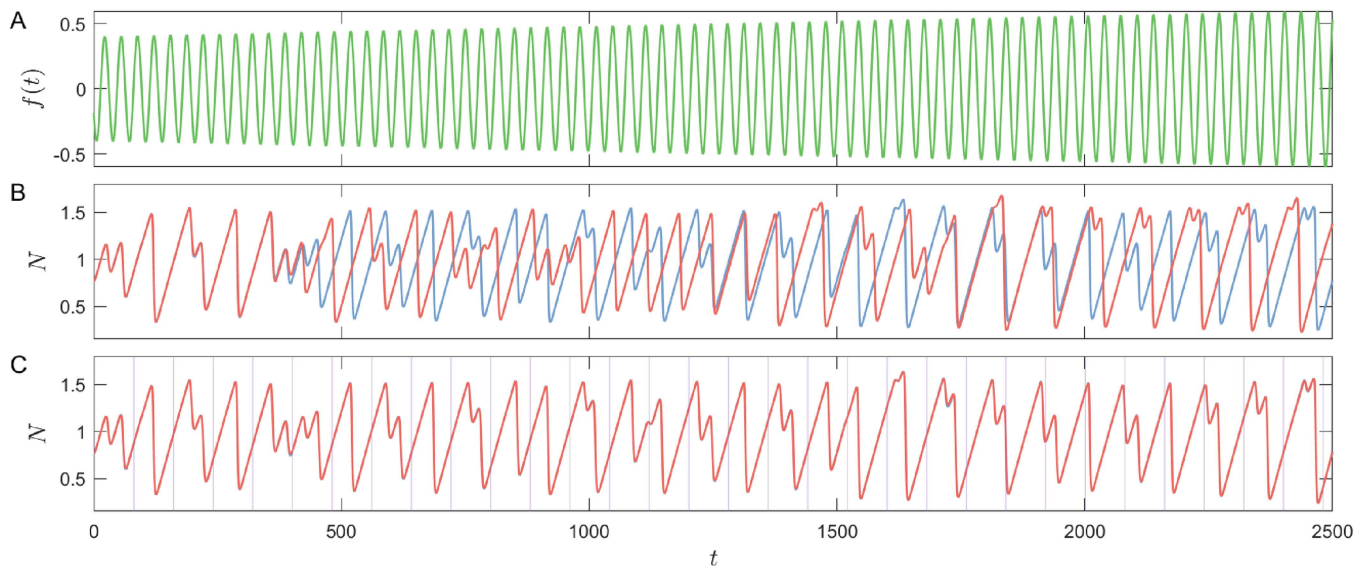
FIG. 9. Continual forecasting of the chaotic ecological system under non-stationary external driving f(t) and with sparse updates of the dynamical variables. (a) A nonstationary sinusoidal driving signal f(t) whose amplitude increases with time. The task for the digital twin is to forecast the response of the chaotic target system under this driving signal for a relatively long term. (b) The trajectory generated by the digital twin (red) in comparison with the true trajectory (blue). For t \in [0, 400] , the two trajectories match each other with small errors, but the digital twin generated trajectory begins to deviate from the true trajectory at t \sim 400 (due to chaos). (c) With only sparse updates from real data at times indicated by the vertical lines (2.5% of the time steps in the given time interval), the digital twin can make relatively accurate predictions for the long term, demonstrating the ability to perform continual forecasting.
