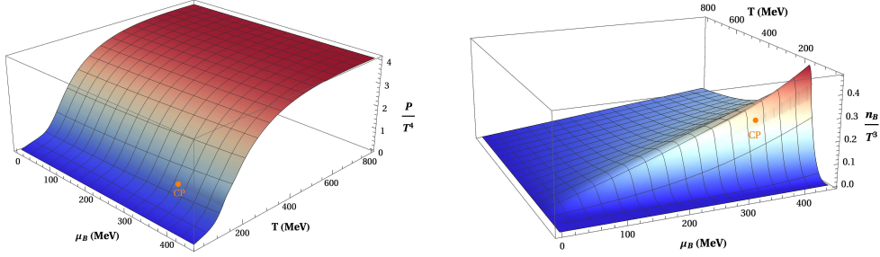
Figure 2: Left: The pressure for the choice of parameters as listed in Section 2. Right: The baryon density for the same choice of parameters.
