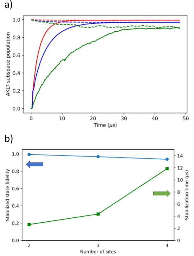
FIG. S6. Protocol performance with multiple qubits in the straddling regime. (a) The AKLT subspace population starting from the qutrits’ ground state |g \dots g\rangle (solid colored lines) and starting within the AKLT subspace (dashed colored lines), we simulate the time evolution of the AKLT chain with open boundary conditions subspace population under the driven dissipative protocol with a varying number of qutrits, N_{\text{sites}} = 2 (red), N_{\text{sites}} = 3 (blue) and N_{\text{sites}} = 4 (green) for comparison. (b) Extracted fitting parameters as the final fidelity and the convergence time with the same method as in Fig. 4 (b) on the total population in the AKLT subspace. The blue dots represent the varied final fidelity with systems of two, three, and four qutrits (left axis), and the green dots represent the convergence time for the protocol (right axis).
