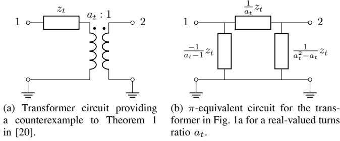
Fig. 1. Transformer circuits.
