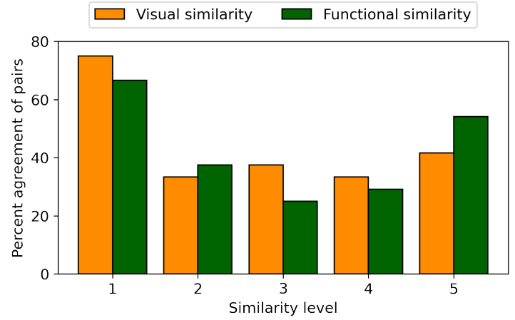
FIGURE 7: PERCENT AGREEMENT OF PAIRS ACCORDING TO HUMAN AND AI-BASED VISUAL AND FUNCTIONAL SIMILARITIES ACROSS SIMILARITY LEVELS
