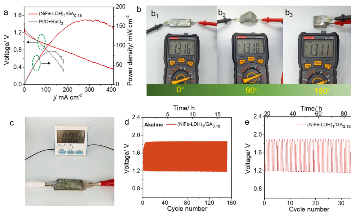
Fig. 9. (a) Discharge polarization and power density curves of (\text{NiFe-LDH})_1/\text{GA}_{0.18} and \text{Pt/C-RuO}_2 -based Zn-air batteries. (b) Photographs of Zn-air battery based on (\text{NiFe-LDH})_1/\text{GA}_{0.18} with OCPs measured with the battery before bending ( 0^\circ ) and after being bent to 90^\circ and 180^\circ . (c) Photos of an electronic clock powered by a (\text{NiFe-LDH})_1/\text{GA}_{0.18} based solid Zn-air battery. (d) Short-period charge-discharge curves (400 s per cycle for 150 cycles) and (e) long-period charge-discharge curves (2 h per cycle for 34 cycles) of the (\text{NiFe-LDH})_1/\text{GA}_{0.18} based solid Zn-air battery at 5 \text{ mA cm}^{-2} .
