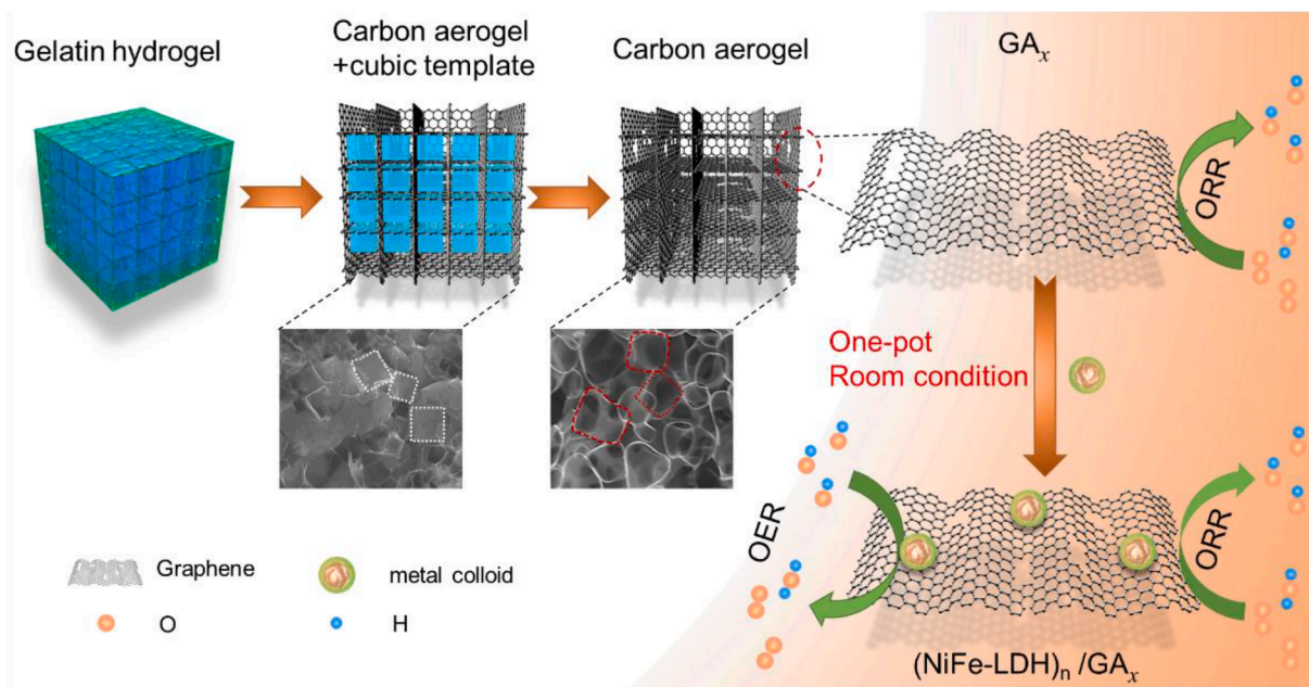
Scheme 1. Schematic illustration of the synthesis of ultrathin carbon aerogel (NiFe-LDH) n /GA x .
