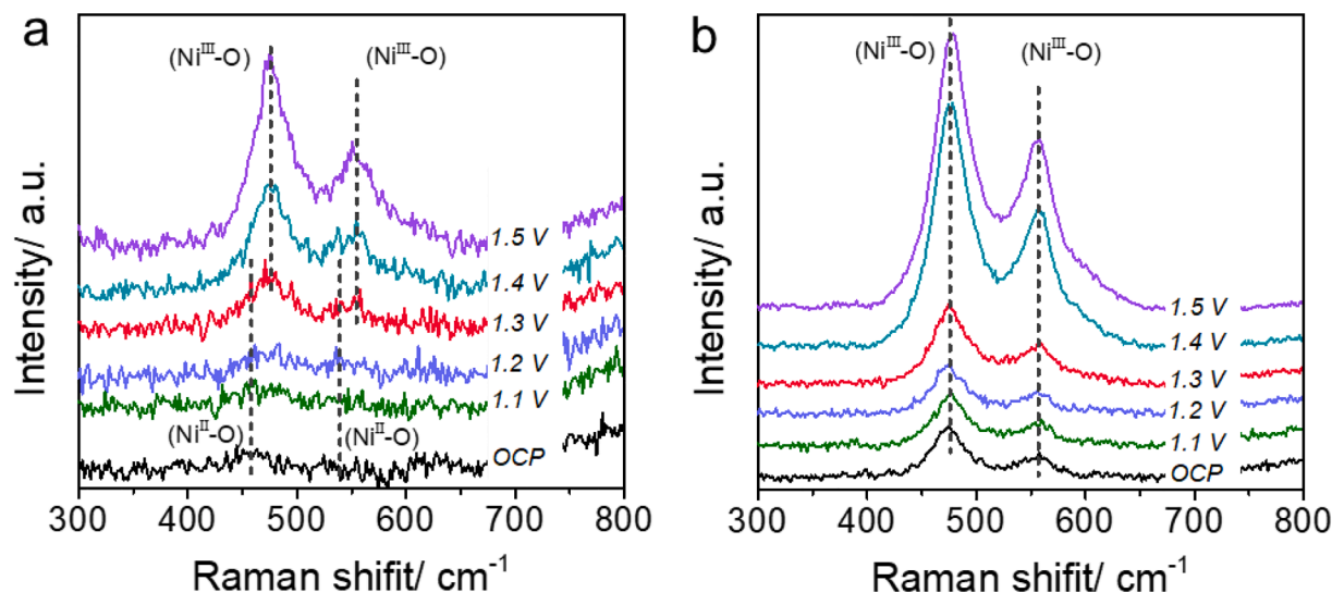
Fig. 6. Operando Raman spectra of the Ni-O vibrations in (a) \text{Ni}(\text{OH})_2 and (b) NiFe-LDH at different applied potentials.
