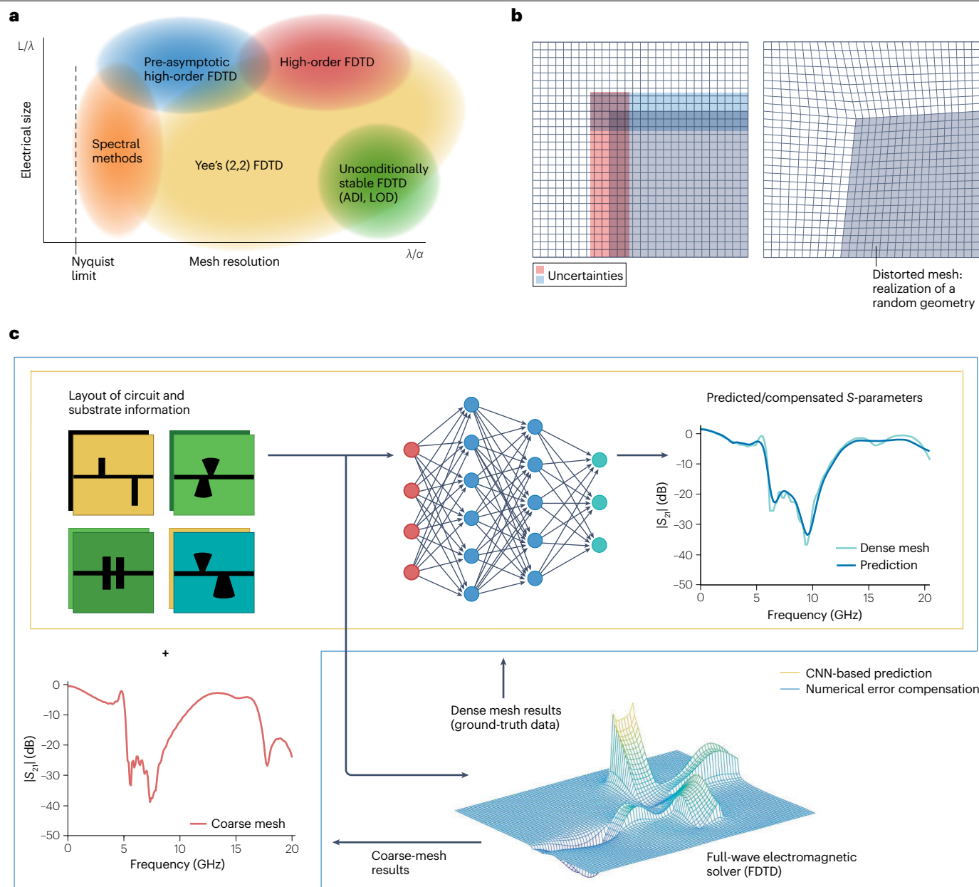
Fig. 2 | Advanced finite-difference time-domain modelling approaches.
