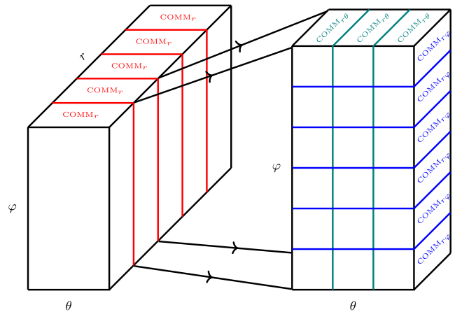
FIG. 1. Overview of the different MPI communicator groups. The global communicator is split along the r direction, and then each r group is split in two different subgroups. For one subgroup, the second splitting is in the \theta direction, while for the other, it is in the \varphi .
