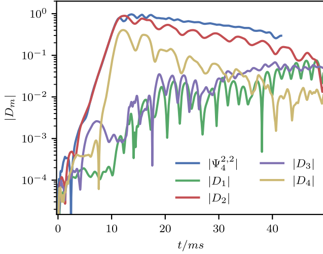
FIG. 13. Evolution of the first four nonaxisymmetric matter distribution modes and the (\ell = 2, m = 2) mode of \Psi_4 . As expected, the m = 2 mode of the density distribution is the dominant contribution to the waveform quadrupole mode.
