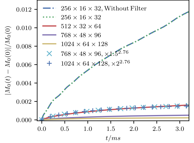
FIG. 9. Conservation of total rest mass for different resolutions. The plot shows relative change in the total mass of the NS for four different resolutions: h_0 ( 256 \times 16 \times 32 ), h_1 ( 512 \times 32 \times 64 ), h_2 ( 768 \times 48 \times 96 ), h_3 ( 1024 \times 64 \times 128 ). The crosses show the relative change in mass of the h_2 resolution run after rescaling by the ratio of the h_2 to h_1 resolution grid sizes to the power 2.76. The pluses show the same rescaled mass change, but for the h_3 case. Hence, the convergence order is between 2 and 3. The dashed and dotted curve are two h_0 resolution runs with and without filtering. They are on top of each other showing that the filter has no effect on the conservation of total rest mass.
