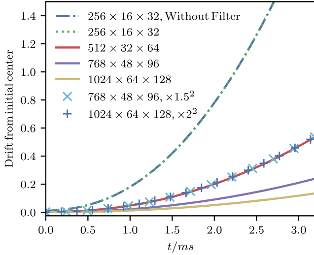
FIG. 8. Drift of the NS center of mass for different resolutions. The plot shows relative drift of the center of the NS for four different resolutions: h_0 ( 256 \times 16 \times 32 ), h_1 ( 512 \times 32 \times 64 ), h_2 ( 768 \times 48 \times 96 ), h_3 ( 1024 \times 64 \times 128 ). The crosses show the relative drift of the h_2 run after rescaling by the square of the ratio of the h_2 to h_1 resolution grid sizes. The pluses show the same rescaled drift but for the h_3 case. These rescaled drifts show clear second-order convergence. The dashed and dotted curve are two h_0 resolution runs with and without filtering. They are on top of each other showing that the filter has no effect on the drift of the NS.
