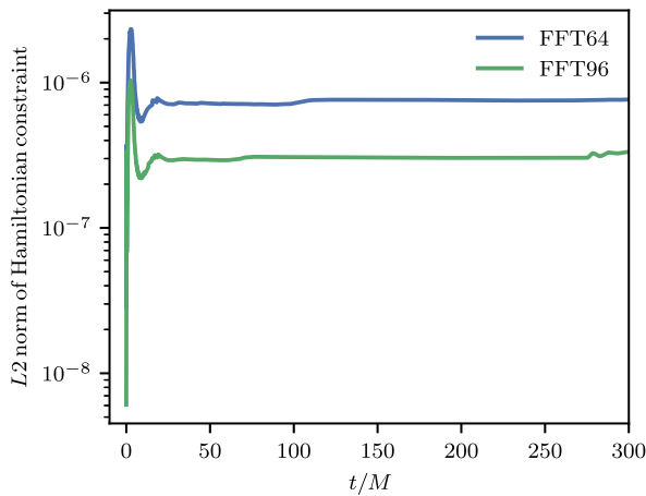
FIG. 3. The L^2 norm of the Hamiltonian constraints versus time at two resolutions FFT64 and FFT96. Here, the norm only includes points outside the horizon. The drop in constraint magnitude between FFT64 and FFT96 is consistent with a convergence order of 2.
