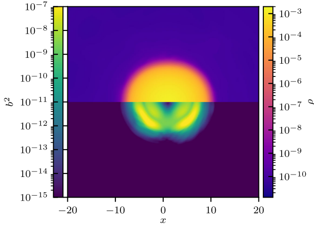
FIG. 11. \rho and b^2 evolution in x - z plane of y = 1 of model B2 at t = 3 ms.
