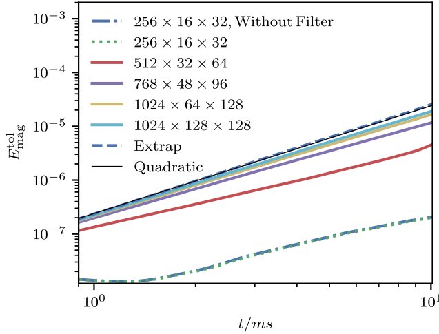
FIG. 14. The toroidal component of the magnetic energy E_{\text{mag}}^{\text{tor}} for early times and different resolutions. Prior to the formation of the instability, the magnitude of the E_{\text{mag}}^{\text{tor}} is expected to increase quadratically in time [129,138] (i.e., as t^2 ). The plot shows E_{\text{mag}}^{\text{tor}} for different resolutions and a Richardson extrapolations assuming second-order convergence, as well as quadratic curve y = ct^2 (chosen to match the initial behavior of the Richardson extrapolated curve). The lowest resolution run ( 256 \times 16 \times 32 ) was run with and without the filter. Since there is no visible difference in the toroidal magnetic energy growth when the filter is added or removed, this demonstrates that truncation error dominates over any errors introduced by the filter.
