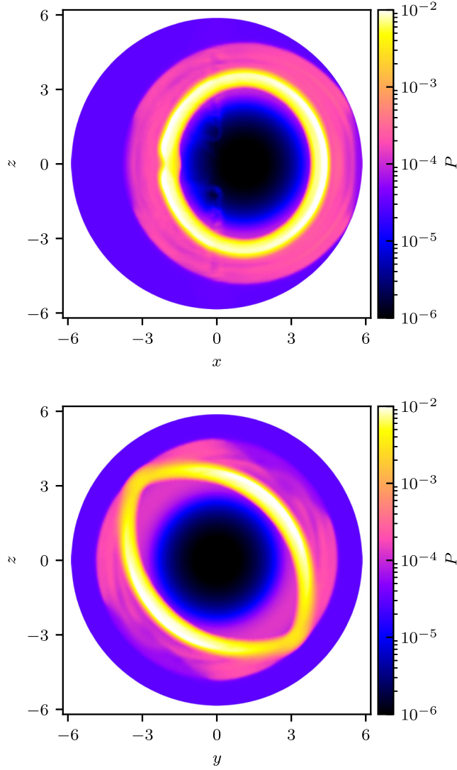
FIG. 7. Pressure in the x - z and y - z plane at t = 4 , with initial magnetic field B^z = 0.1 rotated by 45^\circ about x axis. The top panel shows the shock front along the xz plane ( y = 0 ), while the bottom shows the shock front on the plane x = 1.1 (note that the center of the explosion is at x = 1.1 ). The bottom panel show the x = 1.1 plane (the shock is centered along x = 1.1 ). The flow morphology is clearly seen to be tilted by 45^\circ .
