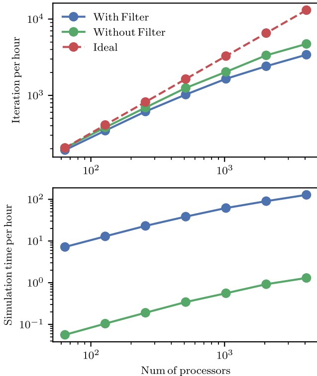
FIG. 2. Strong scaling of SphericalNR with the FFT filtering scheme. In the top plot, we show iterations per hour for both the code with and without the FFT filter. The code without the filter requires a time step 1/136 as small as with filtering. The bottom plot shows the actual performance in run time versus wall time.
