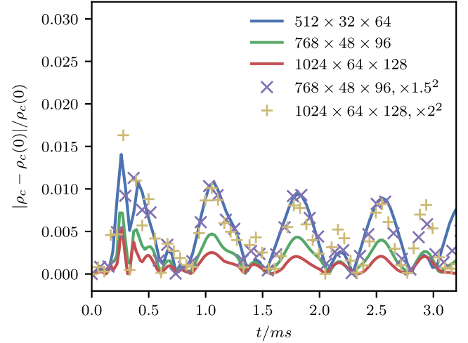
FIG. 10. Maximum density versus time for different resolutions. The plot shows relative change in the central density of the NS versus time for three different resolutions. The crosses show the relative change of the h_2 resolution run after rescaling by the square of the ratio of the h_2 to h_1 resolution grid sizes. The pluses show the same rescaled change, but for the h_3 resolution case. In regions where the relative change in the central density is large, second-order convergence is observed.
