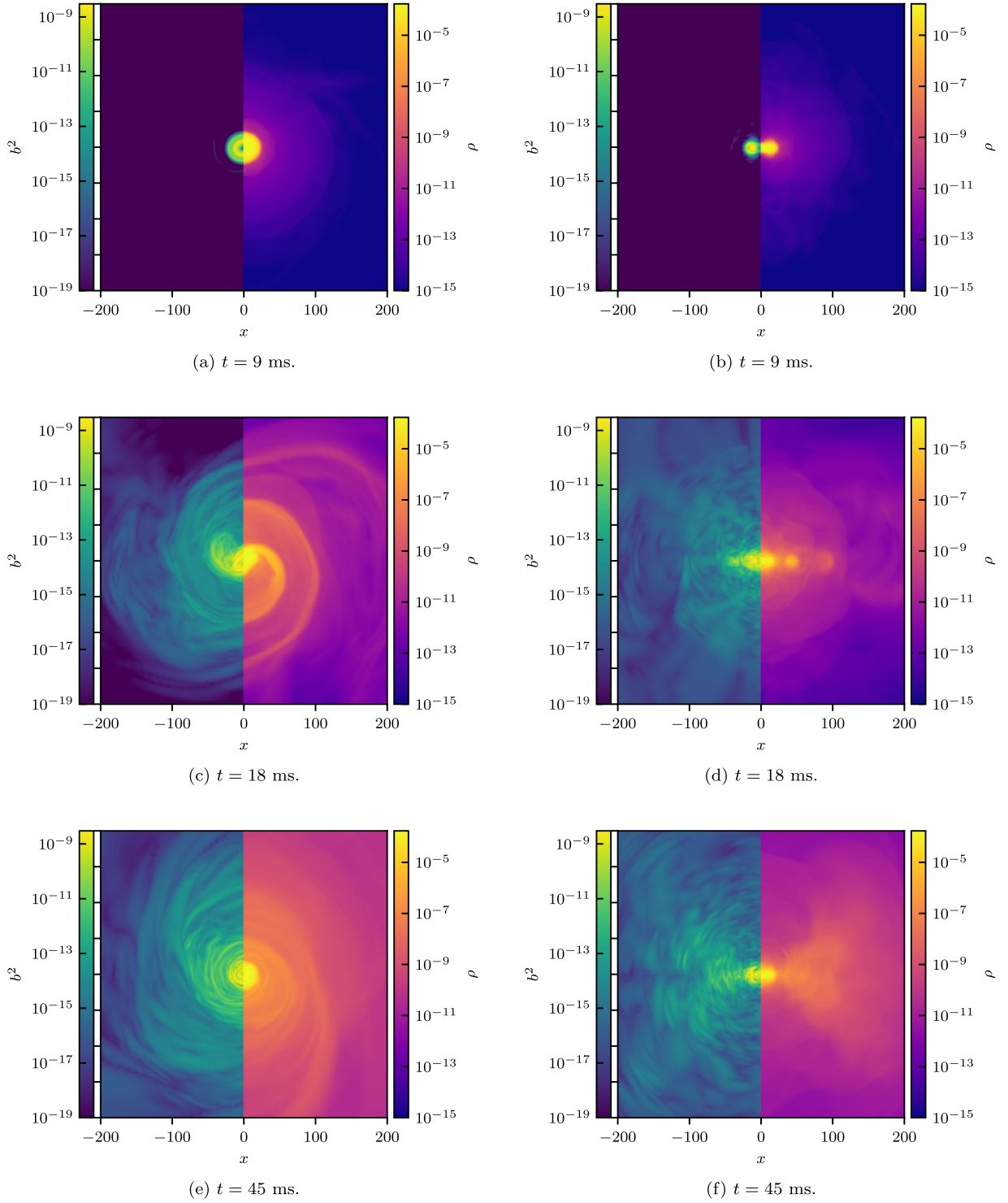
FIG. 12. Snapshots of b^2 and \rho on x - y (left column) and x - z (right column) plane of model U11 at t = 9 ms (top row), t = 18 ms (middle row), and t = 45 ms (bottom row).
