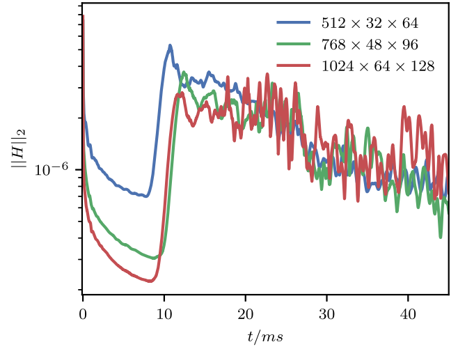
FIG. 15. The L^2 norm of the Hamiltonian constraint for the bar-mode-unstable star. Prior to the onset of the bar-mode instability, we see convergence (to zero) at 1.5 order. Note that, after the onset of the instability (which is seeded by random perturbations), the constraint violations remain small and do not exhibit exponential growth.
