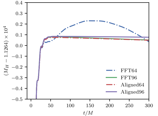
FIG. 5. A comparison of the irreducible mass of the BH versus time as measured by AHFinderDirect for n_\theta = 64 and n_\theta = 96 for the aligned case and using the double FFT filter. Here, mass conservation would imply that the irreducible mass settles to a constant value.
