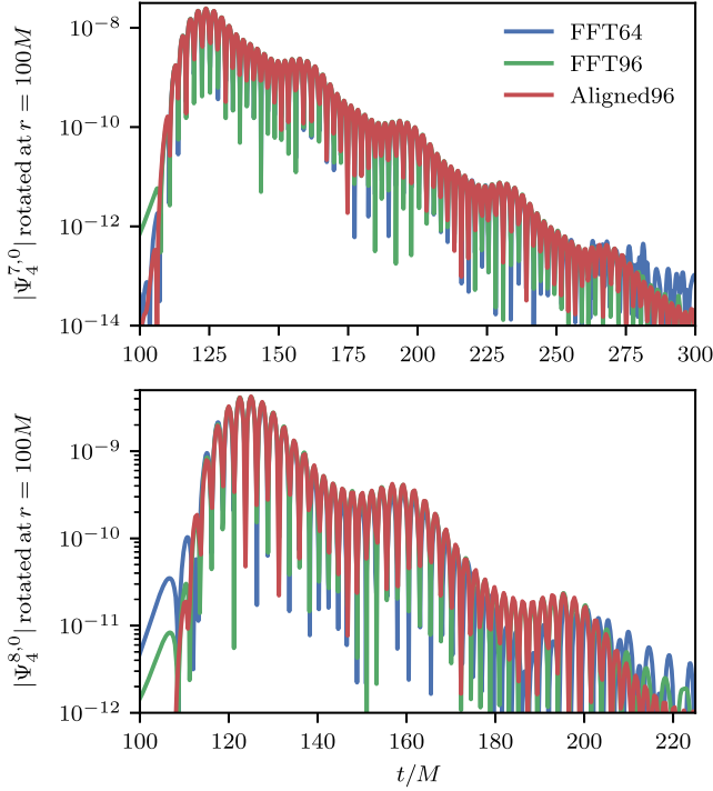
FIG. 6. A comparison of the \ell = 7 and \ell = 8 modes of \Psi_4 .
