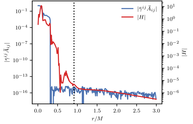
FIG. 4. Algebraic constraints (43) and Hamiltonian constraints along \theta = d\theta/2, \varphi = 0 at t = 150M for case FFT96. The vertical line indicates the radius of apparent horizon.
