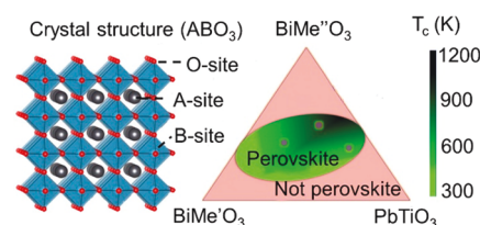
Figure 7. Thermal stability prediction of perovskite crystals with variable elements such as Mo, W, Nb, Ta, etc. and stoichiometric ratios using classification learning and regression. Reprinted with permission from ref 154. Copyright 2018 Springer Nature.
