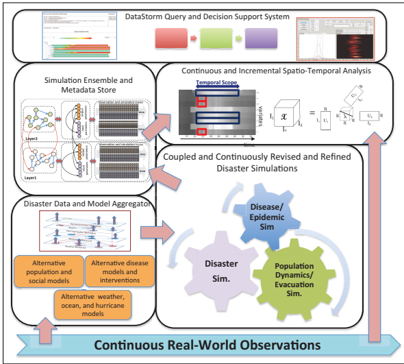
Figure 2: An overview of the DataStorm framework
