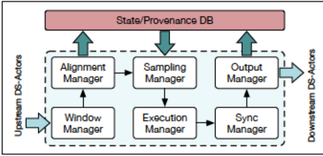
Figure 3: A DataStorm-FE actor (DS-actor), with individual sub-modules.
