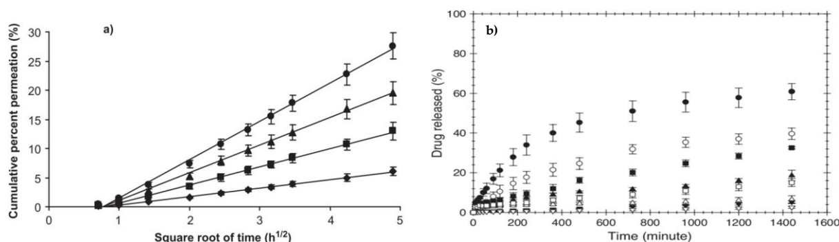
Figure 7. Effect of the molecular weight of a drug on (a) cumulative percent permeation (%), MX loading concentration at (◆) 2.5%, (■) 5%, (○) 10%, and (◊) 20 wt% of PVA (reprinted with permission from Taylor & Francis Online) and (b) the drug release (%) profile of (●) sodium salicylate, (○) diclofenac sodium, (△) indomethacin, and (■) naproxen drugs released from drug-loaded electrospun PVA mats (closed symbols) and as-cast PVA films (open symbols) by the transdermal diffusion through a pig skin method over a period of 0–1440 min (reprinted with permission from IOP Science) [51,52].
