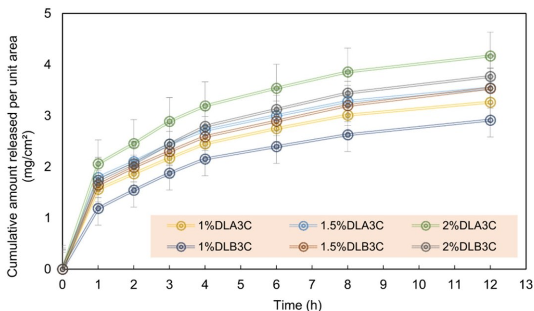
Figure 8. Cumulative amount of DS release per unit area ( \text{mg}/\text{cm}^2 ) for DS -mediated DL A 3C and DL B 3C [54].
