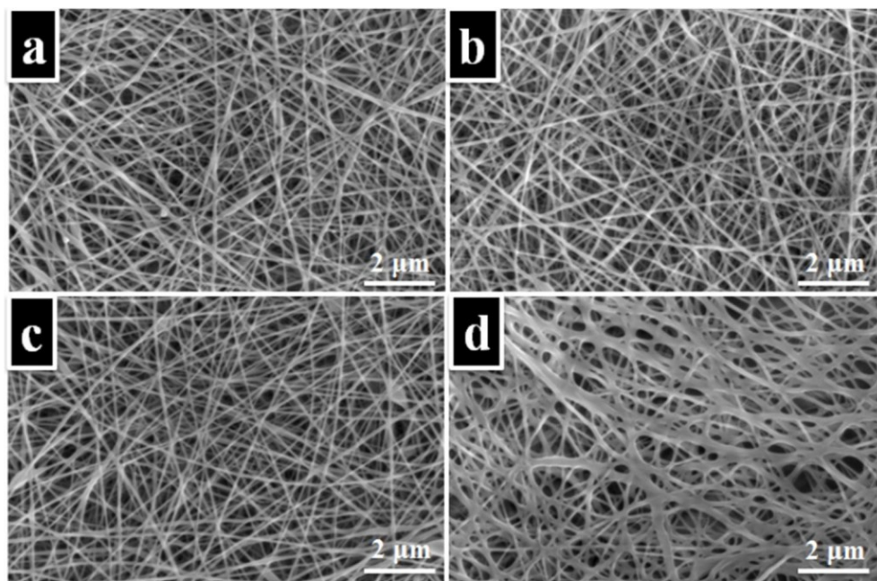
Figure 12. SEM micrographs for the electrospun membranes of (a) PVA, (b) PVA– Thymus vulgaris , (c) PVA– Salvia officinalis folium , and (d) PVA– Hyperici herba [85].
