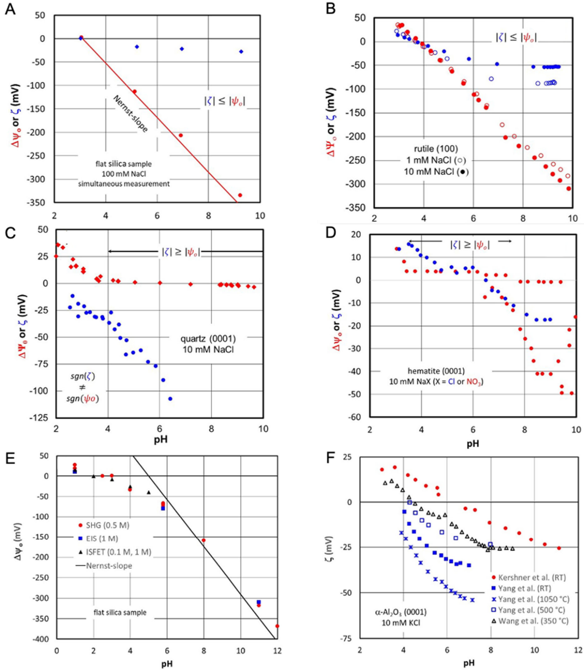
Figure 23. Simultaneous measurements of potentials. A) Surface (ISFET) and zeta (streaming) potentials for flat silica surfaces, 372 the straight line corresponds to the Nernst-slope. B,C) Measured surface potential (single crystal electrode) and zeta potential (streaming current) for rutile (100) and quartz (0001) faces. 377 D) Measured surface potential (single crystal electrode) 379 and zeta potential (streaming current) 382 for hematite (0001) faces. \Psi_0 is the surface potential and \zeta is the zeta potential. E) Comparison of reported surface potentials for flat silica samples as obtained by various methods. SHG, second harmonic generation in 0.5 M NaCl; 383 EIS, electric
