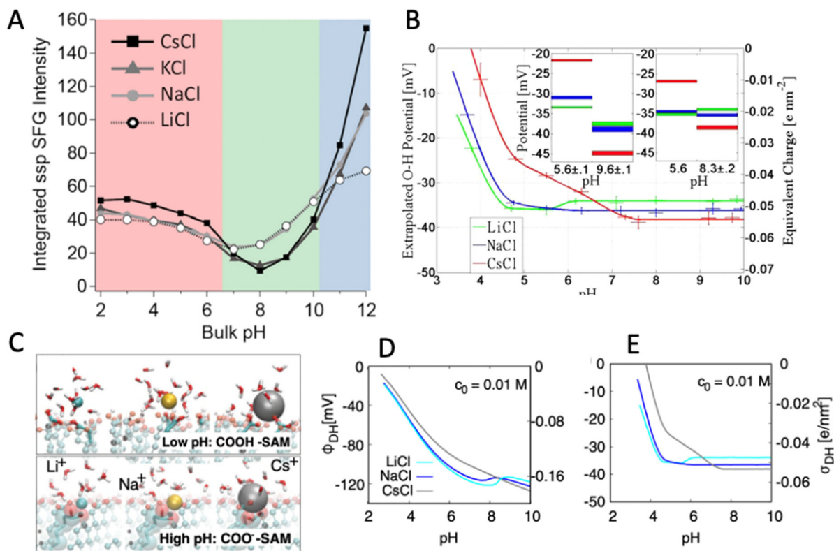
Figure 16. pH-dependence of ion affinity for surfaces. A) Integrated SFG intensities at the silica/aqueous interface as a function of pH with 500 mM alkali chloride solutions. 237 Figure adapted from ref 237. Copyright 2017 American Chemical Society. ACS The integrated intensity is proportional to the amount of ordered water at the interface, which at this high salt concentration should be within a nanometer of the surface. B) Extrapolated outer Helmholtz (O-H) potentials from AFM force measurements between silica surfaces in the presence of 31 mM alkali chlorides. The inset shows replicates on different samples. 235 Figure adapted from ref 235. Copyright 2013 American Chemical Society. C) MD simulation of alkali ions interacting with a carboxylic acid-terminated self-assembled monolayer (SAM) at low pH, corresponding to primarily neutral COOH sites, and high pH, corresponding to more COO - sites. D) Modified PB calculation of the outer Helmholtz potential (left axis) and surface charge density (right axis) as a function of pH for the COOH-terminated SAM. E) Experimental measurements of the outer Helmholtz potential and surface charge density for a silica surface under the same salt concentration as those calculated in part D (0.01 M salt). Both surfaces exhibit this trend reversal with pH suggesting all surfaces dominated by weak acid sites should exhibit such behavior. Figures C-E were reproduced from the literature with permission. 236 Copyright 2016 Elsevier Ltd.
