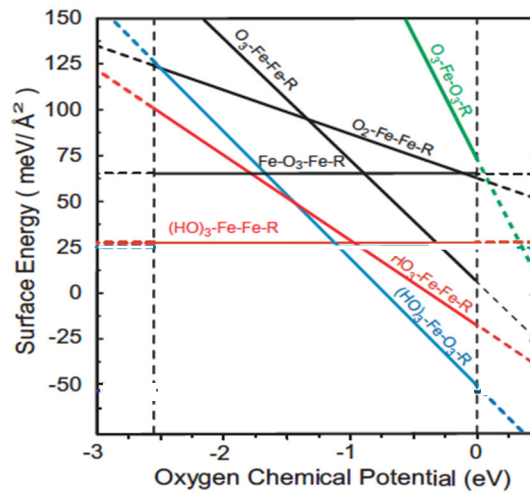
Figure 9. Surface energy vs. O chemical potential for different hematite (0001) terminations. The vertical dashed line on the left is the binding energy of O in the bulk structure, and the vertical
