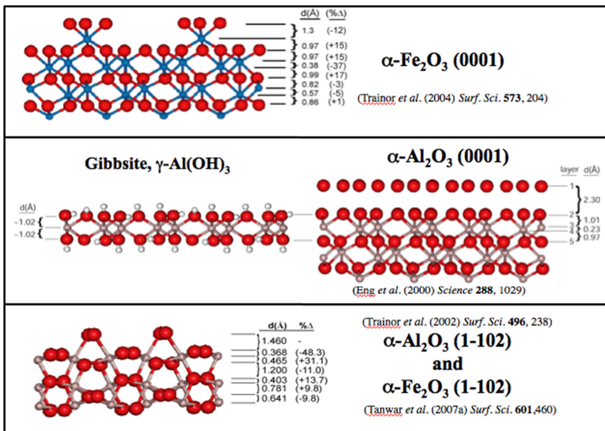
Figure 32. CTR X-ray diffractions studies of the hydrated surfaces of Al- and Fe oxides. (top) Projection of the \alpha\text{-Fe}_2\text{O}_3 structure showing a cross section of the CTR-derived structure of the (0001) hydrated surface; (middle) Projections of the \gamma\text{-Al}(\text{OH})_3 and \alpha\text{-Al}_2\text{O}_3 structures
