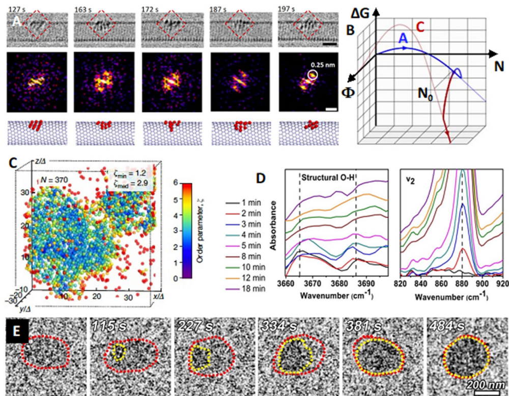
Figure 59. Recent microscopy studies have shed light on multistage nucleation pathways. (A) Figure reprinted with permission after ref 1024. Copyright 2020 Springer Nature. Portion of Au nucleation pathways in a carbon nanotube, showing transition from amorphous to crystalline structure due to (B) crossover in phase stability with size, leading to two nucleation barriers. Figure reprinted with permission after ref 1025. Copyright 2020 Springer Nature Limited. (C) Nucleation of ferritin crystal, showing a gradual increase in order (and coordination) simultaneously throughout the particle. Figure reprinted with permission after ref 1037. Copyright 2020, The Authors, under exclusive licence to Springer Nature Limited. (D, E) 907 Nucleation of calcite, marked by the rise of the \nu_2 IR peak (D) and the spread of high contrast (E) accompanied by loss of structural water (D). Figures after ref 907. Copyright 2020 National Academy of Sciences.
