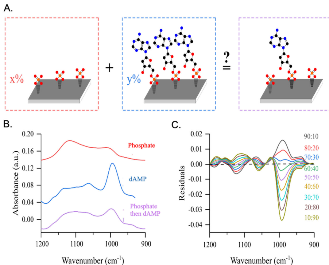
Figure 40. Linear convolution of adsorbed species on \alpha -Fe 2 O 3 . A. Representative cartoon emphasizing the possible percent absorbance intensity of a saturated adsorbed phosphate surface spectrum (red dashed box) added to a percent of saturated adsorbed dAMP surface spectrum (blue dashed box) to yield the spectral absorbance intensity of a multicomponent surface composed of dAMP and phosphate (purple dashed boxed). B. the spectra used for the linear convolution at pH 5. C. the residuals of the experimental spectrum compared to the linear convolution at various percent combinations where the absorbance ratios correspond to % PO 4 : % dAMP. The dotted line represents a perfect overlay of the linear convolution to experimental spectra. Because these cannot be fit using a linear combination, these results suggest synergistic interactions between adsorbed phosphate and dAMP. Figure reproduced from Sit et al. 539 Copyright 2020 American Chemical Society.
