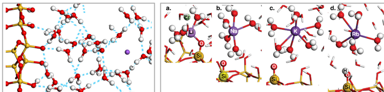
Figure 27. Hydrogen bonding, and impact of ions, at quartz-water interfaces. Left) Quartz (101) surface SiO - with three strong H-bonds to nearby H 2 O. Note that the dipoles of these H 2 O molecules are not aligned perpendicular to the charged surface (Image based on data from DelloStritto et al. 428 ) Right) Geometry optimized Group I cations ions at the quartz (101) surface showing (a.) Li + bonded inner-sphere (IS) to the surface through a SiO - on the surface, (b.) and (c.) Na + and K + outer-sphere (OS) to SiO - on the surface, and (d.) Rb + OS to SiOH on the surface. Right) Images reproduced from Watts et al. 429 Copyright 2022 American Chemical Society.
