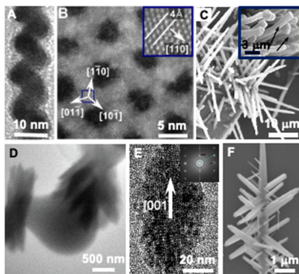
Figure 58. Hierarchical crystallization pathways lead to novel architectures. (A, B) CdSe nanowire (A) 1021 and sheet (B) 1022 formed by particle assembly. Image A is reproduced from ref 1021. Copyright 2005 American Chemical Society. Image B is adapted with permission from ref 1022. Copyright 2014 American Association for the Advancement of Science. (C) Calcite pillars growing epitaxially on calcite rhomb via dense liquid phase (DLP). 1023 (D) Aragonite bundles forming from CaCO 3 DLP droplet. Figure adapted with permission from 1017. Copyright 2014 American Association for the Advancement of Science. (E) Spindle-shaped mesocrystal formed by interface-drive nucleation and subsequent particle attachment. Figure adapted with permission from 919. Copyright 2021, The Authors, under exclusive licence to Springer Nature Limited. (F) Branched rutile nanowire where branches start by attachment and transformation of anatase nanoparticles. Figure adapted from ref 877. Copyright 2013 American Chemical Society.
