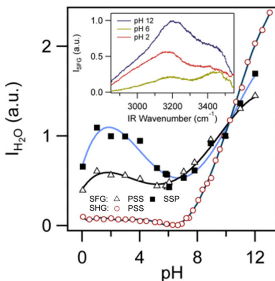
Figure 25. A comparison of non-resonant SHG and vibrational SFG intensities at the silica-water interface at various pH in the presence of 100 mM NaCl. These experiments were performed on the same type of silica sample from the same supplier using the same experimental conditions. These results highlight that non-resonant SHG and SFG report on different features of
