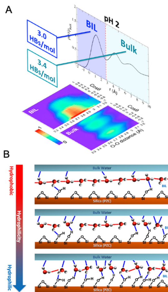
Figure 12. H-bond Structure of Water at Solid Surfaces. A) Water density profile ( r ) with respect to the distance from the neutral silica surface (at the PZC of silica, \sim pH 2) determined from molecular simulations. The bonded interfacial layer (BIL), the average water coordination per molecule (HBs/mol), and the angle with respect to surface normal ( \theta ) are shown. Red-purple scale represents the probability of finding water with the corresponding angle and O-O distance. Figure adapted from ref 11. Copyright 2020 American Chemical Society. B) Scheme illustrating the general organization of water in the BIL of aqueous silica at the PZC with the horizontal order (H-order) shown with the red connectors and the vertical order (V-order) shown with the blue connectors. The scheme illustrates a BIL going from predominant H-order (hydrophobic, top) to predominant V-order (hydrophilic, bottom), via an intermediate balance between H- and V-orders (middle). The schemes also illustrate how the surface chemistry (silanols and siloxanes) influences the balance between H-/V-orders, and vice versa.
