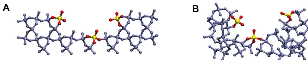
Figure 52. (A) Quartz and (B) amorphous silica surfaces present Q^2 and Q^3 tetrahedra with two and three coordinations to the surface, respectively (figures after Dove et al. 981 ). Copyright 2008 National Academy of Sciences. The physical model holds that amorphous surfaces are repeatedly atomically roughened at a length scale that is the average distance over which Q^2 groups must be removed to get back to a Q^3 -enriched SiO_2 surface.
