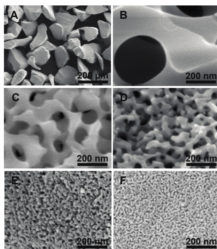
Figure 19. Scanning electron microscopy (SEM) images of experimental substrates: A) amorphous silica controlled pore glass (CPG) particles, and surfaces of porous particles with different average pore sizes B) CPG3000 (328 nm), C) CPG1000, (D) CPG500, (E) CPG120, (F) CPG75. Reproduced with permission from reference Nelson et al. 317 Copyright 2016 Elsevier Ltd.
