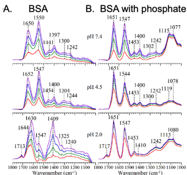
Figure 38. Normalized ATR-FTIR spectra of 1 mg/mL BSA adsorption as a function of time on TiO 2 (22 nm) (a) without phosphate at pH 7.4 (top), pH 4.5 (middle) and pH 2.0 (bottom), (b) with phosphate at pH 7.4 (top), pH 4.5 (middle) and pH 2.0 (bottom). Spectra are shown for four different time points: 10, 30, 60, and 90 minutes (red, green, blue and purple colored spectra, respectively). Figure reproduced from Xu and Grassian. 744 Copyright 2017 American Chemical Society.
