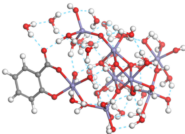
Figure 33. Salicylate bonding to \text{Fe}^{3+} on a model corner site of the goethite (010) surface allows for delocalization of electrons in the aromatic ring and partial reduction of the \text{Fe}^{3+} . Reduction towards the \text{Fe}^{2+} state increases Fe solubility (unpublished results). C = gray, H = white, O = red, Fe = purple, dashed blue line = H-bonds. (Kubicki J.D., unpublished results.)
