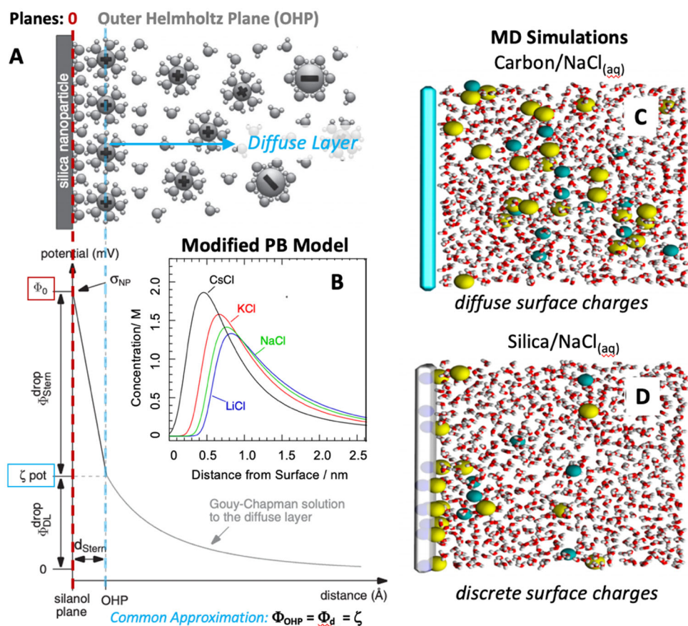
Figure 14. The Electrical Double Layer. A) Schematic of the electrical double layer at a charged silica surface and the corresponding changes in potential as a function of distance from the surface. Modified with permission from reference 223. Copyright 2016 Wiley-VCH. The surface oxygen sites of silica mark the 0-plane, which corresponds to the surface potential \Phi_0 , while the ions are shown at the outer Helmholtz plane (OHP). The potential at the OHP ( \Phi_{OHP} ) is often approximated by the measurable \zeta potential B) Simulations of the ion distribution at a charged silica surface as a function of distance using a modified Poisson-Boltzmann model that incorporates hydration repulsion. 224 Figure adapted from ref 224. Copyright 2015 American Chemical Society. C) Classical MD simulation of aqueous sodium chloride solution at a carbon surface with a diffuse negative surface charge. 225 Figure adapted from ref 225. Copyright 2014 American Chemical Society. D) MD simulation of an aqueous sodium chloride solution at a silica surface with discrete surface charges. 225 Figure adapted from ref 225. Copyright 2014 American Chemical Society.
