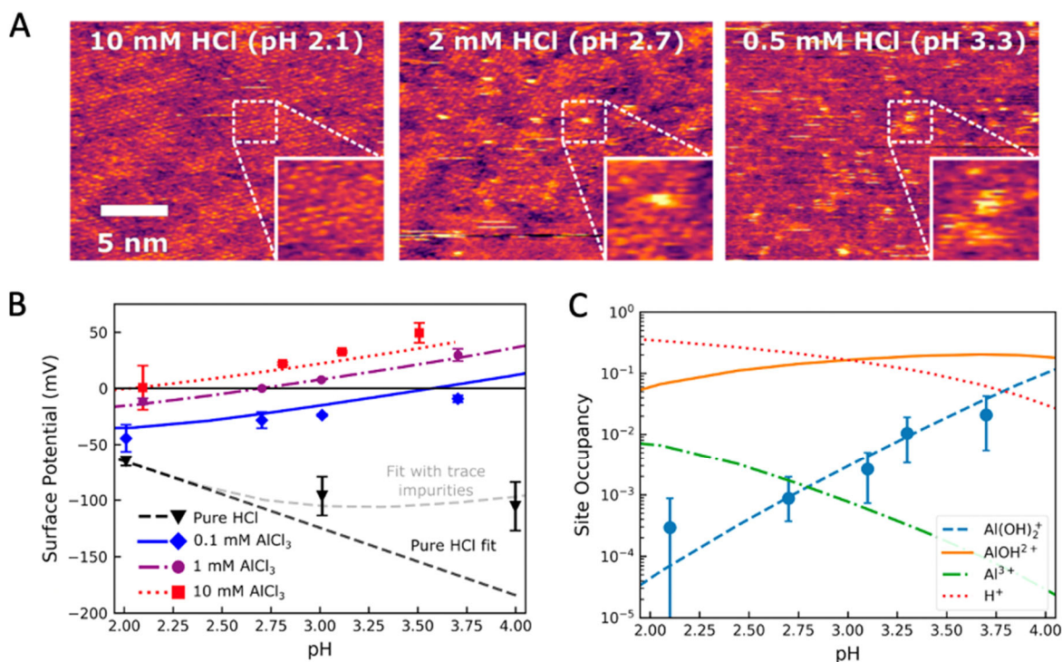
Figure 24. A) High-resolution AFM images of the mica/aqueous interface with increasing pH in the presence of 1 mM AlCl 3 . B) Zeta potentials determined from streaming potential measurements as a function of pH in the presence of various initial concentrations of AlCl 3 . C) Results from a fit of the experimental measurables with a triple layer model. The predicted speciation results were corroborated by AIMD calculations. Reproduced from Legg et al. 391 Copyright 2020 American Chemical Society.
