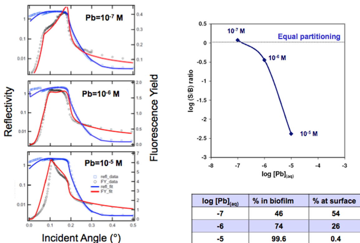
Figure 43. LP-XSW-FY spectroscopy studies of Pb^{2+} partitioning between Shewanella oneidensis MR-1 biofilm coatings and metal-oxide substrates (left) LP-XSW-FY spectra (open circles), fits (red line), and X-ray reflectivity data (open squares) and fits for Pb^{2+} at different lead concentrations on a Shewanella oneidensis MR-1 biofilm-coated \alpha - Fe_2O_3(0001) substrate. (right) Plot of \log Pb^{2+} concentrations in the biofilm coating relative to Pb^{2+} concentrations on \alpha - Fe_2O_3(0001) as a function of \log aqueous Pb and the % Pb^{2+} in the biofilm and on \alpha - Fe_2O_3(0001) at different Pb concentrations. Figure adapted with permission from Wang et al. 265 Copyright 2016 Elsevier Ltd.
