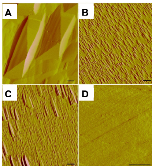
Figure 48. AFM images of (100) quartz surfaces exposed to different solution chemistries for equivalent extents of reaction show the different dissolution processes that are active across driving force and solution chemistry. (Scale bar: 1 \mu\text{m} in all images.) (A) For \sigma = 0.10 in \text{H}_2\text{O} , surfaces are dominated by large etch pits with sloping sides that converge at dislocation sources. Pits are separated by relatively flat regions on the surface. (B) Where \sigma = 0.10 for a solution of 0.0167 M \text{CaCl}_2 , surfaces show a high density of small pits with flat bottoms and with flanks that are 25% steeper than measured for pits in (A). (C) At the intermediate driving force of \sigma = 0.65 in 0.0167 M \text{CaCl}_2 , mixed larger and smaller flat-bottomed pits forms across the surface. (D) For a driving force of \sigma = 0.90 in 0.0167 M \text{CaCl}_2 , surfaces present only straight-edged steps, with no evidence of pitting. Figure after ref 933. Copyright 2005 National Academy of Sciences.
