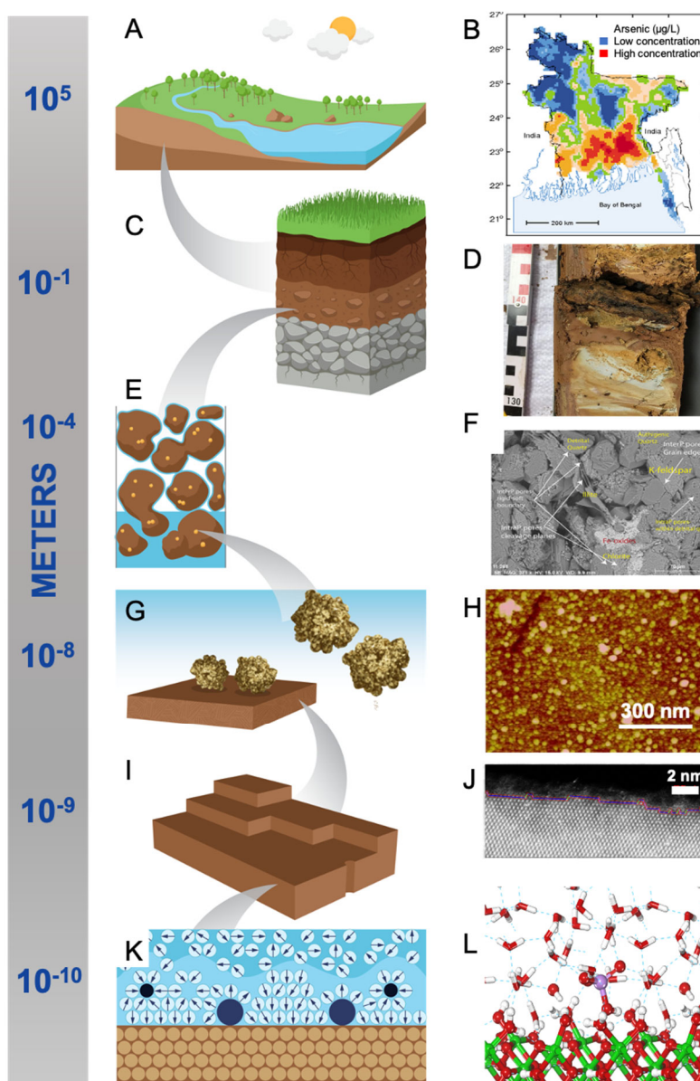
Figure 2. Multi-scale impacts of oxide-water interfacial chemistry. At the global scale, oxide-water interfaces control elemental cycling and therefore impact the availability of clean water,
