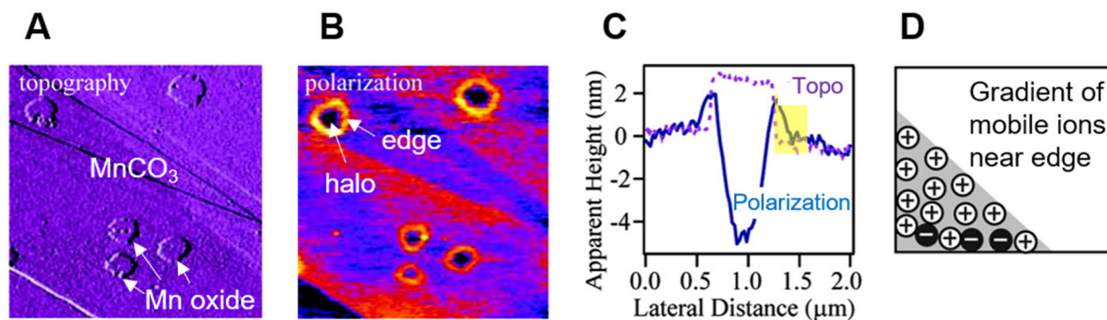
Figure 69. Edge polarization effects are apparent in these dc electric-force microscopy images of Mn oxide on a MnCO 3 surface at 75% relative humidity. Imaging mode: (A) contact, (B) negative dc (note edges), and (C) height profiles of a–b . (D) schematic of mobile ion concentration gradient shown in the yellow box in (C). Reproduced from ref 1292. Copyright 2008 American Chemical Society.
