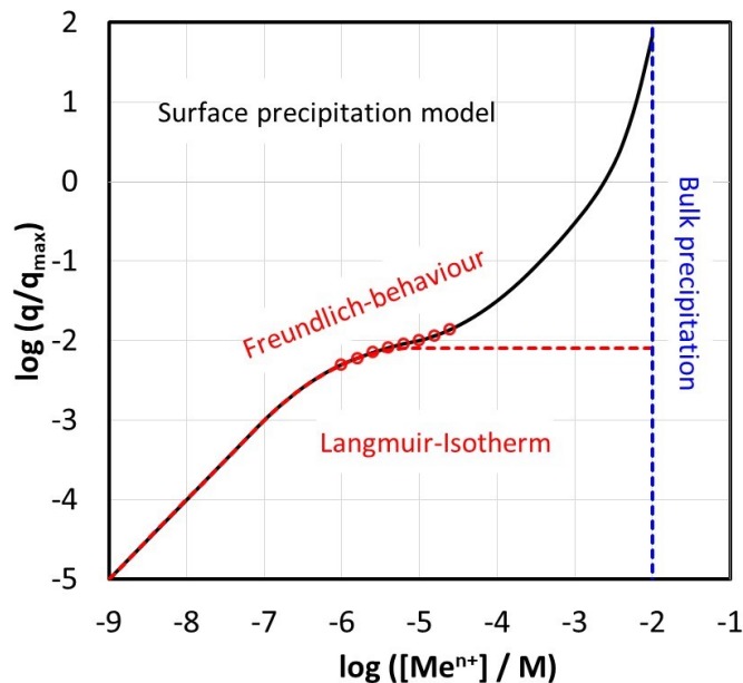
Figure 29. Uptake behavior for a metal ion with charge +n on an oxide surface as a function of metal concentration at constant pH and background electrolyte concentration within the surface precipitation model according to Farley et al. 439 The black full line shows the surface precipitation isotherm. The red-dotted line shows the contribution from a Langmuir isotherm kind behavior. The concentration range with open circles indicates Freundlich-type behavior. The vertical, blue-dotted line shows the limit of bulk precipitation. The symbol q is the adsorbed amount of Me (a cation of charge n^+ ), q_{max} represents the amount of surface sites. Image reproduced from ref 439. Copyright 1985 Elsevier Inc.
