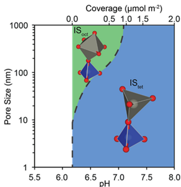
Figure 20. Predominance diagram of \text{Zn}^{2+} surface complexes with respect to pH and pore size. Positions of lines, curves, and shaded regions are specific to the chemical conditions of experiments and would shift as a function of aqueous \text{Zn}^{2+} concentration and amount of available substrate surface area. Green regions and \text{IS}_{\text{oct}} refer to inner-sphere monodentate \text{Zn}^{2+} complexes in octahedral coordination with surface oxygen atoms on am- \text{SiO}_2 . Blue regions and \text{IS}_{\text{tet}} refer to inner-sphere monodentate \text{Zn}^{2+} complexes in tetrahedral coordination with surface oxygen atoms on am- \text{SiO}_2 . Superimposed structures depict possible molecular-level geometries (from Nelson et al. 317 ).
