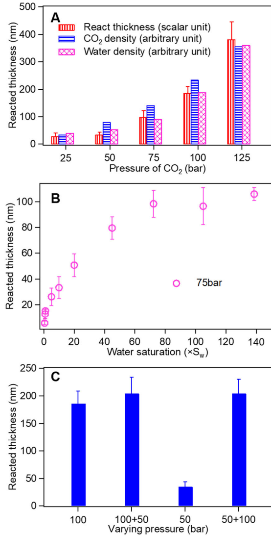
Figure 68. (A) Reacted thicknesses of wollastonite particles with a volumetric mean size of 3.8 \mu\text{m} , after 40 hours at 140\times S_w , 60 °C, and different pressures of CO 2 . The density scales for CO 2 and water at different pressures are not shown. The reacted thicknesses show the same trend as the densities of CO 2 and water. (B) Reacted thicknesses of wollastonite particles with a volumetric mean size of 3.8 \mu\text{m} after 40 hours at different water saturation percentages, 60 °C, and 75 bar CO 2 . The reacted thicknesses reached a plateau beyond 75\times S_w . (C) The reacted thicknesses of wollastonite particles with a volumetric mean size of 3.8 \mu\text{m} after 40 hours at varying pressures, 60 °C, and 140\times S_w . The reacted thicknesses are similar for the control sample reacted only at 100 bar and the sample reacted at 50 bar after an initial reaction at 100 bar. The sample reacted at 100 bar after initial reaction at 50 bar had a larger reacted thickness than the sample reacted only at 50 bar and was similar to the sample reacted only at 100 bar. Figures reproduced with permission from Min and Jun. 1268 Copyright 2018 Elsevier B.V.
