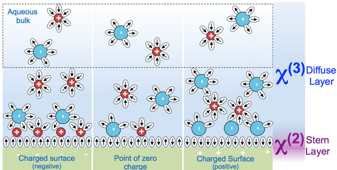
Figure 22. Simplified textbook cartoon of a surface transitioning through the point of zero charge. Dipoles of strongly coordinated water molecules are shown along with ions and charges. (N.B. Dipole are illustrated using the definition prevalent in chemistry, where dipole moments are seen to result from the difference in electronegativity between two chemically bonded atoms, and point toward the most electronegative atom the chemist's vision of electron flow. The physics definition would have the dipole point in the opposite directions, from the negative to the positive). The ion concentration is constant at 1 cation and 1 anion in the bulk slab. \chi^{(2)} and \chi^{(3)} are the nonlinear susceptibilities that contribute to both SHG and SFG measurements and form a basis for understanding structure and electrostatic in the Stern and the diffuse layers.
