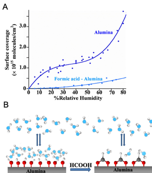
Figure 7. Adsorption of water onto hydroxylated \gamma -Al 2 O 3 particles before and after their exposure to formic acid. (A) Calculated surface coverage by water molecules as a function of relative humidity, measured using quartz microbalance technique. The dramatic decrease in water adsorption is linked to the change in the hydrophobicity of the surface following formic acid adsorption reaction. (B) A molecular-scale interpretation of surface structure and association with water for –OH-terminated vs. –O 2 CH-terminated alumina. Figure reproduced from ref 150. Copyright 2013 American Chemical Society.
