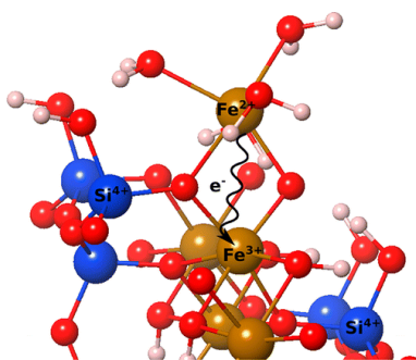
Figure 36. Electron transfer from \text{Fe}^{2+} adsorbed at the edge site to \text{Fe}^{3+} in the structure of an Fe-containing clay mineral. 672 Figure adapted from ref 672. Copyright 2013 American Chemical Society.
