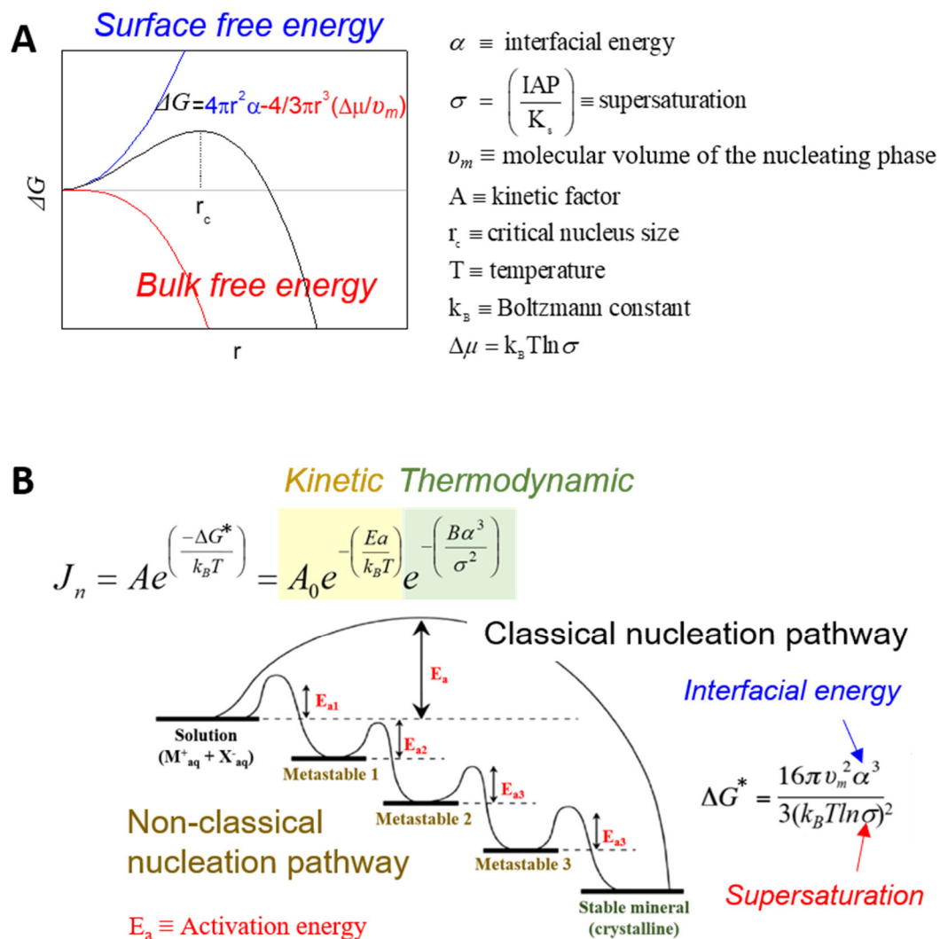
Figure 54. (A) Energy landscape of classical nucleation theory: The bulk and surface terms are related as functions of cluster size, creating a free energy barrier. (B) Energy landscape of non-classical nucleation theory.
