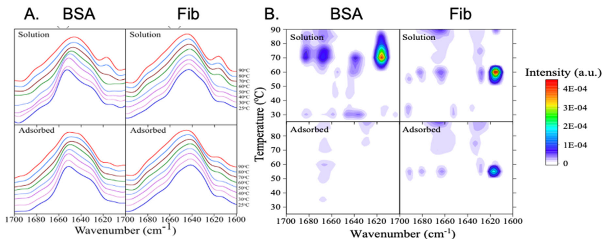
Figure 39. Changes in BSA structure as a function of temperature. A) Normalized ATR-FTIR spectra over a temperature range of 25–90 °C for solution phase BSA and Fib (top) and adsorbed BSA and Fib on TiO 2 (bottom). B) Autocorrelation moving window 2-dimensional correlation map of the amide I band shown in A relating temperature to spectral intensity changes for solution phase BSA and Fib (top) and adsorbed BSA and Fib on TiO 2 (bottom). The color bar intensity (a.u.) value represents the extent of spectral variation due to the external perturbation i.e. temperature. Figures reproduced with permission from Sit et al. 747 Copyright 2019 Elsevier Ltd.
