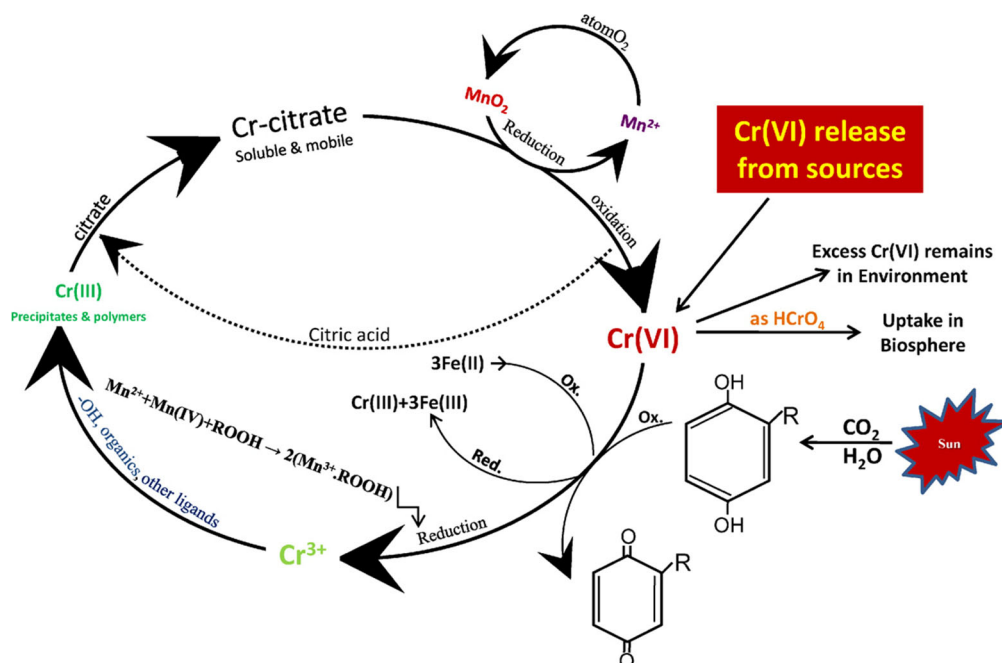
Figure 37. Potential abiotic redox cycles of chromium in the presence of Fe- and Mn-bearing minerals and organic ligands. Figure adapted with permission from Dhal et al. 691 Copyright 2013 Elsevier B.V.
