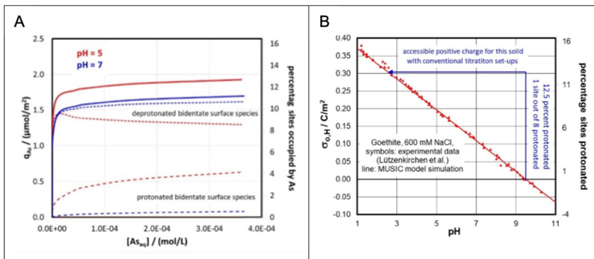
Figure 30. Adsorption of arsenate on goethite. A) Isotherms for arsenate (As) on goethite (0.2 g/L, 100 m 2 /g) at constant pH in 10 mM NaNO 3 solution (inert atmosphere), calculated using parameters from ref 443 at pH 5 (red) and pH 7 (blue). Full lines correspond to the overall uptake (i.e., sum of all surface complexes), dotted lines show the contributions from the relevant surface species (the monodentate species has no contribution for these conditions). The left y-axis shows the percentage of sites that is occupied by As or the surface species. B) Titratable surface charge of goethite as a function of pH for 600 mM NaCl; symbols are experimental data 440 and the full line is a simulation using the MUSIC model. 440
