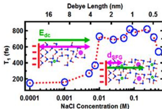
Figure 13. Impact of NaCl concentration on the observed OH stretch vibrational relaxation dynamics at SiO 2 water interfaces. Figure adapted from ref 211. Copyright 2020 American Chemical Society.
