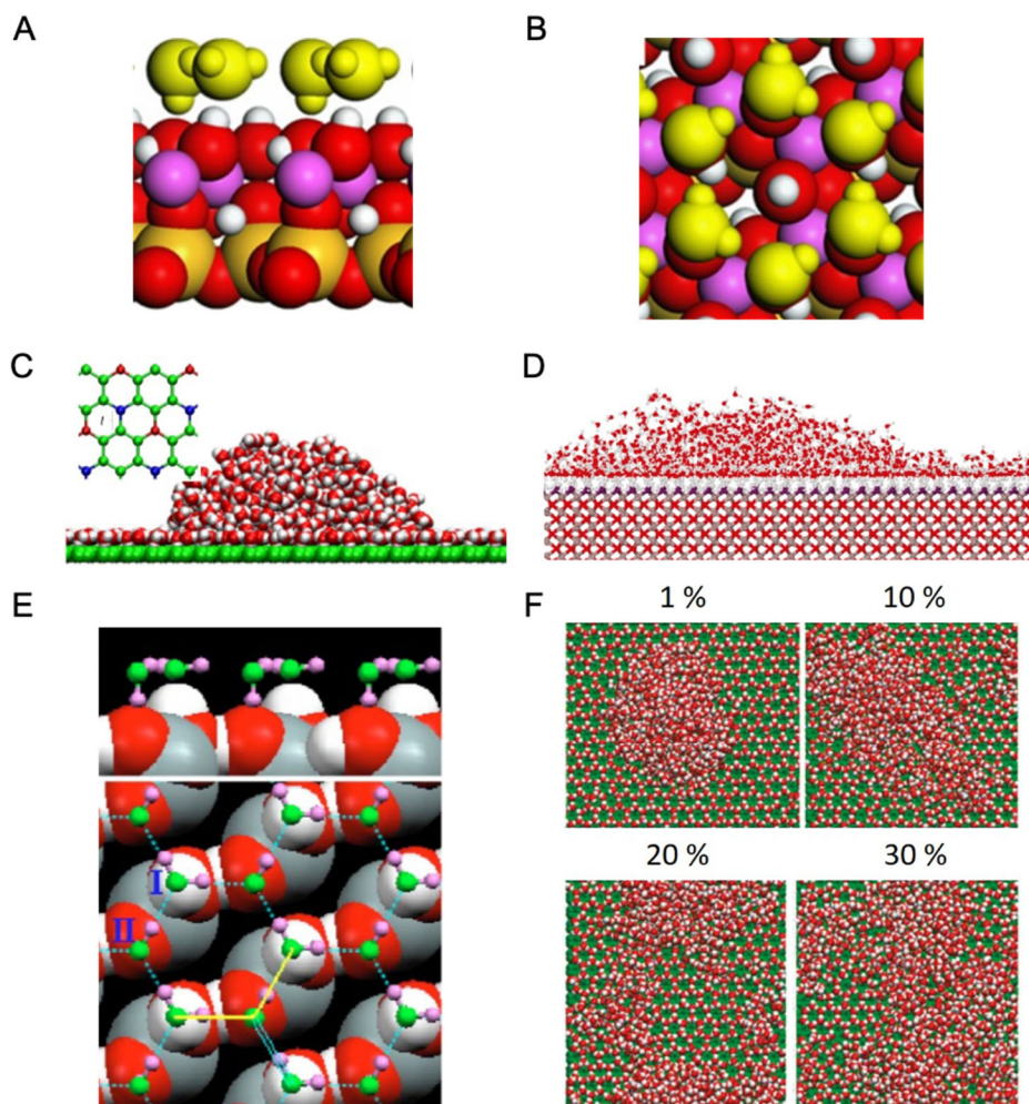
Figure 11. Hydrophobic water layers on hydrophilic surfaces. A) Side and B) and top view of a water film on the gibbsite plane of kaolinite. 171 Figures adapted with permission from ref 171. Copyright 2007 Elsevier. C) Water droplet on a water film that is formed on a generic surface with a hexameric structure. 174 Figure adapted with permission from ref 174. Copyright 2009 American Physical Society. D) Water droplet spreading on a hydroxyl terminated sapphire (0001) plane. Figure adapted from ref 175. Copyright 2011 American Chemical Society. E) The hydrophobic water layer on a quartz (0001) plane. 179 Figure adapted with permission from ref 179. Copyright 2006 American Physical Society. F) The effect of the quantity of defects on the persistence of the hydrophobic water layer. Figure adapted from ref 182. Copyright 2011 American Chemical Society.
