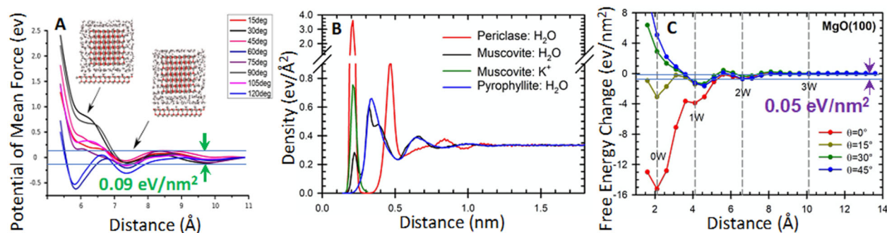
Figure 61. Simulations predict a dependence of interparticle potentials on relative orientation driven by hydration structure, which is strongly impacted by surface hydrophobicity. 1072 (A) Potential of mean force vs distance between ZnO surfaces, showing minima that correspond to integer numbers of water layers and barriers between minima equivalent to \sim 40k_B T for a 10 nm 2 contact area. (B) Effect of hydrophobicity on water density, with periclase (MgO) being most hydrophilic and pyrophyllite most hydrophobic. (C) Free energy vs distance between MgO surfaces for the water structure in (B), showing strong orientation dependence and sizeable barriers. Figures adapted from ref 1072. Copyright 2020 American Chemical Society.
