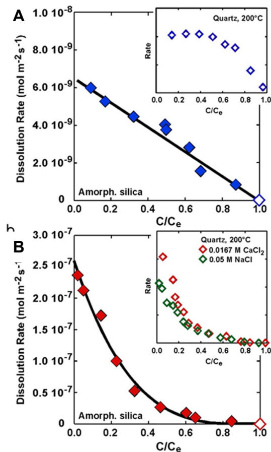
Figure 51. Measured rates of vitreous silica dissolution versus undersaturation, C/C_e , show two different trends , where C and C_e are measured and equilibrium concentrations of H_4SiO_4^0 , respectively.: (A) In the absence of electrolytes, the rates show a linear dependence on chemical driving force, as expected for an amorphous material. (B) Solutions of NaCl or CaCl_2 \cdot 6H_2O at 150°C induce 100X faster dissolution rates at high undersaturations because a pit nucleation-dominated process predominates. The measurements show exponential dependence upon the degree of undersaturation, just as was determined for a crystalline polymorph, quartz, at 200°C. Figure after Dove et al. 981 Copyright 2008 National Academy of Sciences.
