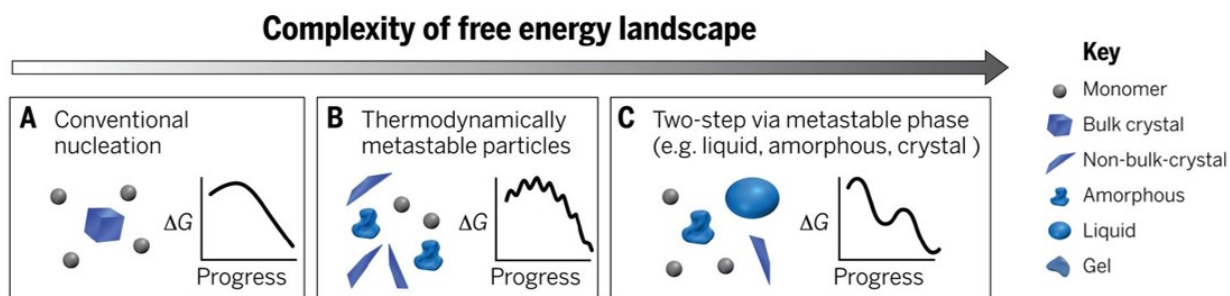
Figure 55. Crystallization by a wide variety of pathways. The possible pathways by which monomers form a stable bulk crystal, and the physical mechanisms that give rise to them, can have thermodynamic origins (A to C). (A) Classical monomer-by-monomer addition. (B) Aggregation of metastable particles, such as liquid, amorphous, or poorly crystalline particles. Although not shown, the free energy landscape graphed in (B) can also result from aggregation by oriented (and nearly oriented) attachment of metastable nanocrystals. (C) Crystallization via the formation of a metastable bulk phase, such as a liquid or solid polymorph. (B) and (C) illustrate the non-classical nucleation pathway. Reproduced with permission from De Yoreo et al. 994 Copyright 2015 American Association for the Advancement of Science.
