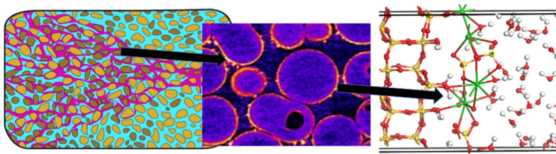
Figure 3. Flow through porous media 34 leads to adsorption of nutrients (e.g., phosphate), and contaminants (e.g., arsenate, pathogenic bacteria), while dissolution enhances and precipitation hinders macroscopic flow. From left to right, the images depict models of flow through porous media, how the porosity and permeability change as a function of precipitation on grains, and a molecular mechanism of surface precipitation. (Left: Reproduced from ref 34. Middle: Courtesy of Anovitz at ORNL. Right: Reproduced from ref 22. Copyright 2014 Watts, Tribe, and Kubicki.)
