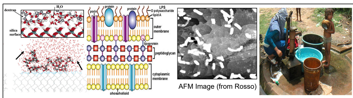
Figure 4. Bacterial-mineral interactions that impede transport of microorganisms in soils and aquifers. EPS extending from the surfaces of bacteria interact with metal oxides (commonly Fe-oxy(hydr)oxides) and filter them out of the flowing solution. This naturally-occurring phenomenon can be mimicked for low-cost water filtration systems. (L to R –Figure adapted from Kwon et al. 45 Copyright 2006 American Chemical Society. AFM image adapted with permission from Rosso et al. 46 Copyright 2003 Elsevier Science Ltd.)
