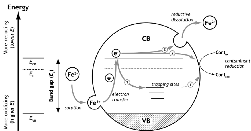
Figure 35. Conceptual schematic representation of the redox-driven conveyor belt mechanism. Reprinted from Gorski & Scherer. 663 Copyright 2011 American Chemical Society.
