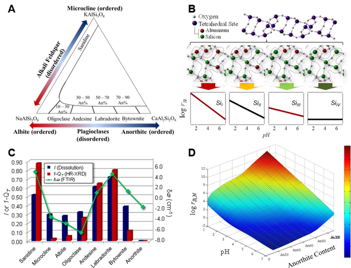
Figure 53 Effect of crystallography on feldspar dissolution. (A) The feldspar group. (B) The “crankshaft chain” structure in feldspar’s framework and illustrations of the pH dependence of the release of different types of Si atoms. Reproduced from ref 987. Copyrights 2014 Elsevier Ltd. (C) Results from feldspar dissolution experiments ( I ), structure refinements based on synchrotron X-ray diffraction ( 1 - Q_T , where Q_T represents the distribution of Al between two different types of tetrahedral sites. Q_T = 0 if completely ordered, and Q_T = 1 if Al is randomly distributed), and data from Fourier transform infrared (FTIR) spectroscopy analyses ( \delta\omega is the displacement of the peak at 650 \text{ cm}^{-1} , which is proportional to the square of the difference in Al/Si ordering). Here, the dissolution incongruence is shown as I , where I = 0 means congruent, and I = 1 if r_{Si}/r_{Al} = 0 . It is obtained from water chemistry experiments and correlates closely with the pattern of the variation in the degree of Al/Si ordering for the feldspar specimens. The Al/Si ordering varies with anorthite contents, as shown in C. Reproduced from ref 986. Copyrights 2014 Elsevier Ltd. (D) pH dependence of plagioclase dissolution at various anorthite contents. Reproduced from ref 987. Copyrights 2014 Elsevier Ltd.
