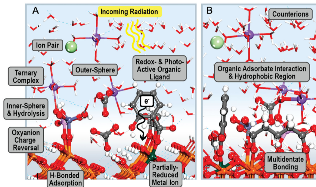
Figure 28. Schematic illustrating the types of sorbates and reactions at the interface. A) The EDL as discussed in Section 2 with various types of adsorbates and sorption mechanisms represented complicating the surface structure and water interactions. Sorbates can compete for sites or form ion pairs and ternary surface complexes. Redox reactions on surfaces such as goethite ( \alpha -FeOOH) shown here often catalyzed by light can be precursors to dissolution reaction discussed in Section 4. B) Adsorption of organic compounds can lead to hydrophobic region on previously hydrophilic surfaces. Longer chain organics can form multiple bonds to a surface and connect multiple particles by binding to more than one surface.
