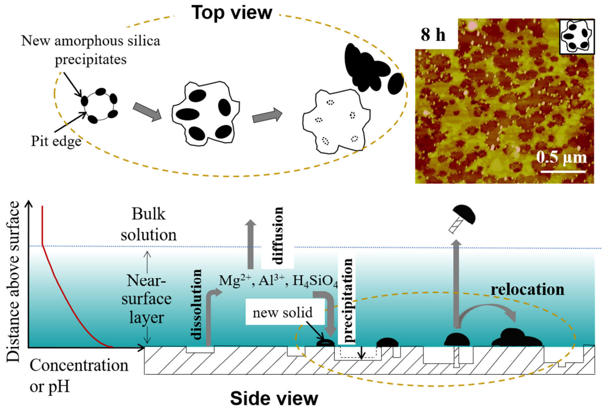
Figure 45. Schematic of proposed reaction pathways for dissolution and precipitation on a phlogopite surface under geologic CO 2 sequestration conditions. The top view, not to scale, shows the evolution of silica particles formed on the edges of a dissolution pit. The inset AFM image shows nanoscale amorphous silica particles formed close to edges of phlogopite dissolution pits after 8 h reaction with 1 M NaCl under 102 atm of CO 2 and at 368 K. Reproduced from ref 824. Copyright 2010 American Chemical Society.
