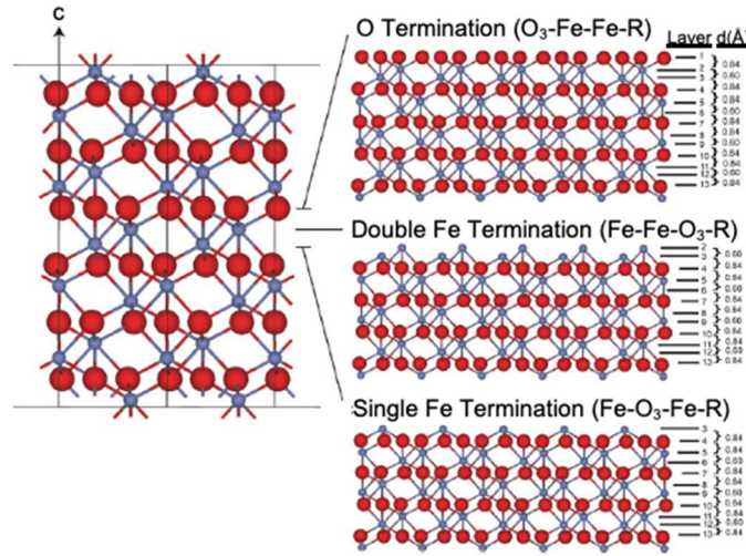
Figure 8. Left panel: Atomic-layer sequence of the bulk unit cell of the \alpha\text{-Fe}_2\text{O}_3 structure along the [0001] direction. Right panel: Surface layer models of the three possible “clean” terminations: ( top ) the O-terminated surface, where \text{O}_3\text{-Fe-Fe} represents the three outermost layers of the (0001) surface; ( middle ) the double iron terminated (0001) surface; and ( bottom ) the single iron terminated (0001) surface. Reproduced with permission from ref 116. Copyright 2004 Elsevier B.V.
