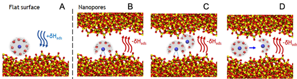
Figure 18. Lanthanide adsorption on surfaces and in pores. Proposed lanthanide (III) adsorption mechanisms which can result in an endothermic ( +\delta H ) or an exothermic ( -\delta H ) signal. A) Lanthanide adsorption as an outer-sphere complex on unconfined SiO 2 surface; B) Lanthanide adsorption as an inner-sphere complex on nanoconfined SiO 2 surface; C) Lanthanide adsorption as an inner-sphere dimer complex on nanoconfined SiO 2 surface; D) Decrease in \Delta G_{\text{hydr}} under nanoconfinement, making dehydration reaction less energetically costly. Modified from reference. 335 Copyright 2021 Royal Society of Chemistry.
