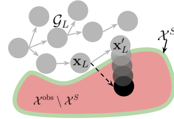
Fig. 3: Generation of contact configurations. When the low-D state \mathbf{x}_L is expanded, the newly generated state is in collision (shown in black with a dashed edge) with X^{\text{obs}} . In this work, we use the inbuilt property of MuJoCo to naturally repel the objects in collision to generate the first configuration \mathbf{x}_L' that exits from X^{\text{obs}} \setminus X^S to X^S as a successor.
