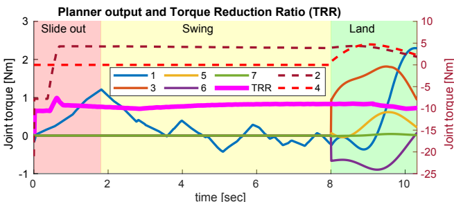
Fig. 8: Joint torque trajectory for simulation scenario (c) and TRR calculated with respect to our baseline (Bi-RRT + direct collocation). The torque plot for joints 2 and 4 using dotted lines use the y-axis on the right.
