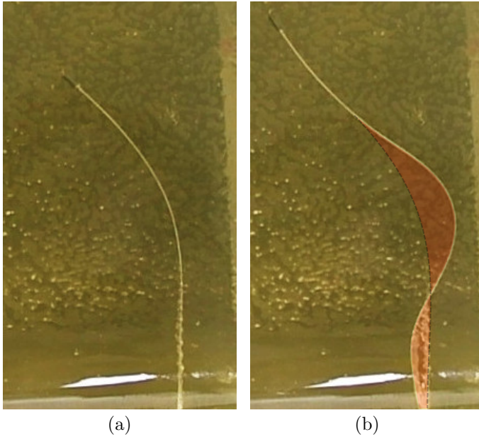
Fig. 2. An example of a needle (a) before and (b) after shearing through a gelatin phantom. Shearing occurs when the force applied by the needle’s shaft to the surrounding tissue is larger than the tissue can support without fracturing, causing the needle shaft to slice laterally through tissue. In (b) we show a dotted line of the shape prior to shearing, and a red region showing the sheared area. This figure demonstrates significant tissue damage due to shearing in a gel-based tissue phantom.
