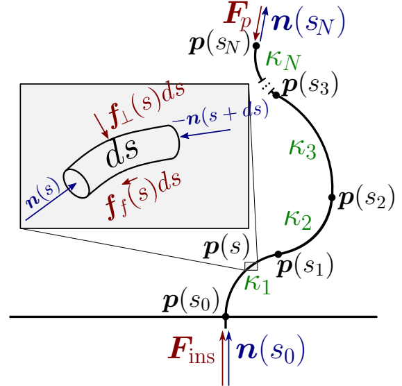
Fig. 3. An example piecewise-circular arc path with parameter endpoints s_i and curvatures \kappa_i . A small segment of length ds is shown with forces. Friction \mathbf{f}_f(s) , tissue normal force \mathbf{f}_\perp(s) , internal needle force \mathbf{n}(s) , insertion force \mathbf{F}_{\text{ins}} , and piercing force \mathbf{F}_p are labeled.
