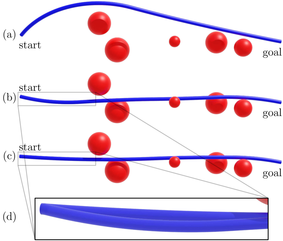
Fig. 10. Generated collision-free trajectories in a randomly generated 3-D environment with spherical obstacles. Utilizing our force model during motion planning produces paths that reduce the normal force on the surrounding tissue when compared with utilizing length as the cost during planning. (a) Initial solution by both planners before optimization, with maximum tissue normal force of 47.0 mN/mm (note, this fit force model predicts shearing begins at 17.6 mN/mm). (b) Solution of the planner using the path-length cost, resulting in a maximum tissue normal force of 20.0 mN/mm. (c) Solution of our planner using our maximum tissue normal force bottleneck cost, resulting in a maximum tissue normal force of 3.5 mN/mm. (d) 3 \times zoomed-in view of both solutions at the start; the path from (b) is below and (c) is above, with much more curvature on path (b). The length difference between (b) and (c) is less than 0.2%, but the force cost from the length planner is 5.7 times larger than the force planner’s force cost, and is beyond the fit force model’s average shearing force.
