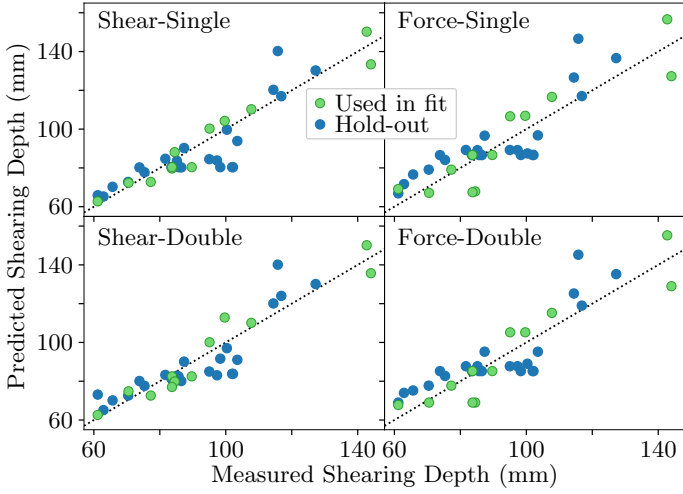
Fig. 8. Qualitative correlation visualization of measured shear depth versus predicted shear depth for various fits. The model parameters are fit from the same set of 12 randomly selected runs, shown in light green, with the remaining 23 runs shown in blue. A perfect model would have all points on the y = x diagonal dotted line.
