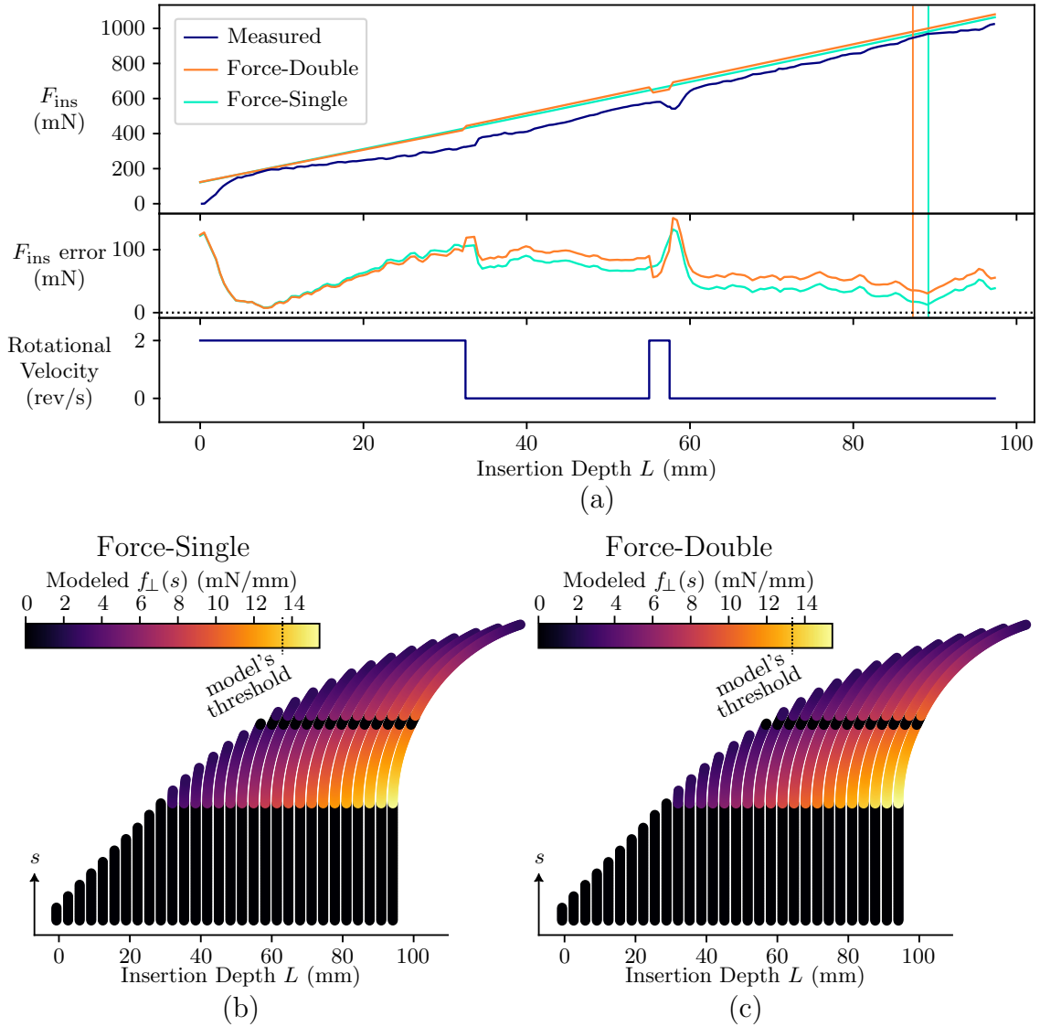
Fig. 7. Modeled and measured F_{\text{ins}} from a hold-out run, and the models' predicted tissue force along the path. This plot is structured the same as Fig. 6, but shows a path not used in the fit. In this example, the predicted insertion forces from this particular fit do not fit the exponential behavior shown in the measured insertion force. Despite this insertion force mismatch, the predicted shearing depth for the Force-Double has nearly identical error percentage compared to Fig. 6 (10%), and for the Force-Single, the error percentage is much better (12% versus 4%).
