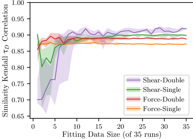
Fig. 9. Fitting data size versus similarity Kendall \tau correlation coefficient. For each fitting data size, d , we performed ten separate fits using d randomly chosen runs from our full dataset of 35 runs, with the remainder kept as a hold-out dataset. The similarity Kendall \tau correlation is computed over all 35 runs. From the ten fits at each fitting data size, we show the median with a solid line between upper and lower quartiles in the shaded regions. A perfect ordering is correlation 1 and a random ordering in expectation is correlation 0.
