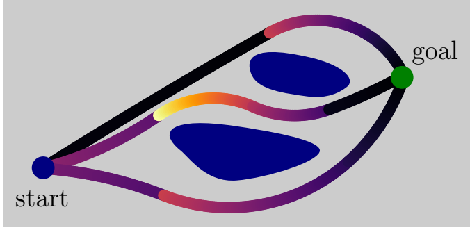
Fig. 1. A tissue normal force profile for three example paths using our new needle-to-tissue force and friction model. Darker colors indicate small values and lighter colors indicate large values. The upper and lower paths have similar lengths and maximum tissue forces. The middle path is 8.5% shorter but has 79% higher maximum normal force despite the middle path’s maximum curvature matching the top path’s maximum curvature. According to our model, the middle path has a higher probability of causing significant damage to the surrounding tissue than the top or bottom paths.
