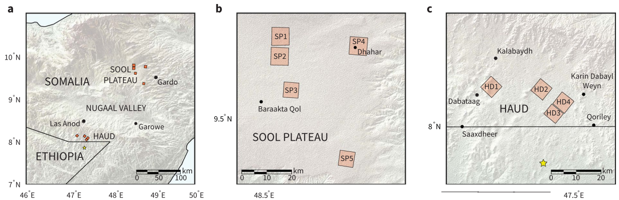
Figure 2. Areas studied in this investigation are defined by nine distinct aerial survey photographs taken in 1952. (a) Study areas are clustered in two regions of Somalia separated by the Nugaal Valley. (b) SP1–SP5 are located in the Sool Plateau pastoral region of Somalia. (c) HD1–HD4 are located in the Haud pastoral region of Somalia. Location of the example images shown in Fig. 1 is indicated with a star. Each photograph covers an approximate area of 50 km 2 . Relief maps rendered using the Shuttle Radar Topography Mission Global 1 arc second elevation dataset 41 in MATLAB 2016b.
